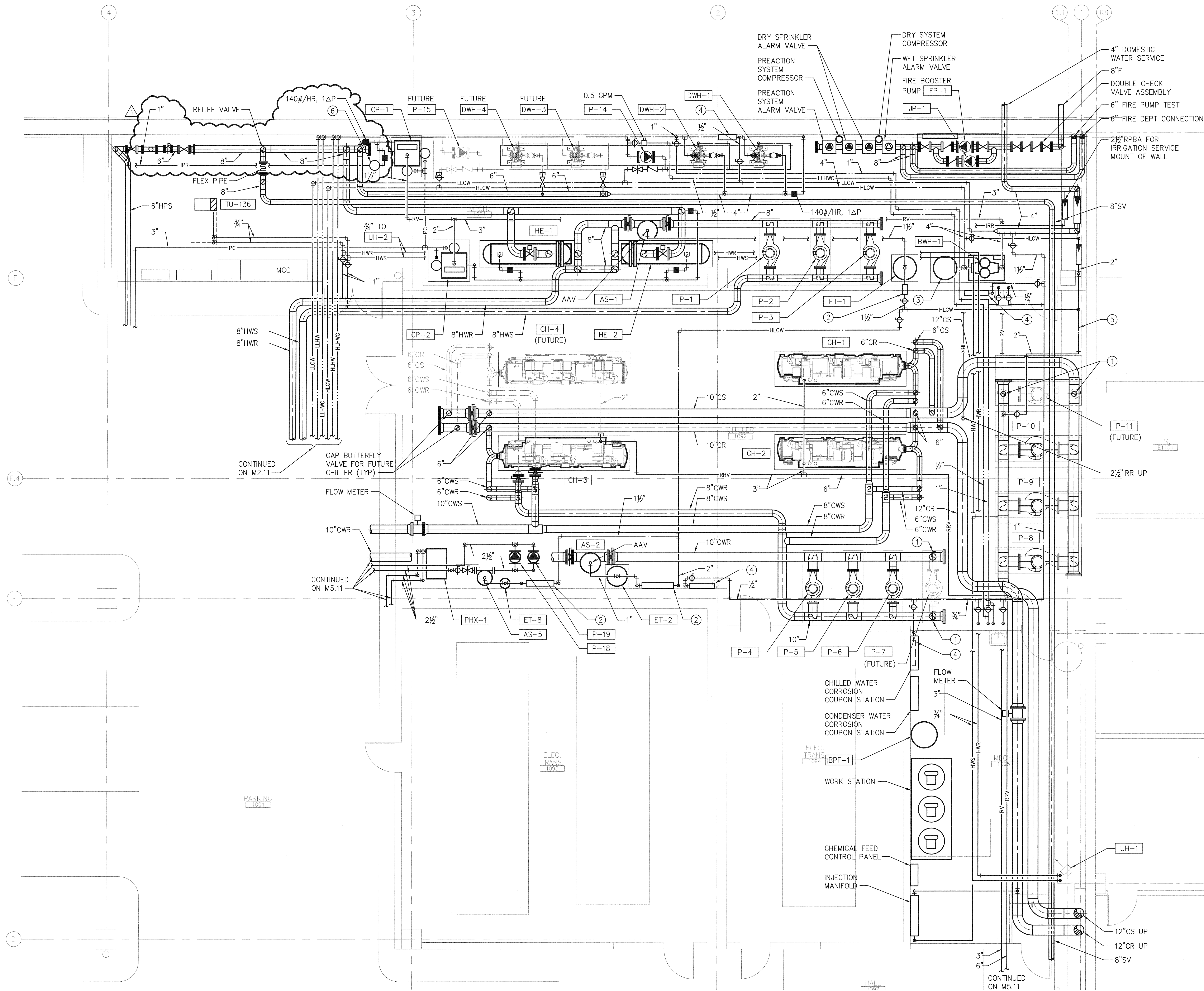
MECHANICAL ROOM PLAN - PLUMBING AND PIPING SCALE: 1/4"=1'-0"
