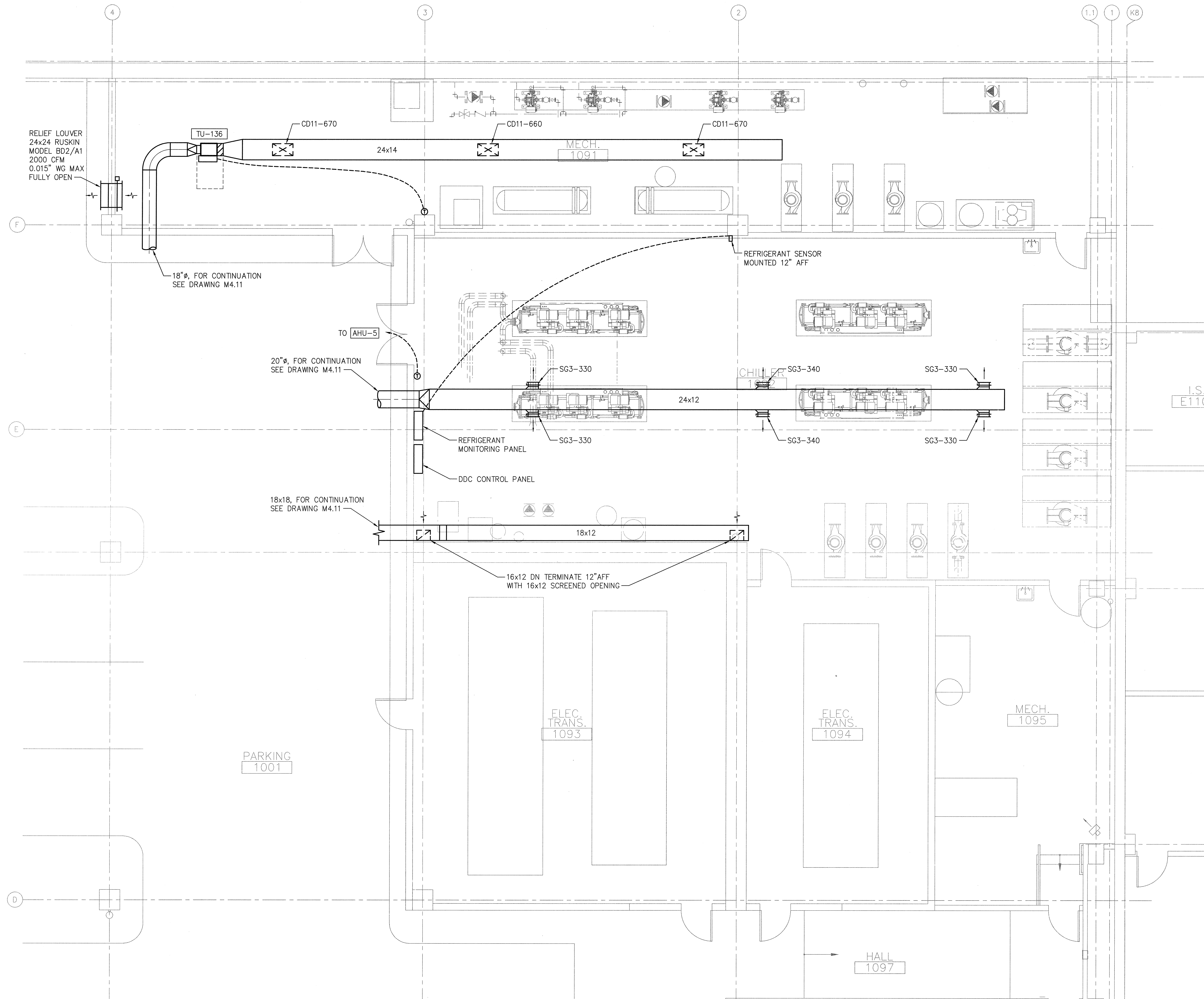
MECHANICAL ROOM PLAN - HVAC SCALE: 1/4"=1'-0"
