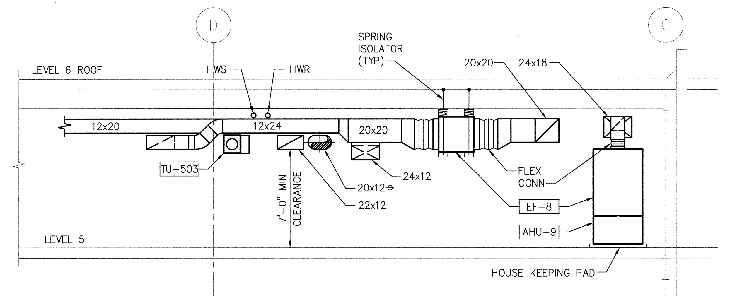
SECTION SCALE: 1/4"=1'-0" (B)
