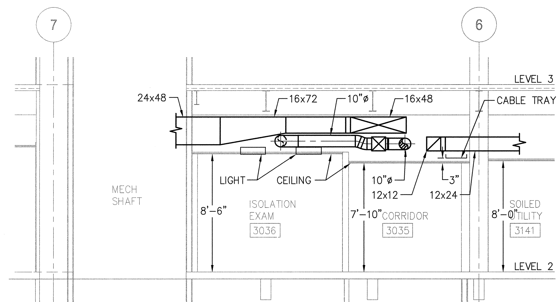
SECTION SCALE: 1/4"=1'-0" (C)
