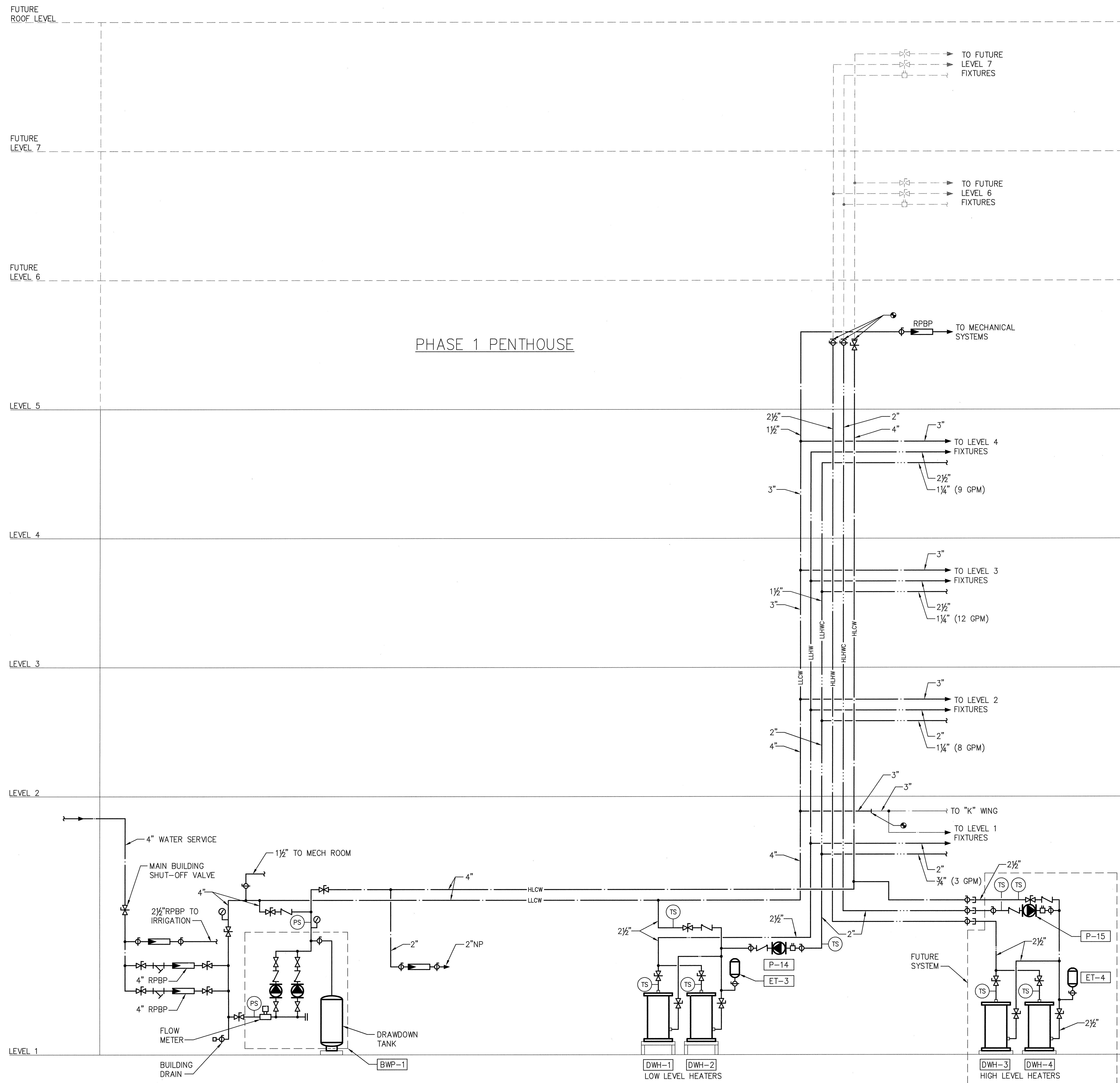
DOMESTIC WATER DIAGRAM SCALE: NONE
