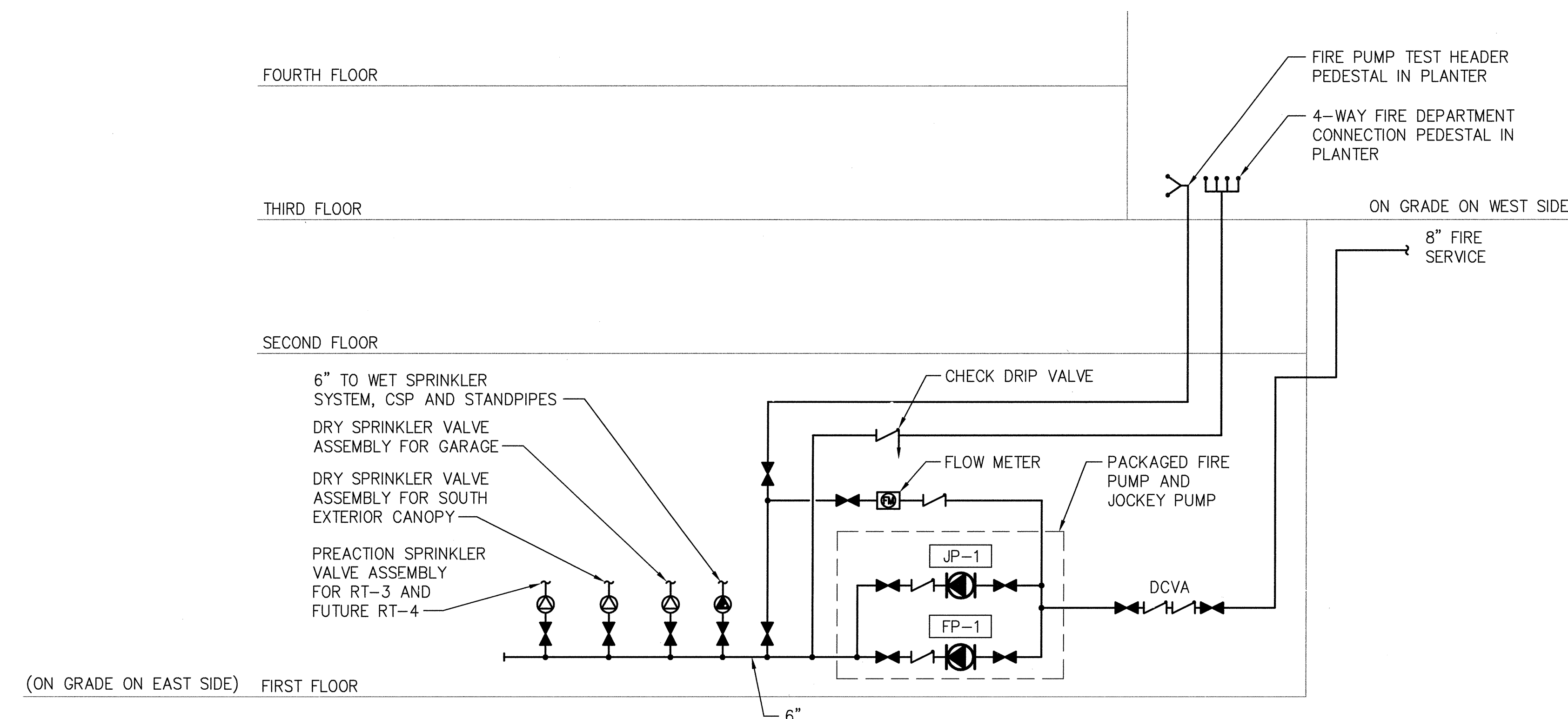
MECHANICAL ROOM FIRE PUMP PIPING DIAGRAM SCALE: NONE
