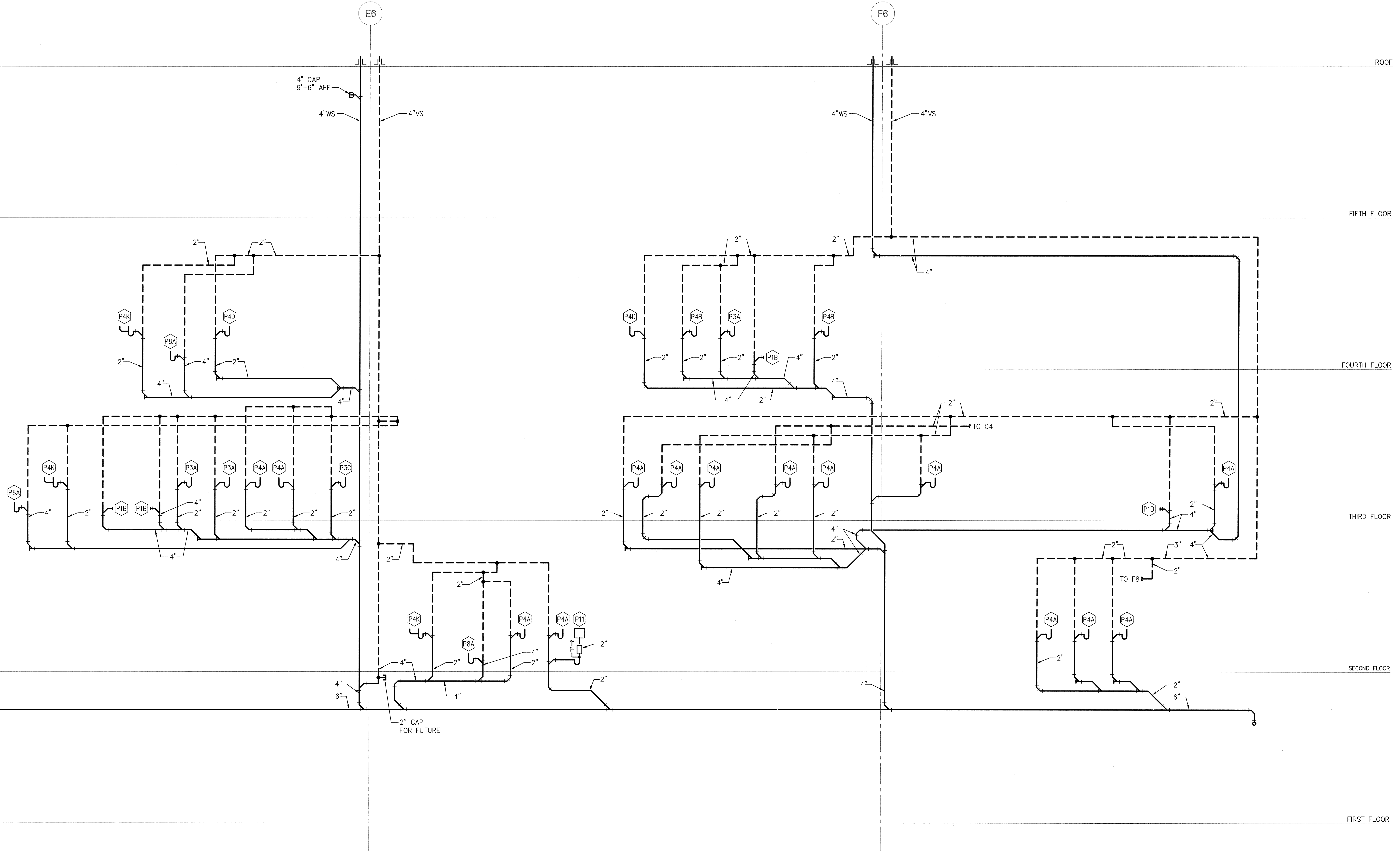
WASTE AND VENT RISER DIAGRAM SCALE: NONE
