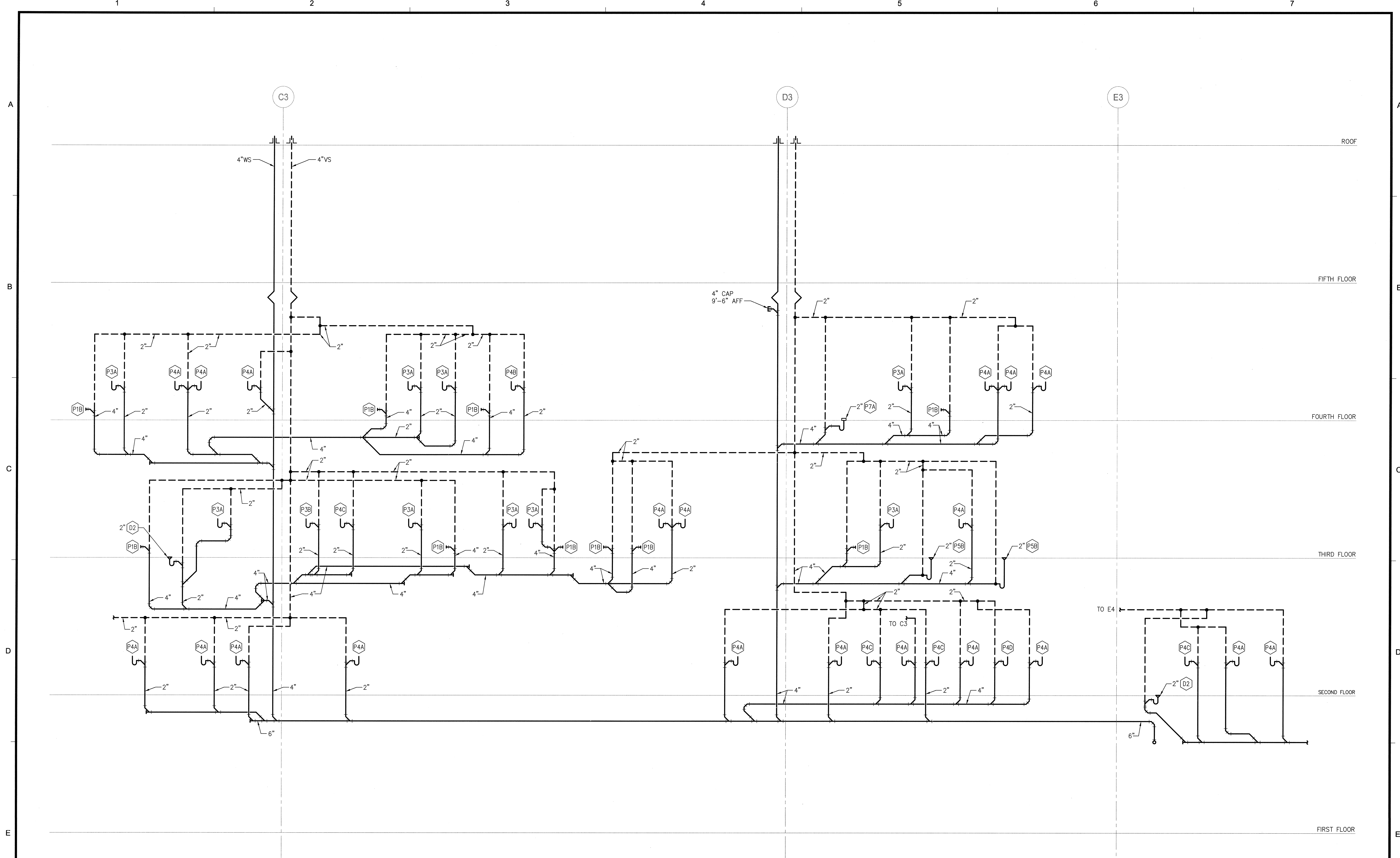
WASTE AND VENT RISER DIAGRAM SCALE: NONE
