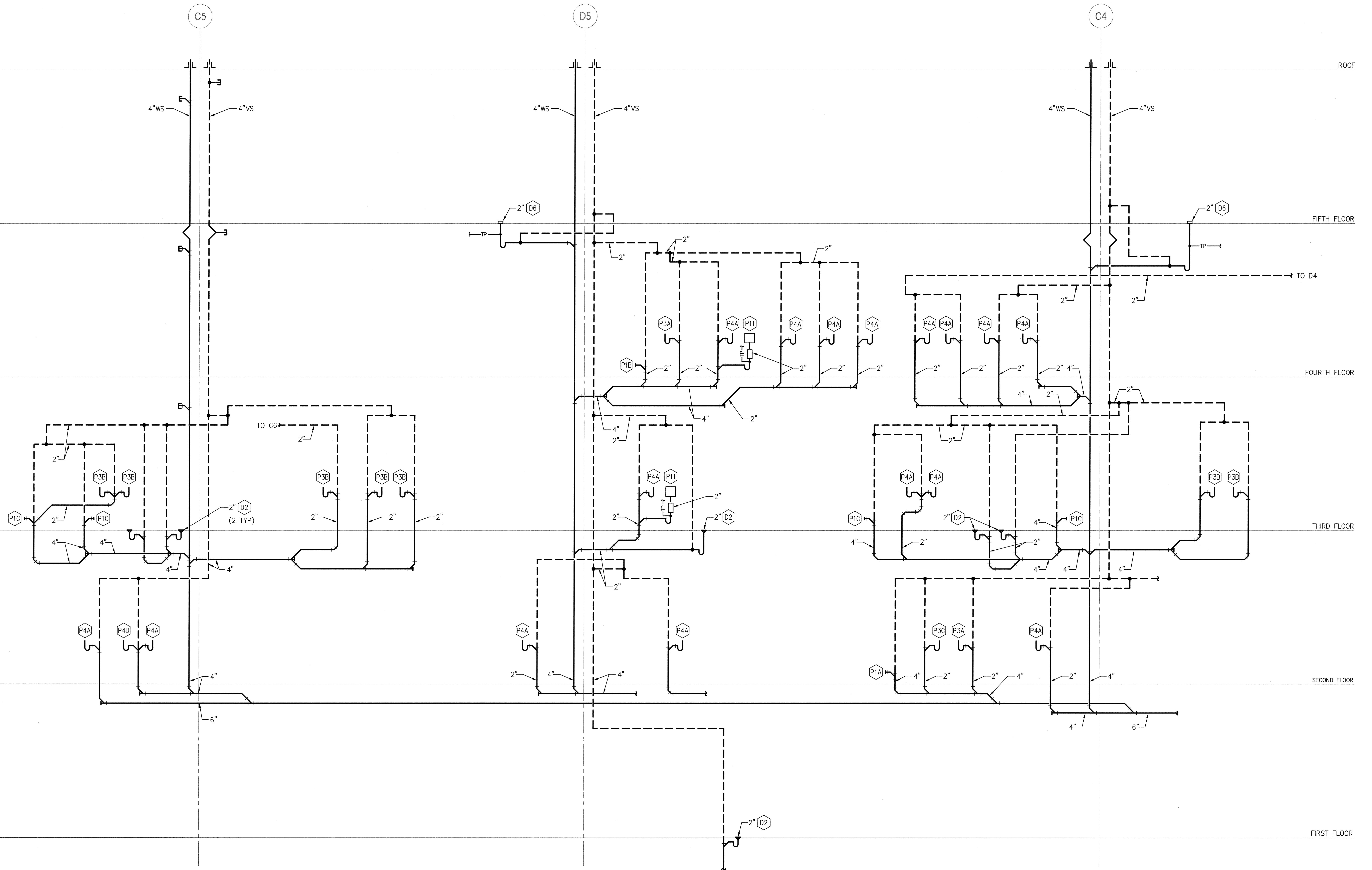
WASTE AND VENT RISER DIAGRAM SCALE: NONE
