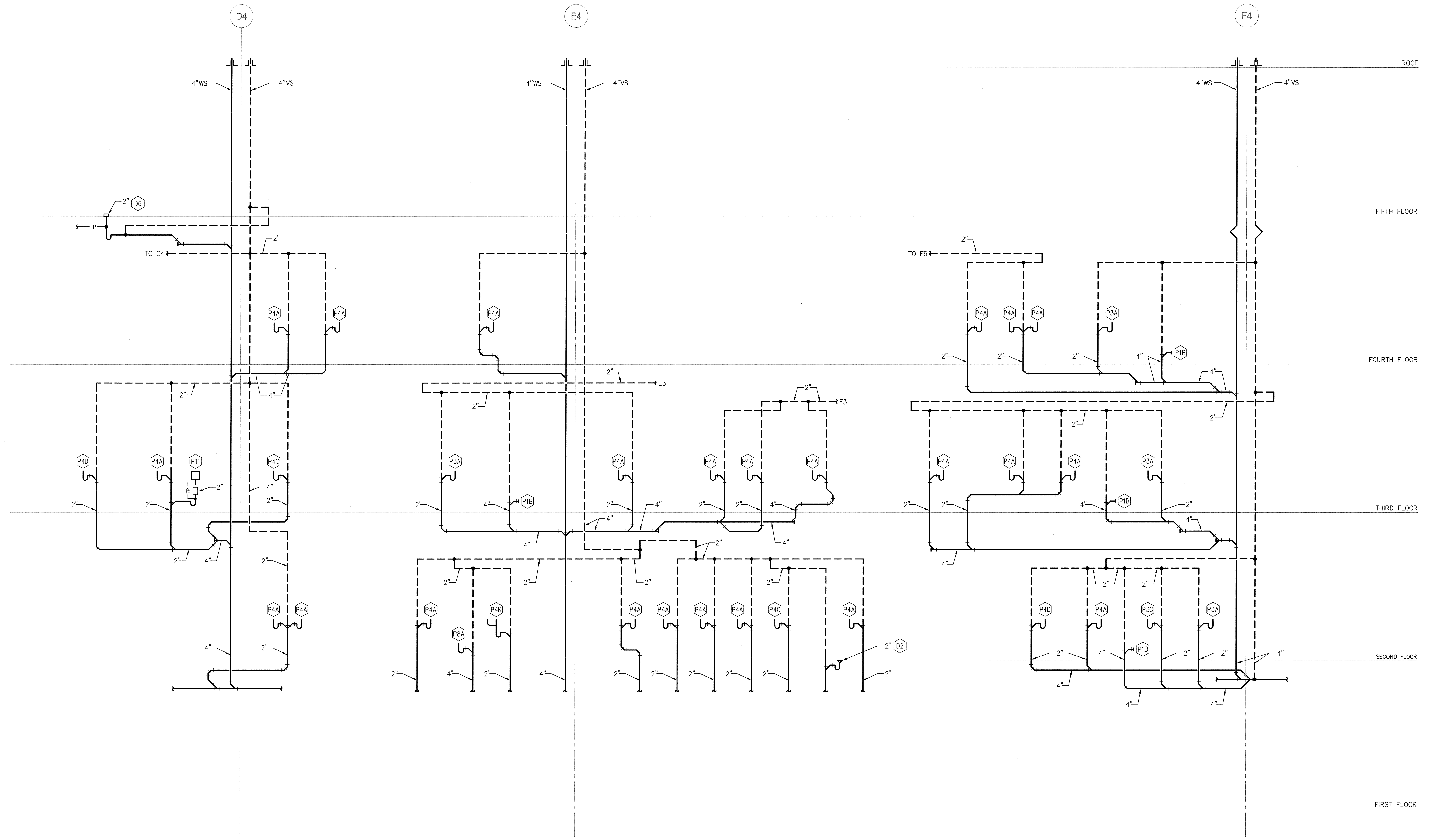
WASTE AND VENT RISER DIAGRAM SCALE: NONE
