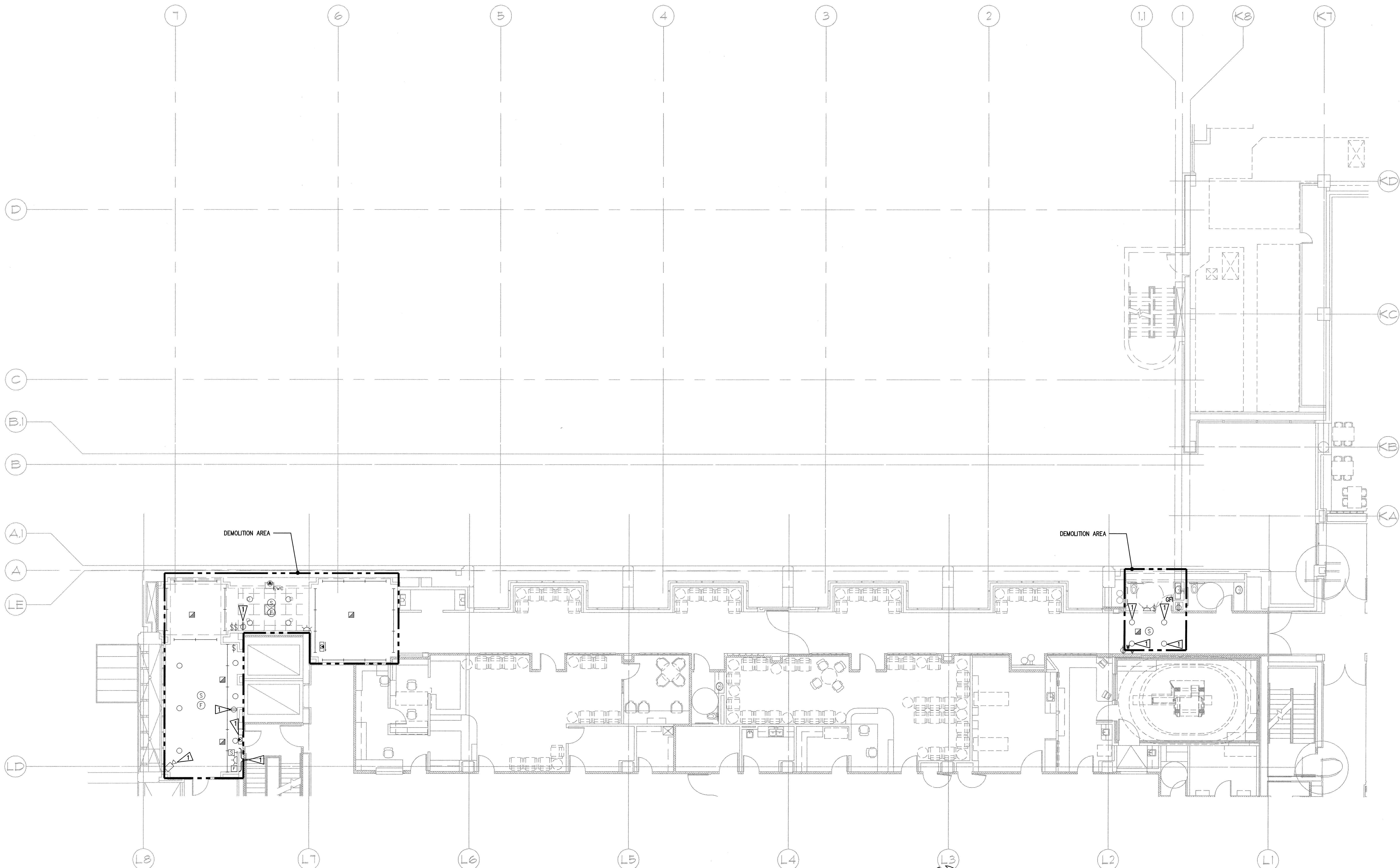
1 THIRD FLOOR PLAN - L-WING & K-WING DEMOLITION - ELECTRICAL E1.33 SCALE: AS INDICATED 0 4 8 16 24 as indicated feet
