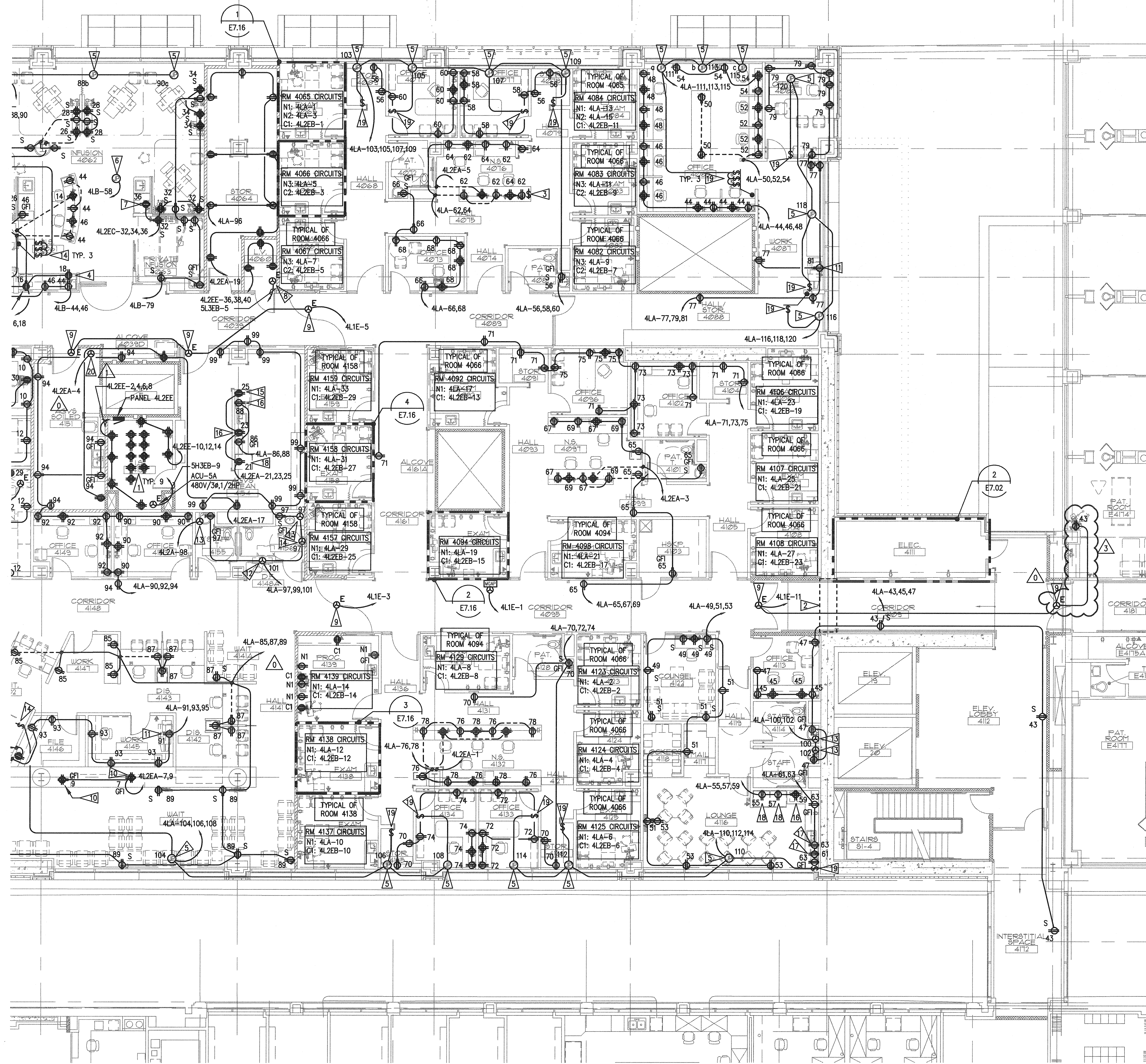
1 FOURTH FLOOR PLAN - NORTH - POWER
