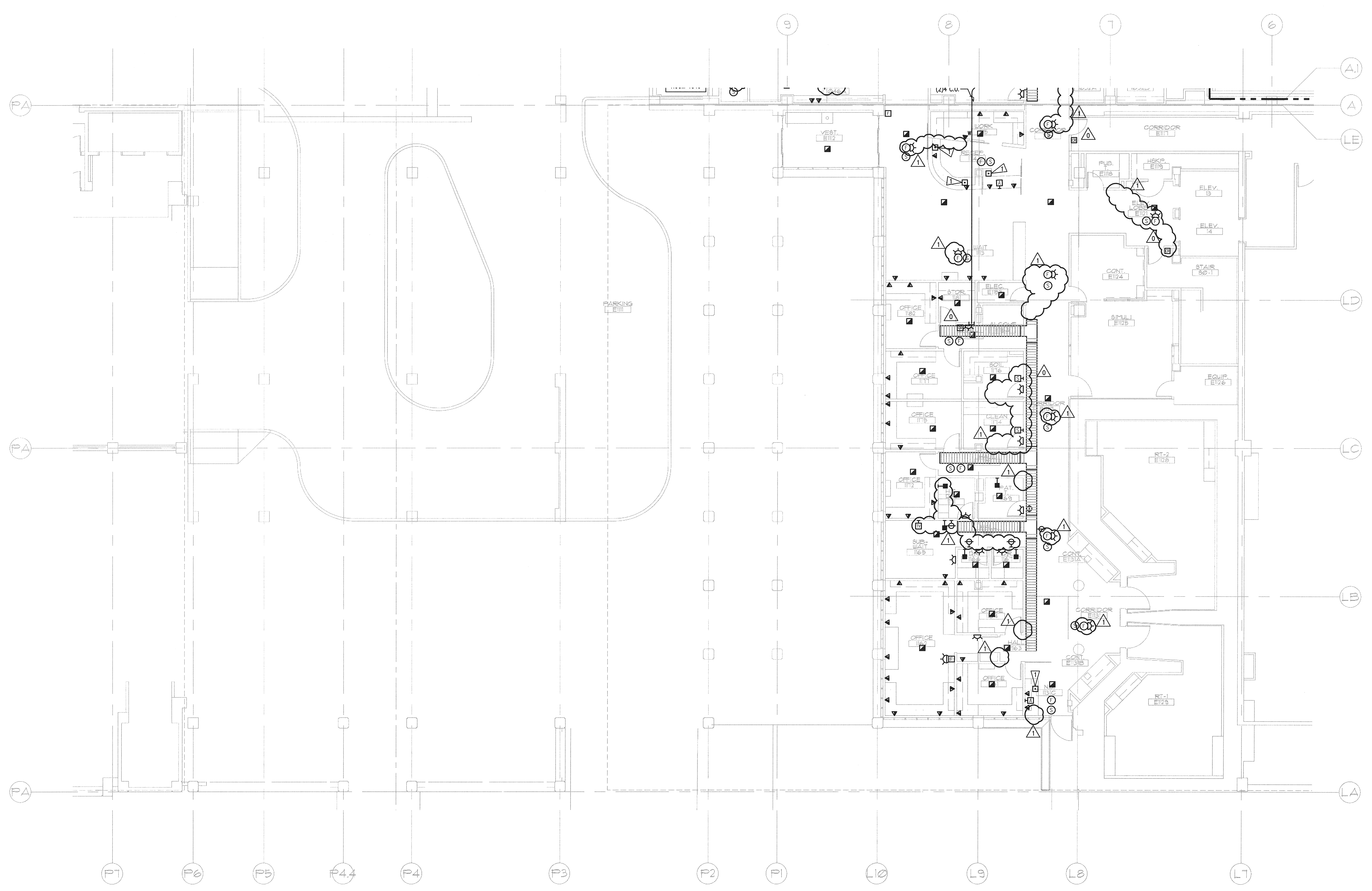
1 FIRST FLOOR PLAN - L-WING - SYSTEMS E4.31 SCALE: AS INDICATED 0 4 8 16 24 as indicated feet
