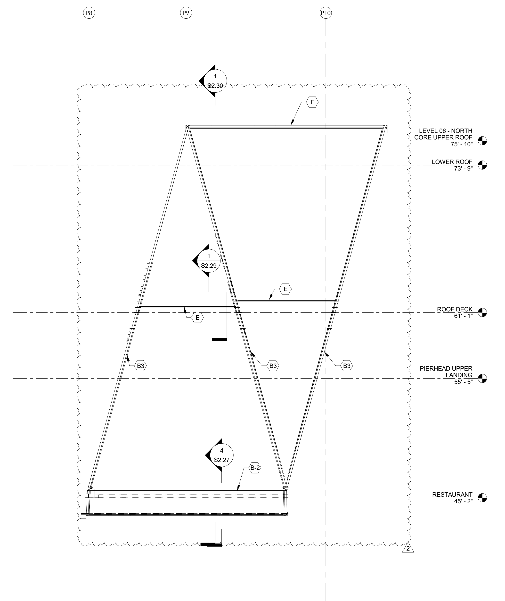
3 SECTION @ VERTICAL ALUMINUM FRAMING 1/4" = 1'-0"
