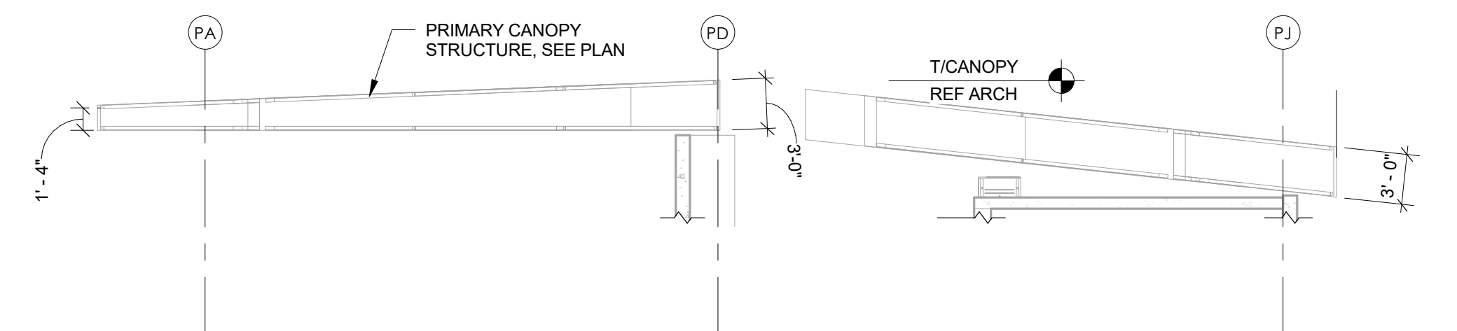
3 SECTION @ VERTICAL ALUMINUM FRAMING 1/4" = 1'-0"
