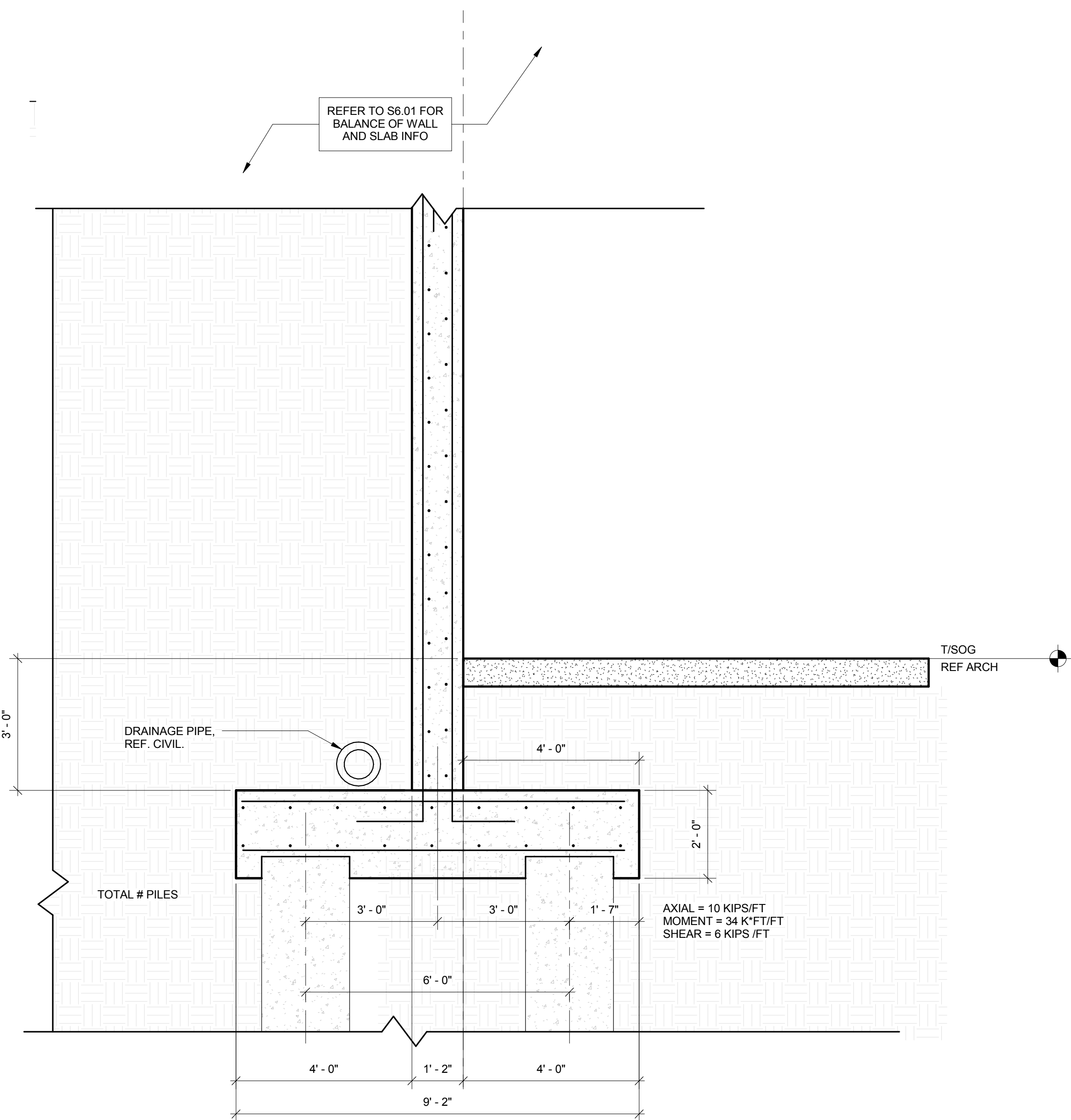
2 TILTED LAWN - TYP SECTION - DEEP PILE ALT. 1/2" = 1'-0"
