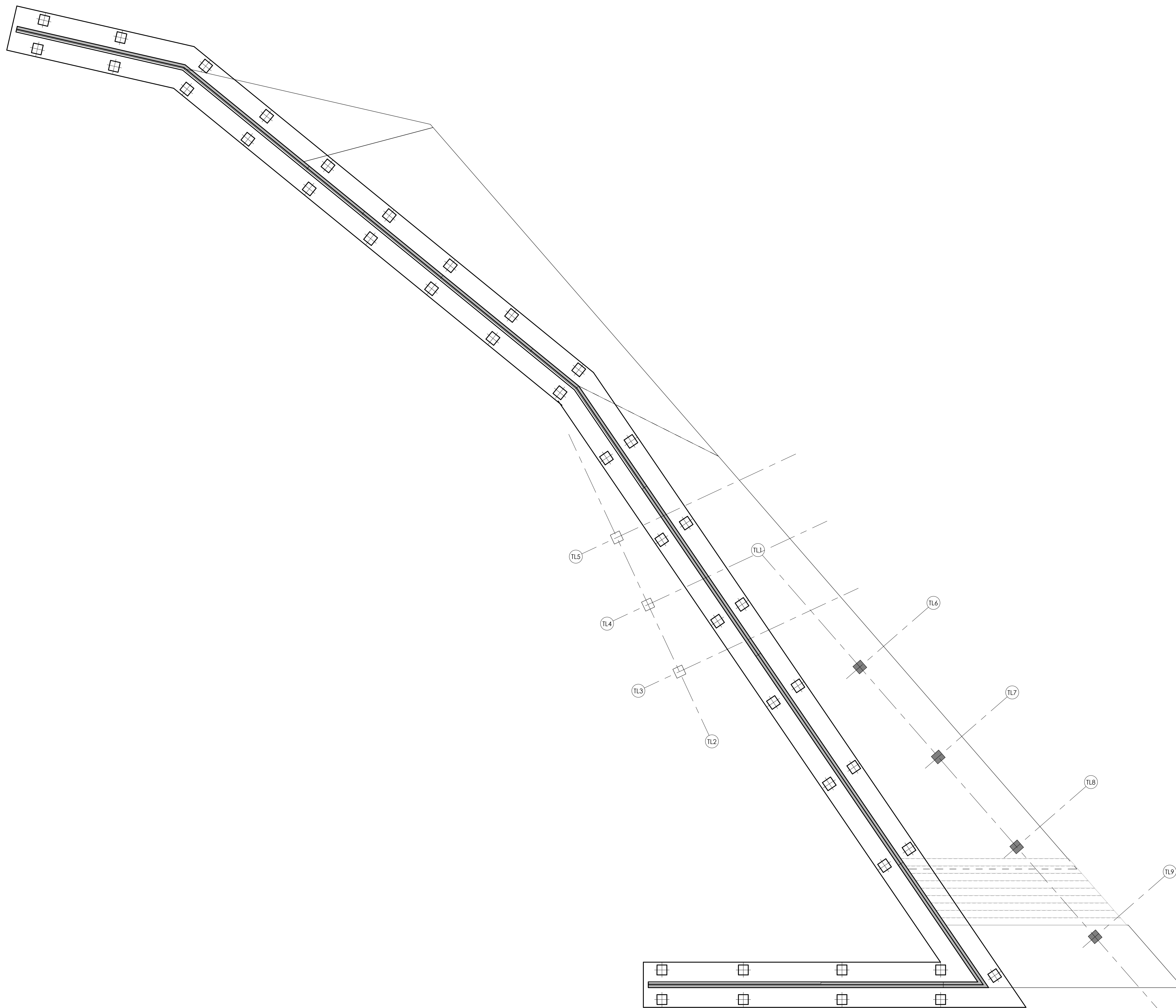
1 TILTED LAWN FOUNDATION DEEP PILE ALT. 3/32" = 1'-0"
