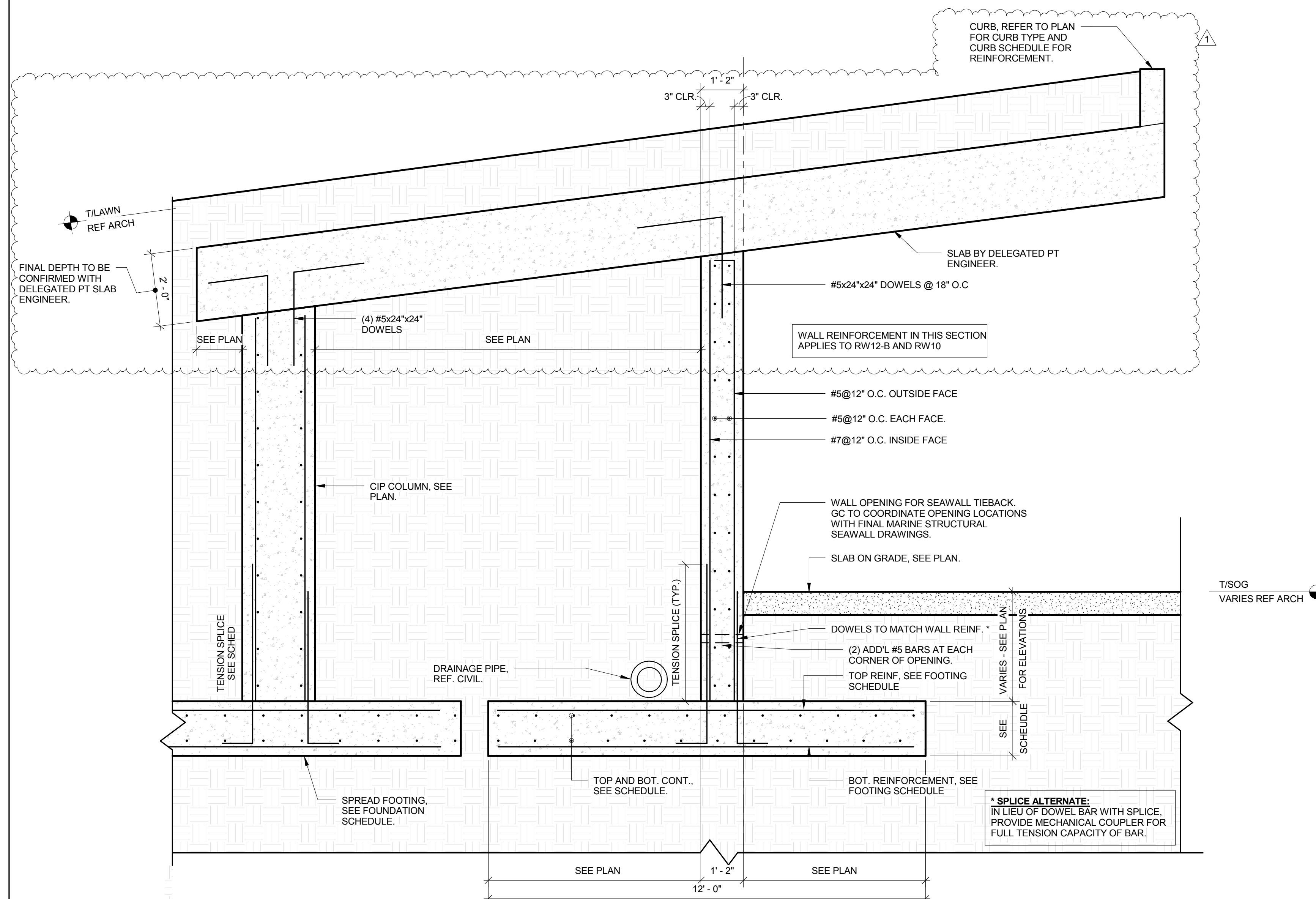
2 TILTED LAWN - SECTION B 1/2" = 1'-0"
