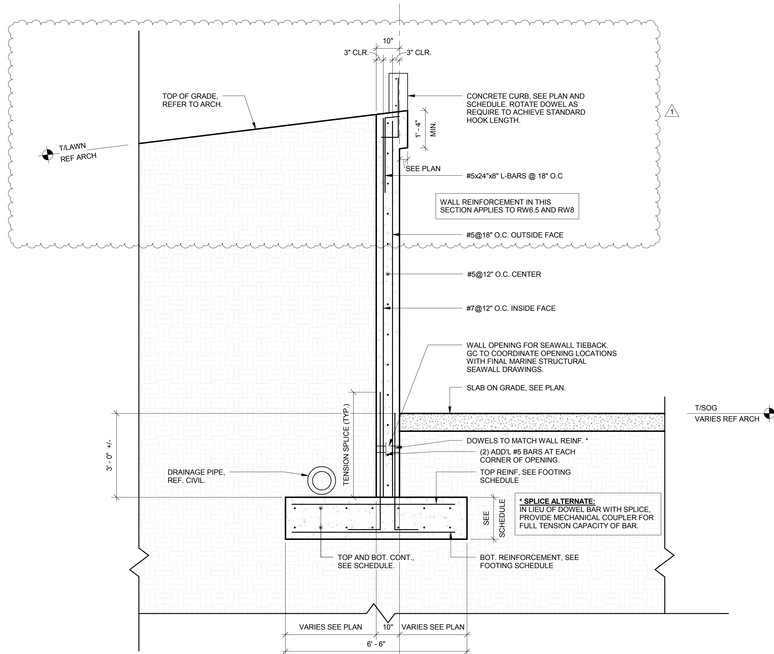
3 TILTED LAWN - SECTION C 1/2" = 1'-0"
