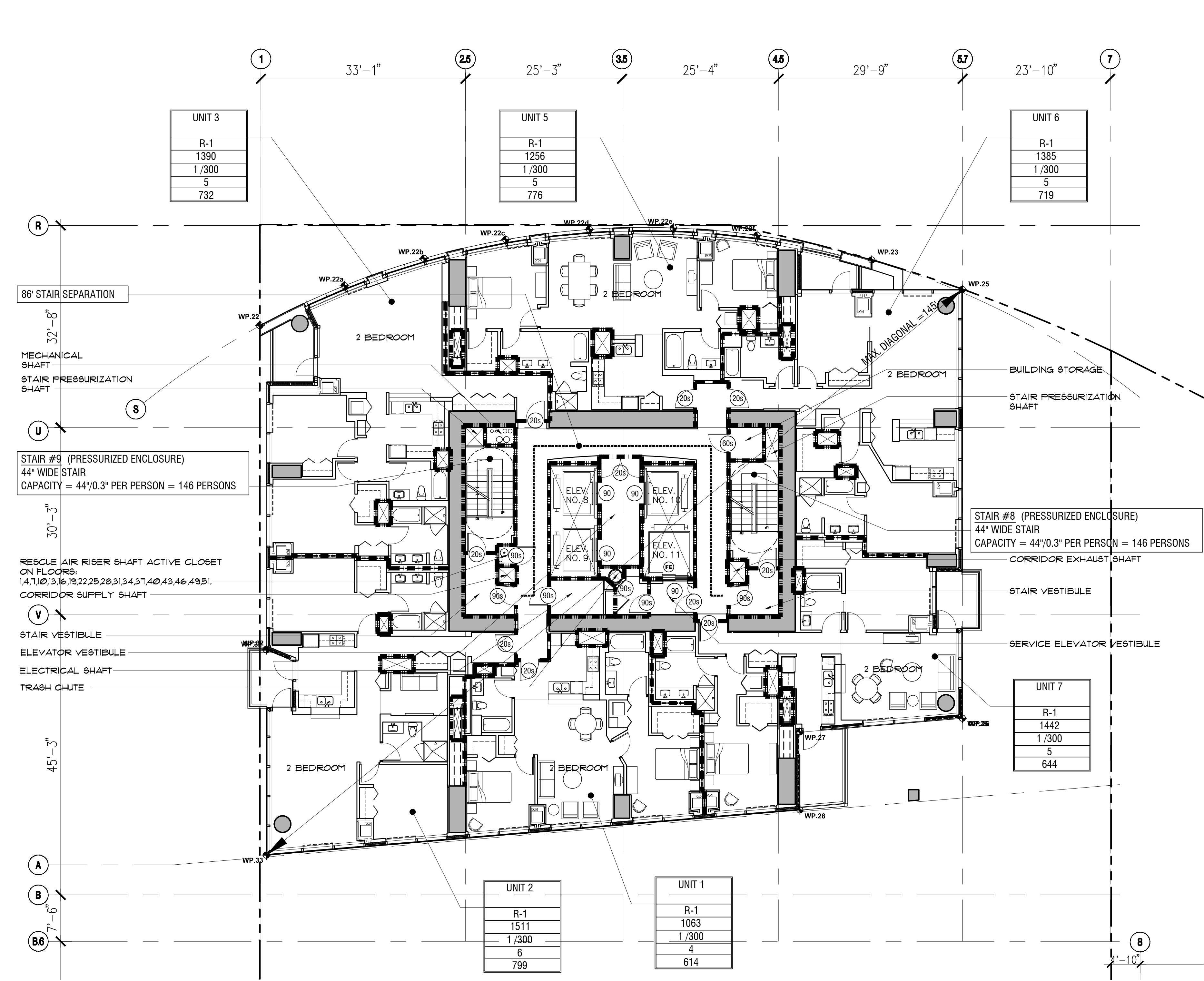
3 LEVELS 40 & 43 PLAN (OUTER OUTRIGGER) SCALE: 1"=1'-0"
