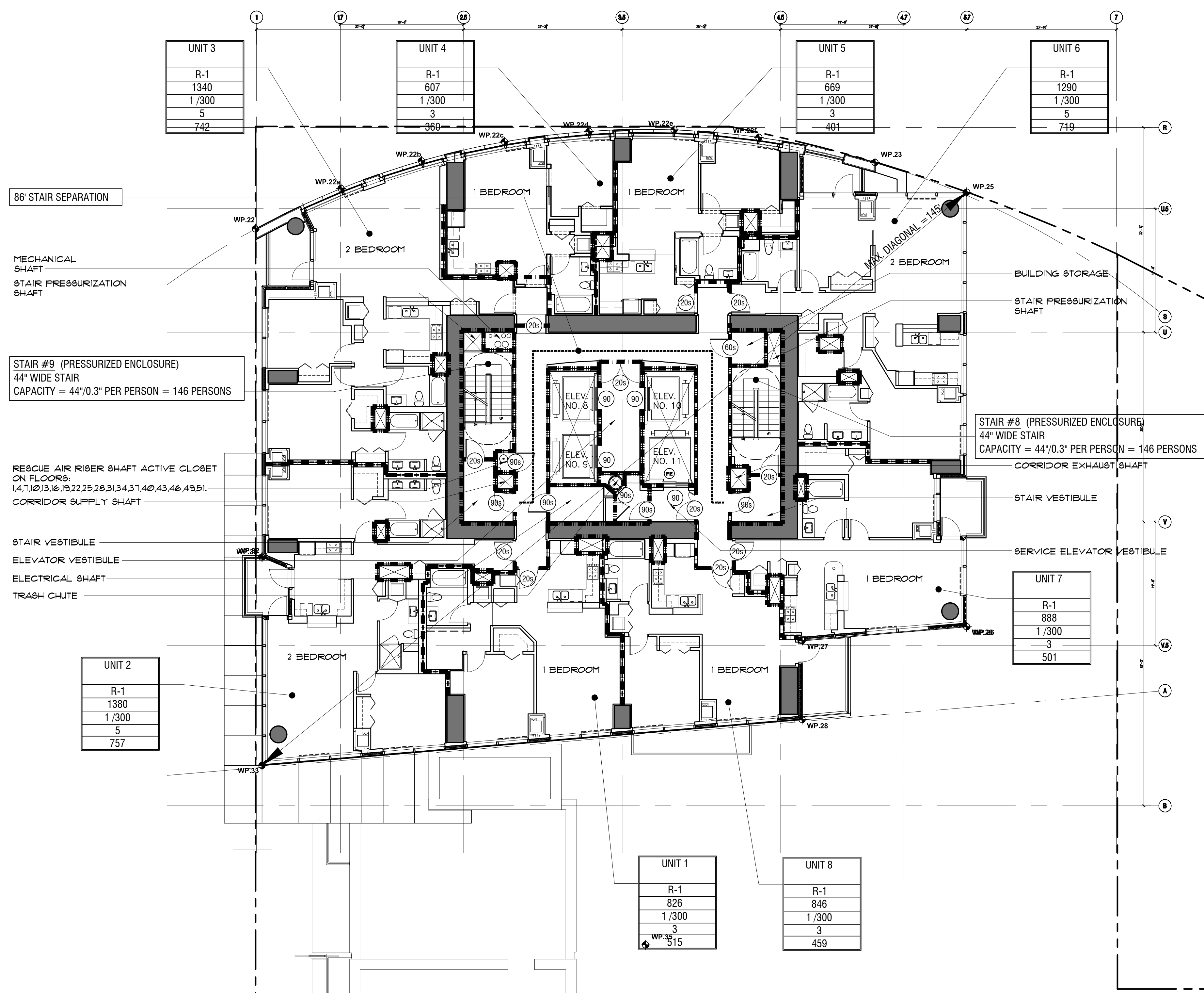
1 LEVELS 8-16 PLAN (LOWER TOWER) SCALE: 1"=1'-0"
