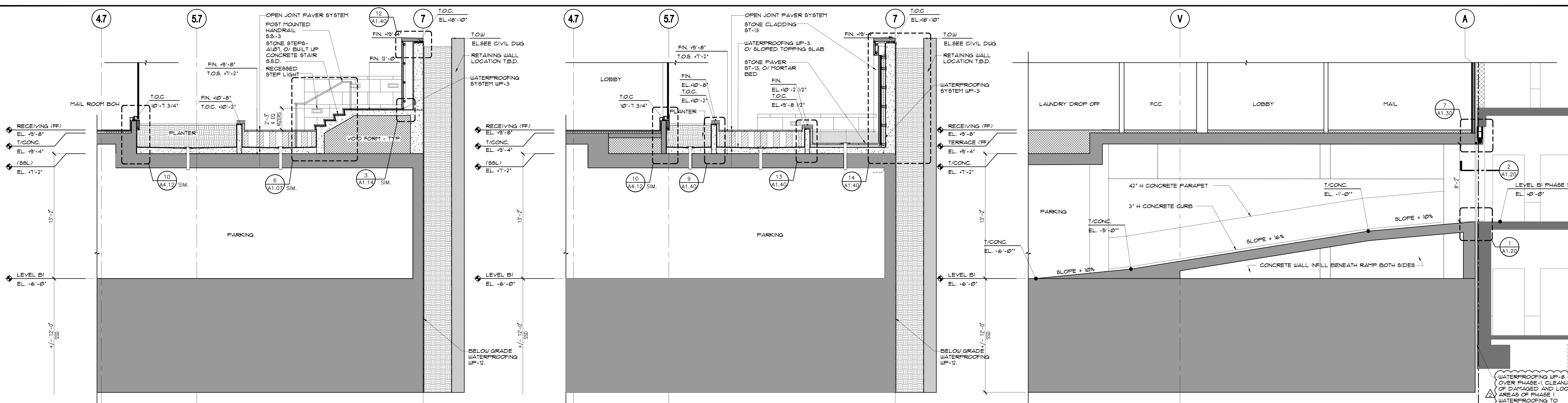
10 SECTION THROUGH LEVEL1 TERRACE SCALE: 1/4" = 1'-0" 9 SECTION THROUGH LEVEL1 TERRACE SCALE: 1/4" = 1'-0" 8 SECTION THROUGH LEVEL1 TERRACE SCALE: 1/4" = 1'-0"
