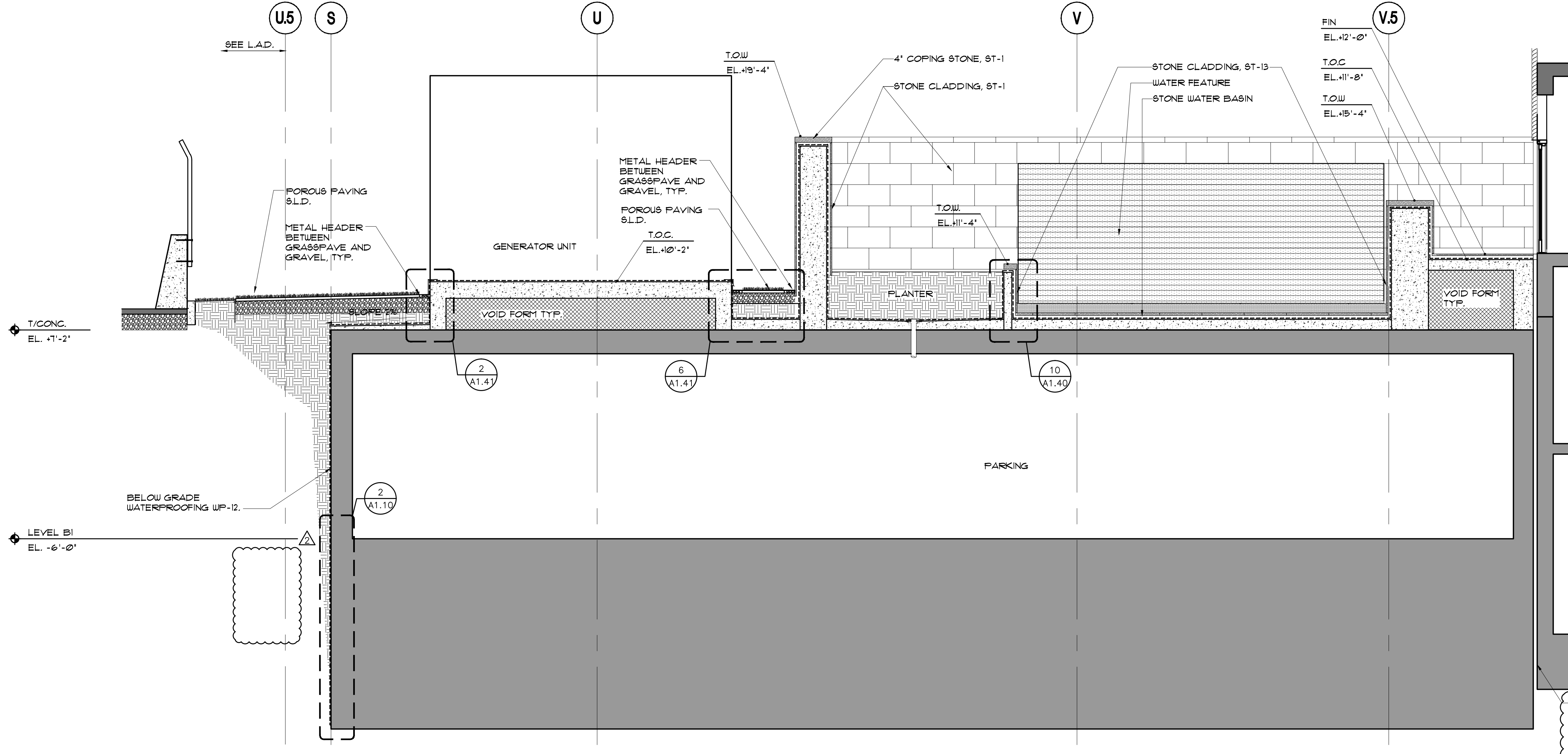
2 SECTION @ LEVEL 1 TERRACE LOOKING SOUTH SCALE: 1/4"=1'-0"
