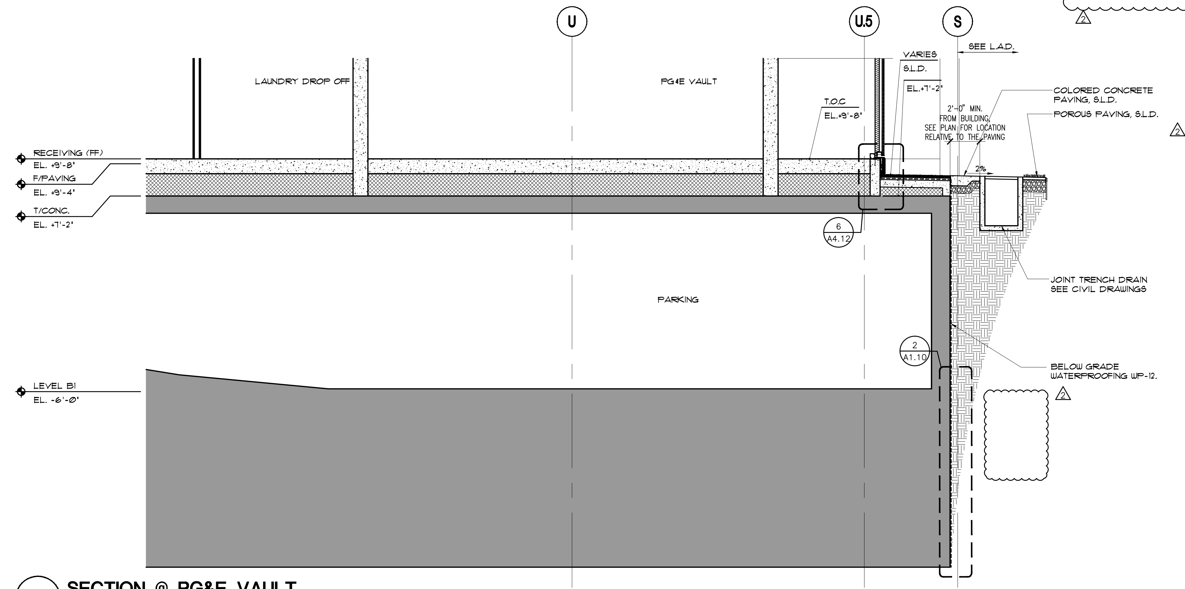
1 SECTION @ PG&E VAULT SCALE: 1/4"=1'-0"
