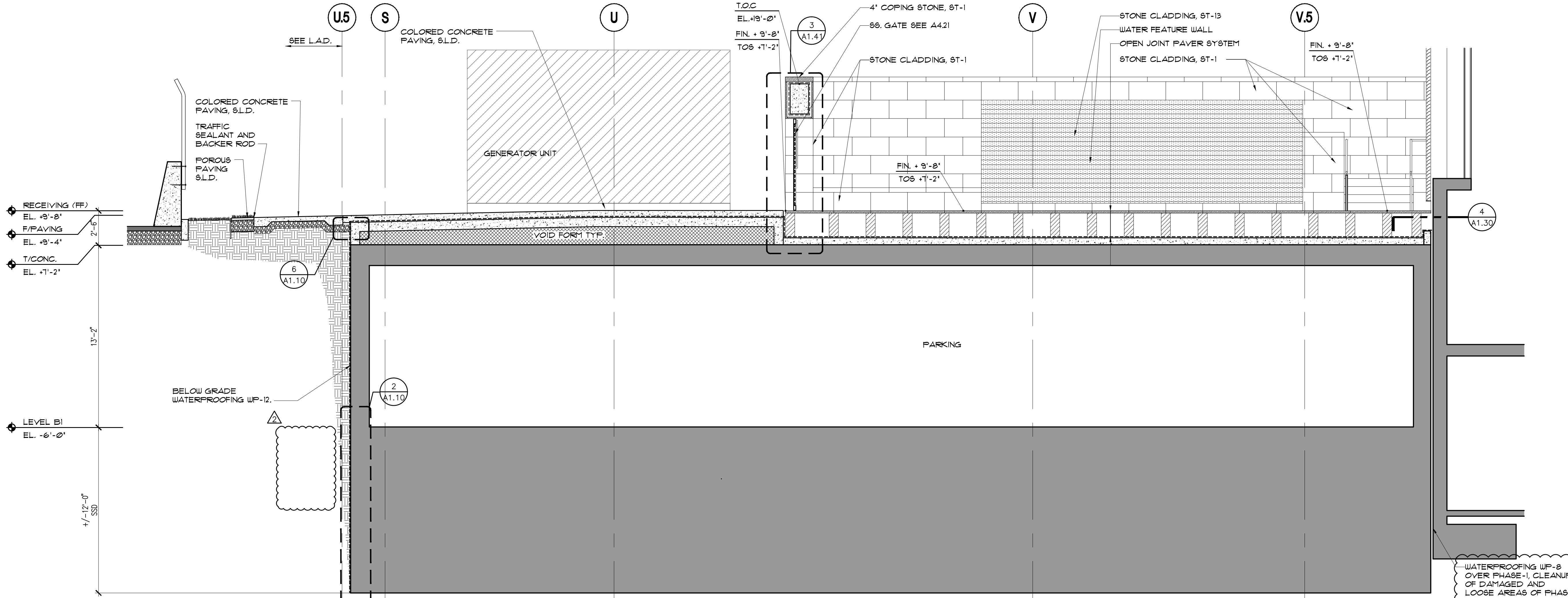
3 SECTION @ LEVEL 1 TERRACE LOOKING SOUTH SCALE: 1/4"=1'-0"
