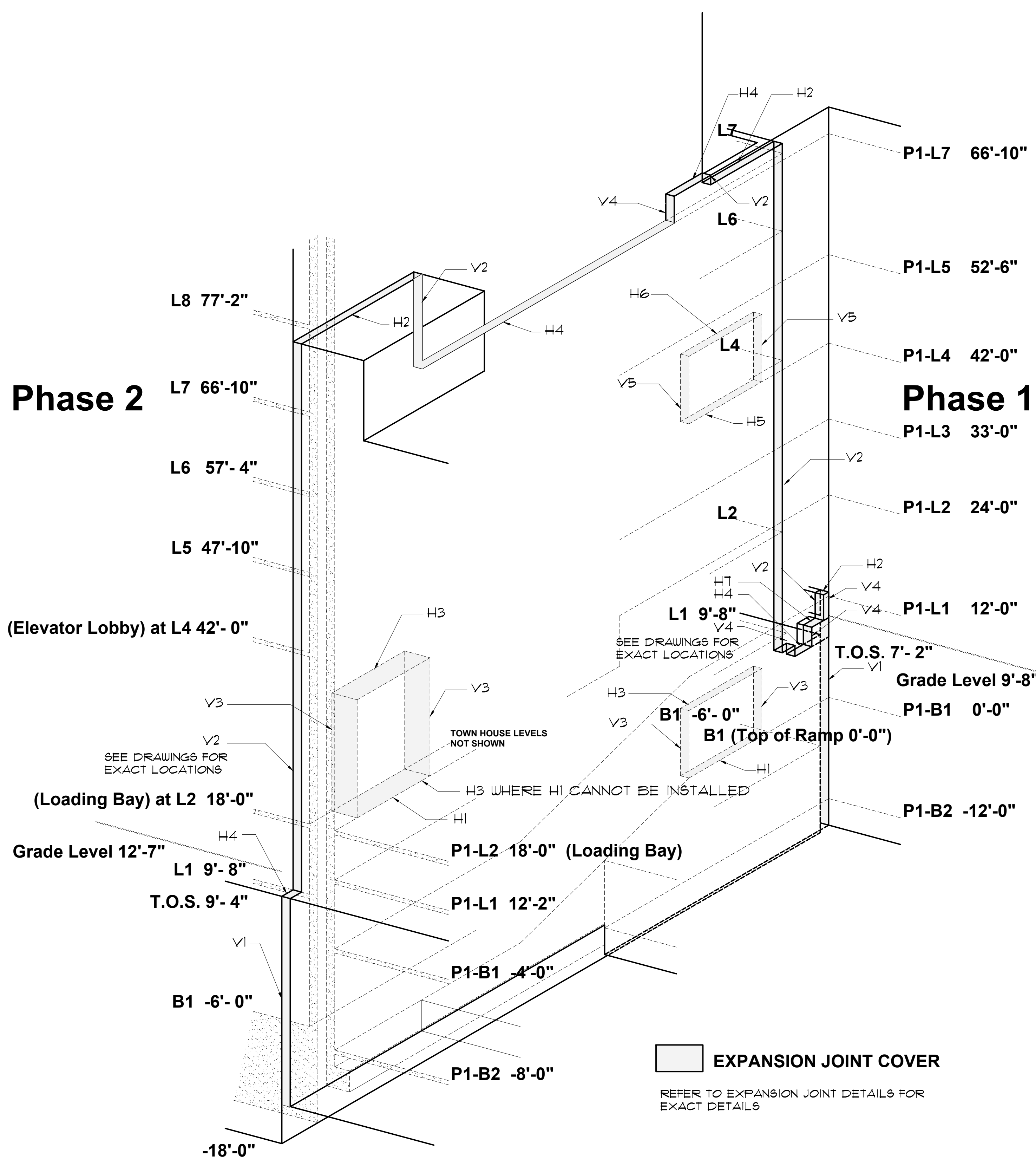
9 EXPANSION JOINT DIAGRAM BETWEEN PHASE 1 AND PHASE 2 SCALE: 6" = 1'-0"
