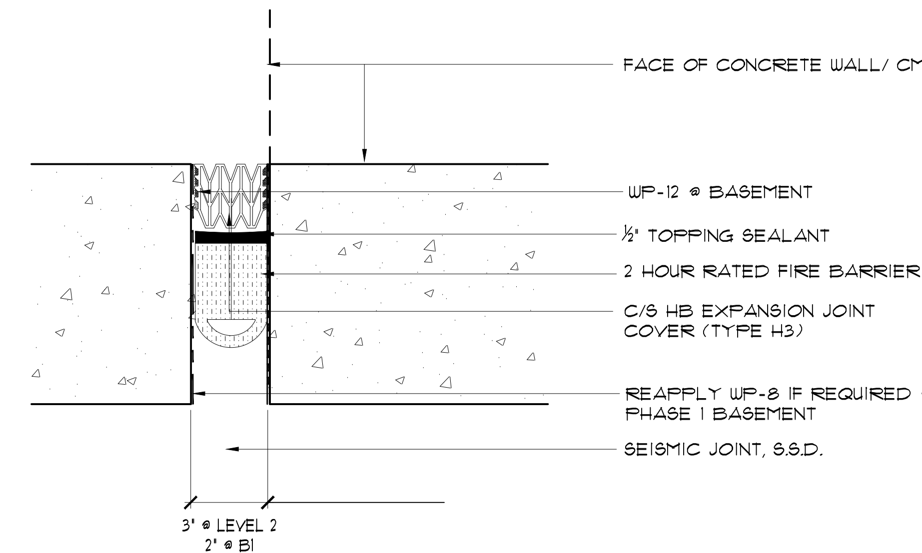
2 E.J. COVER (TYPE H3 and V3) SCALE: 3" = 1'-0"
