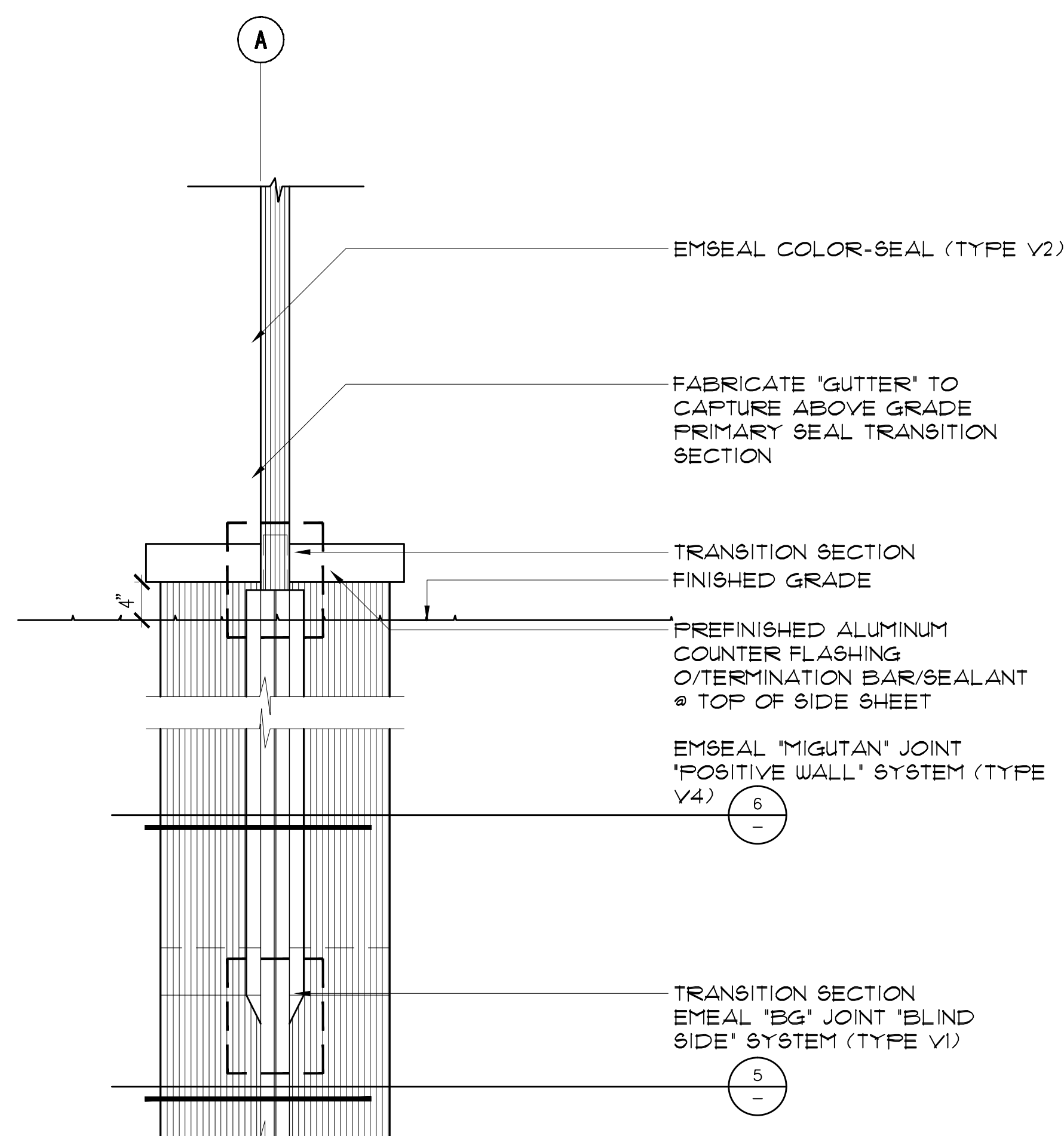
7 A LINE SEISMIC JOINT CRITERIA SCALE: 1" = 1'-0"
