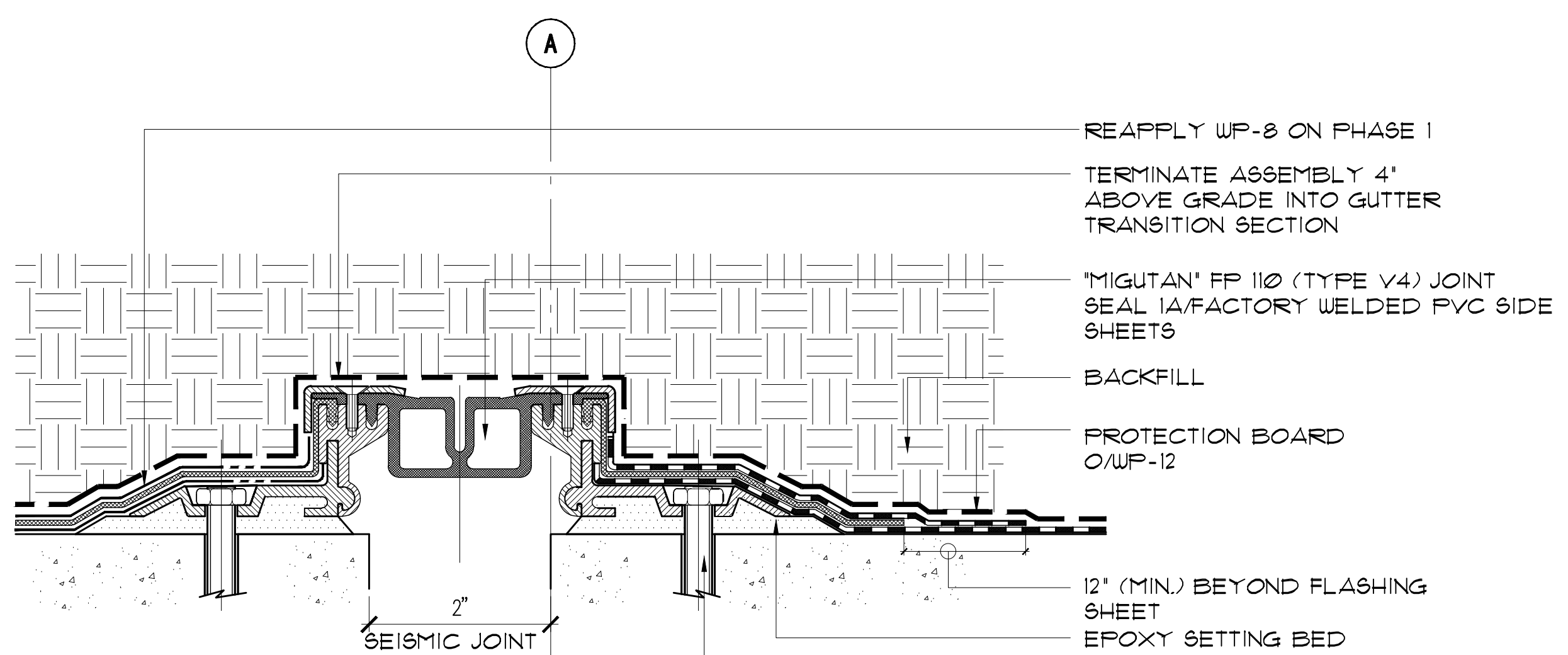
6 BELOW GRADE "POSITIVE SIDE" PLAN DETAIL (TYPE V5) SCALE: 6" = 1'-0"
