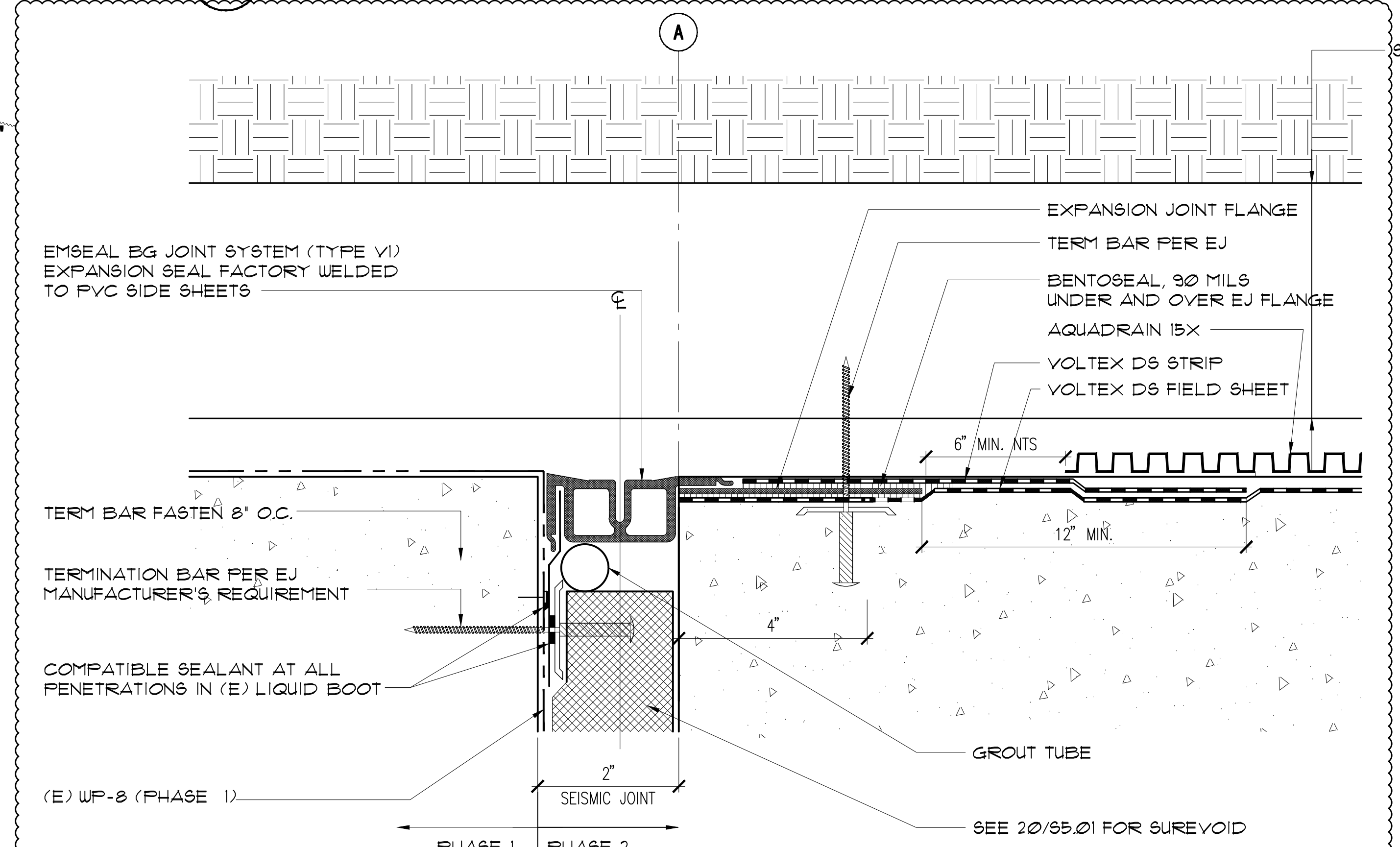
5 BELOW GRADE "BLIND WALL" PLAN DETAIL (TYPE V1) SCALE: 6" = 1'-0"
