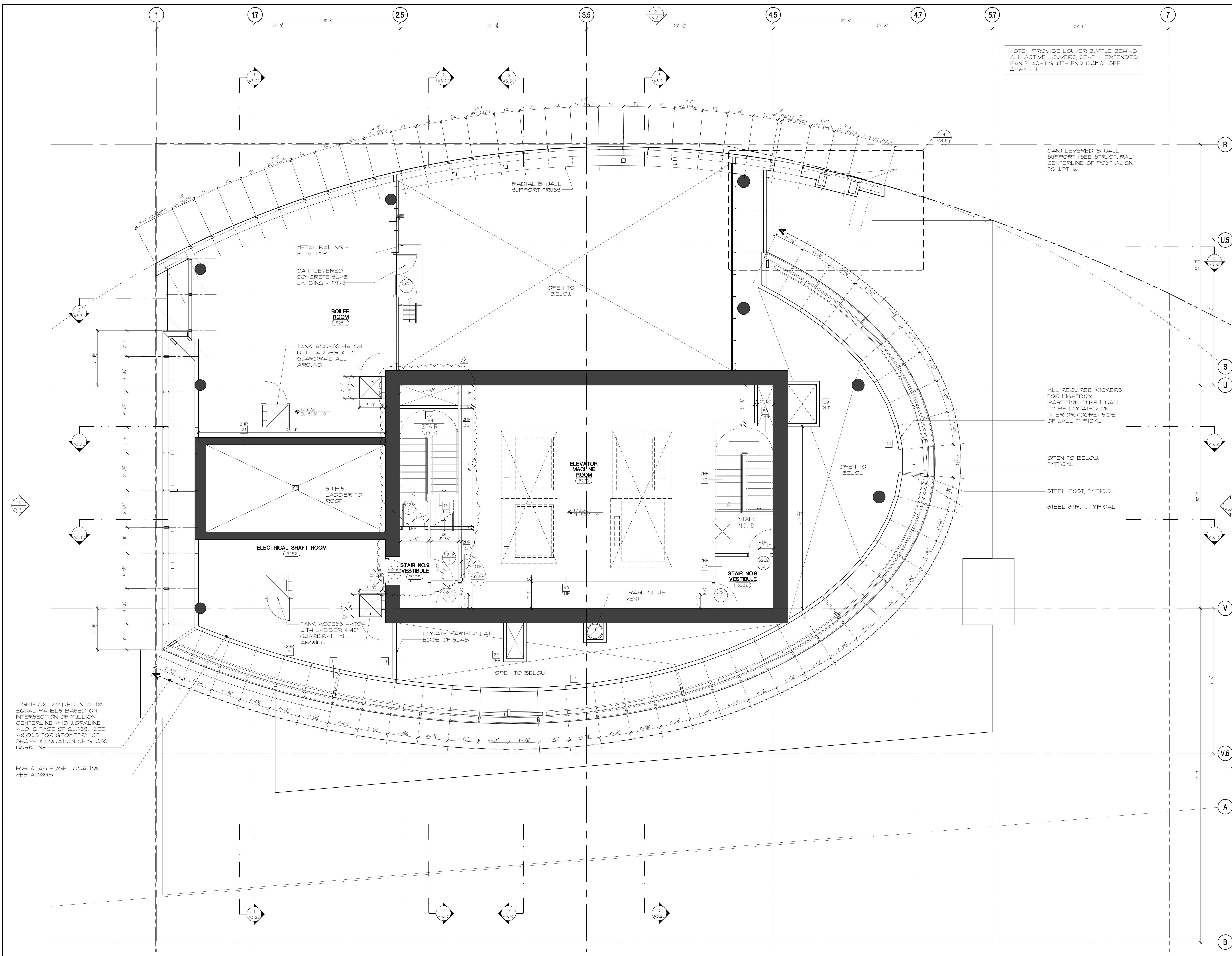
LEVEL 52 PLAN (MECHANICAL PENTHOUSE) SCALE: 1/4"=1'-0"
