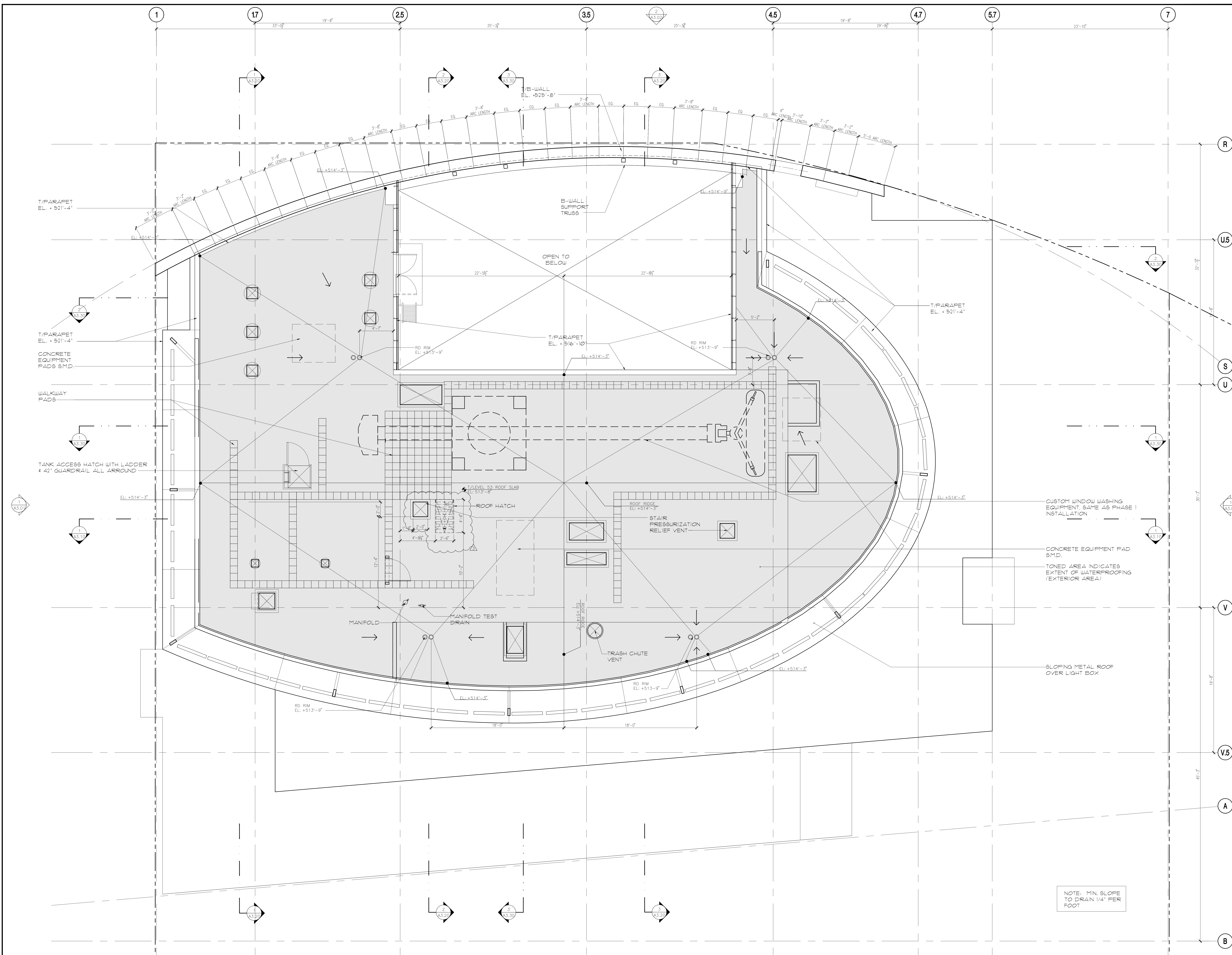
LEVEL 53 (ROOF) PLAN SCALE: 1/4"=1'-0"
