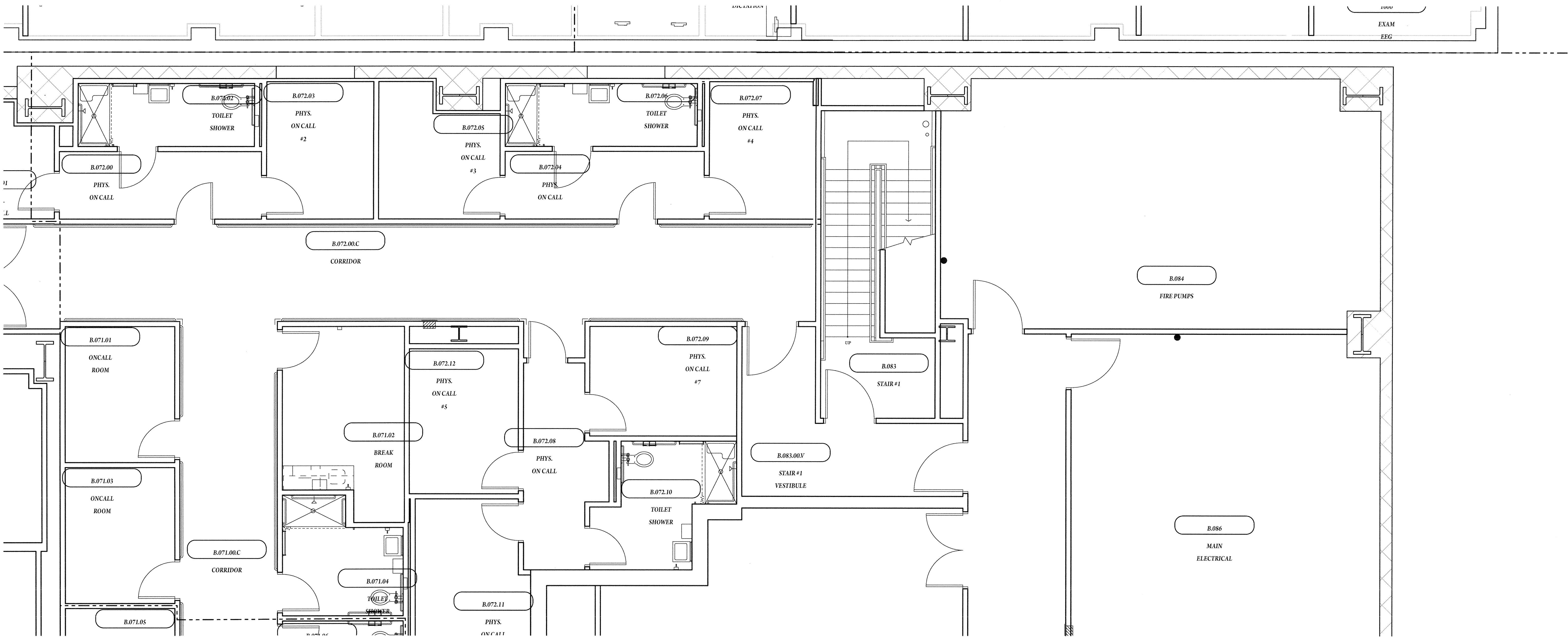
B6 B FURNITURE PLAN SCALE: 1/4" = 1'-0"
