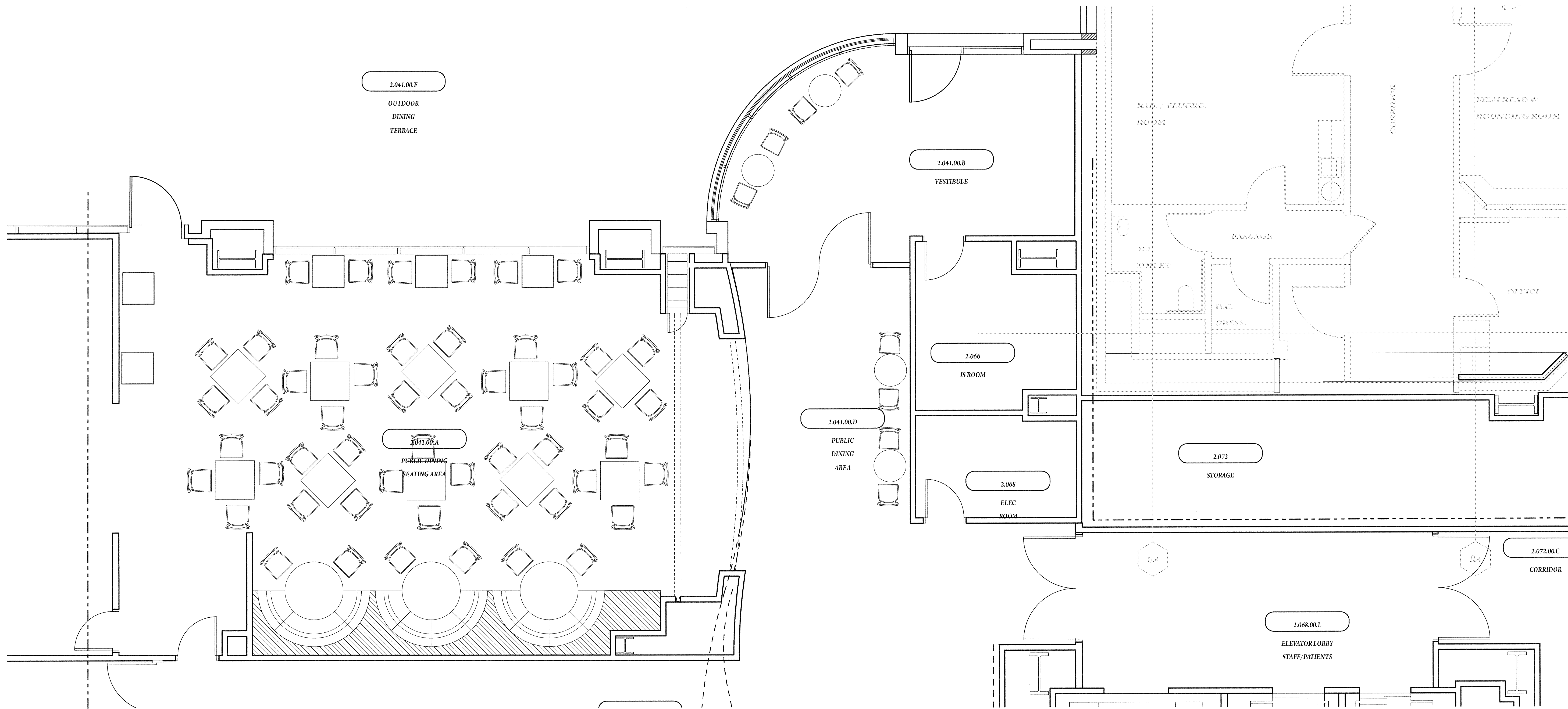
B6 Furniture Plan SCALE: 1/4" = 1'-0"
