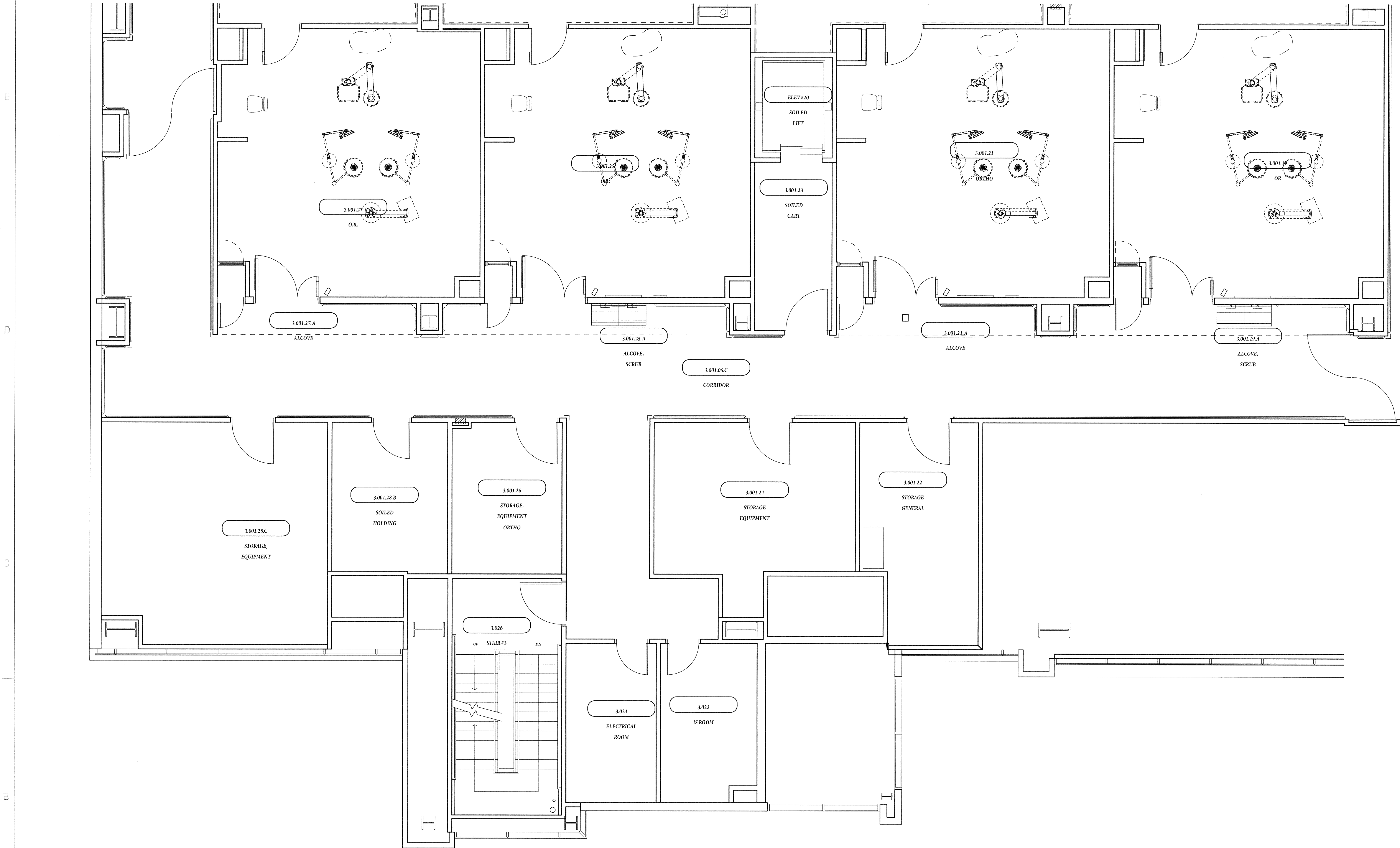
B6 Furniture Plan SCALE: 1/4" = 1'-0"
