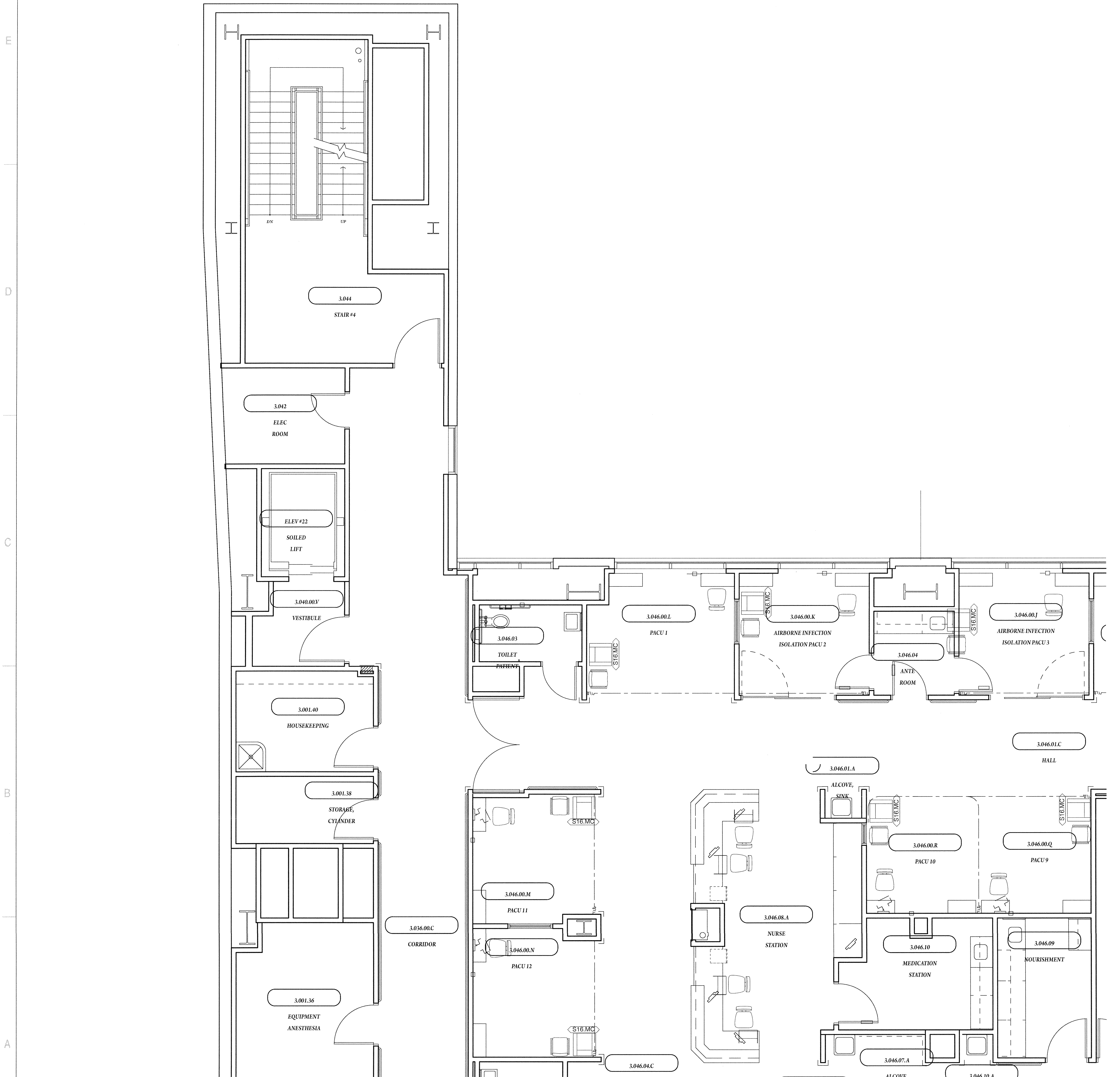
A6 Furniture Plan SCALE: 1/4" = 1'-0"
