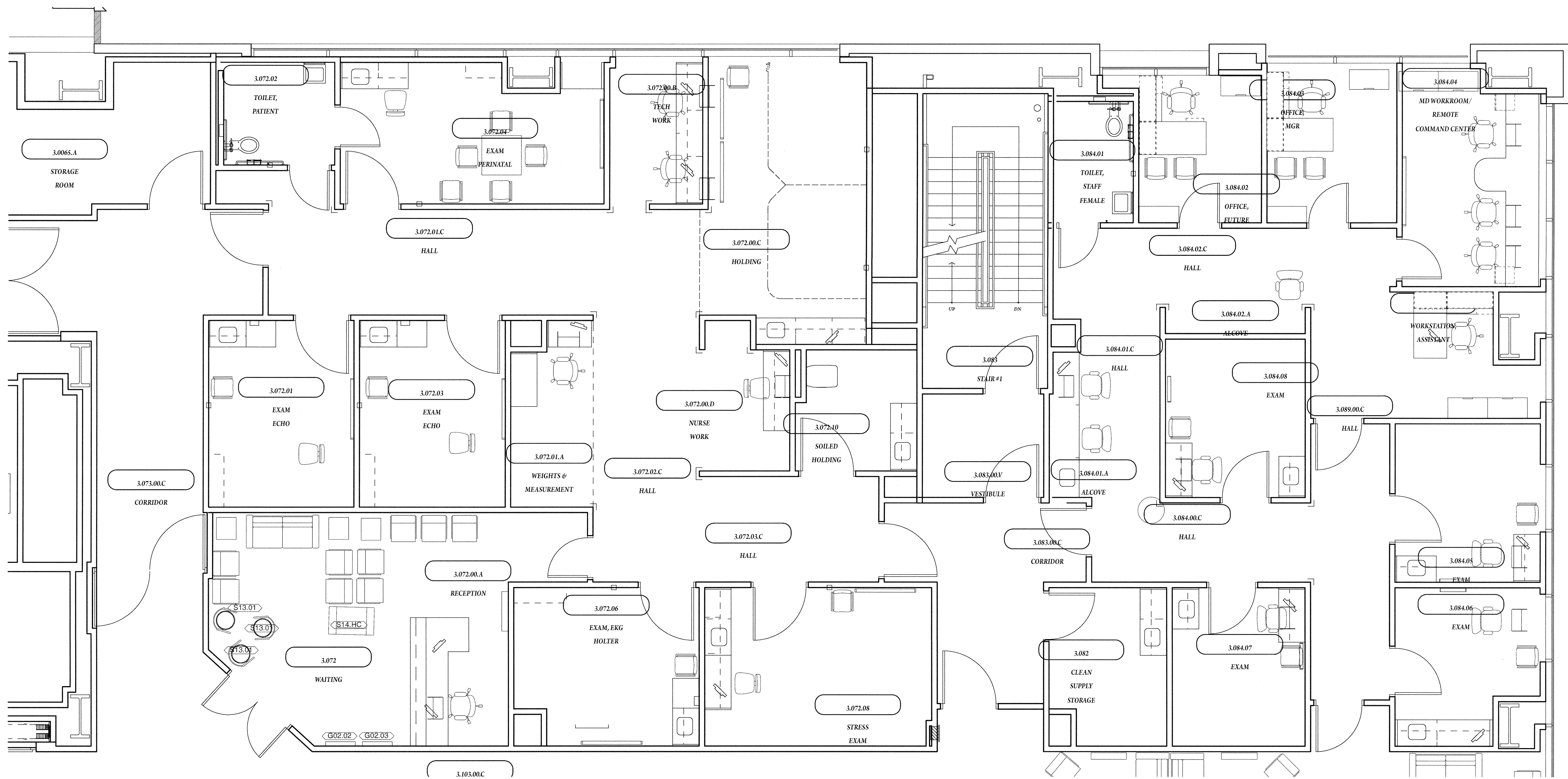
B6 Furniture Plan SCALE: 1/4" = 1'-0"
