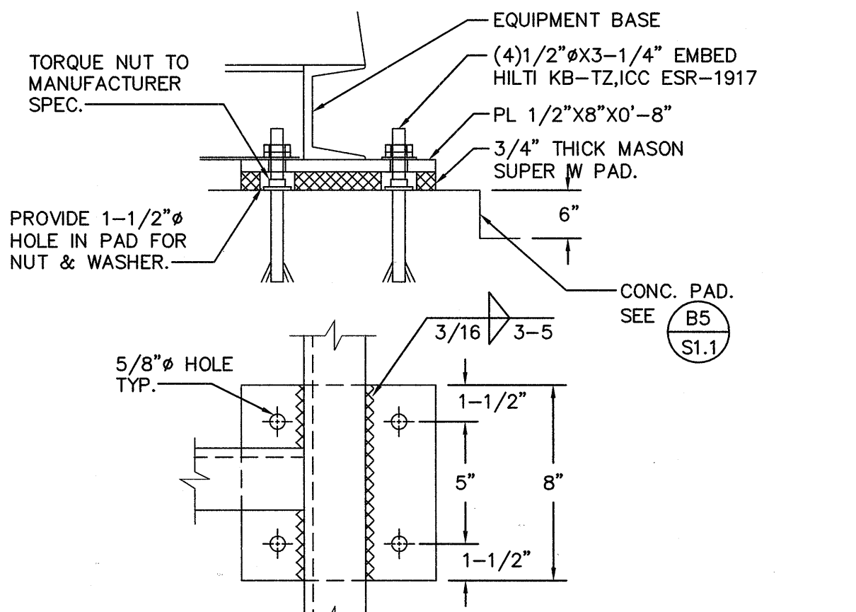
ANCHORAGE DETAIL FOR STEAM BOILERS' DEAERATOR (DA-1)
