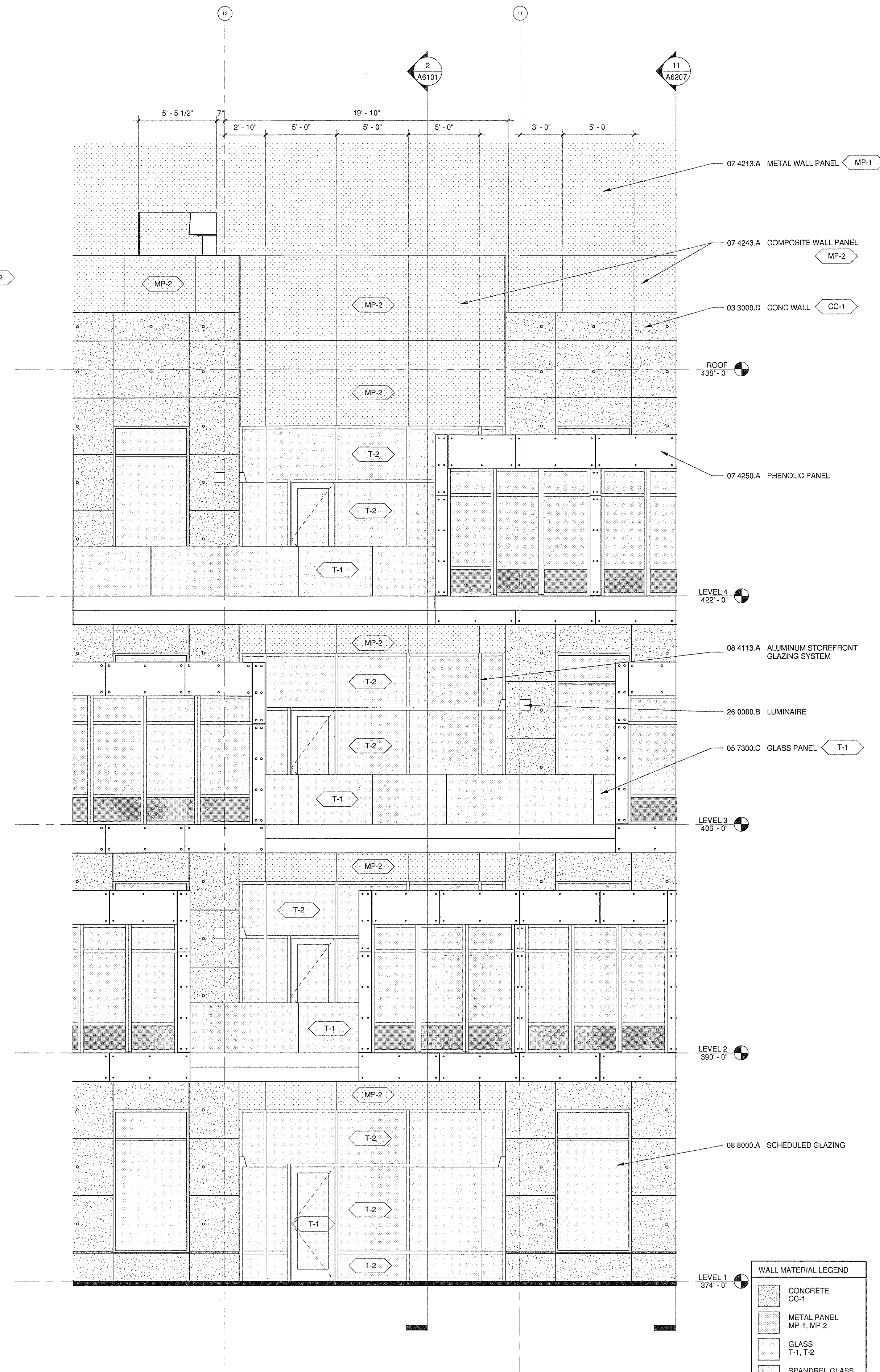
1 PARTIAL ELEV. - WEST @ BREAK RM. A5101/A5202 1/4" = 1'-0"
