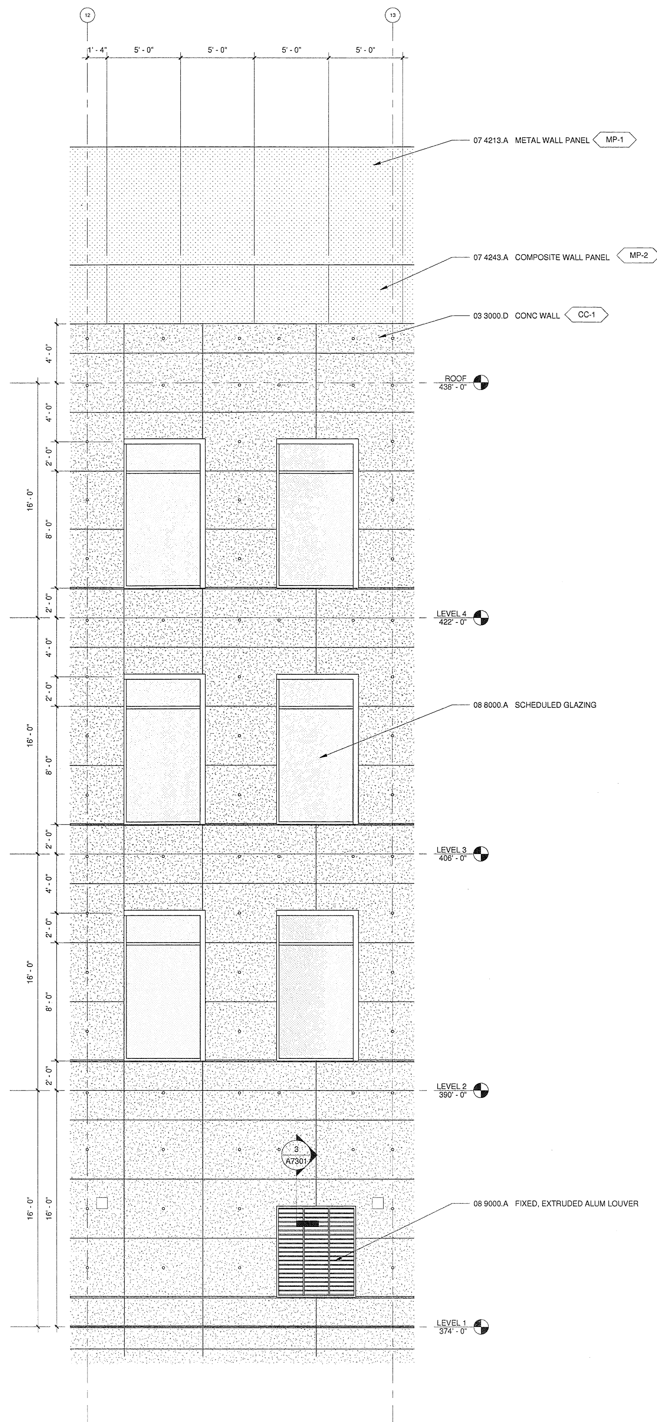
3 PARTIAL ELEV. - TYPICAL BAY A5102/A5202 1/4" = 1'-0"
