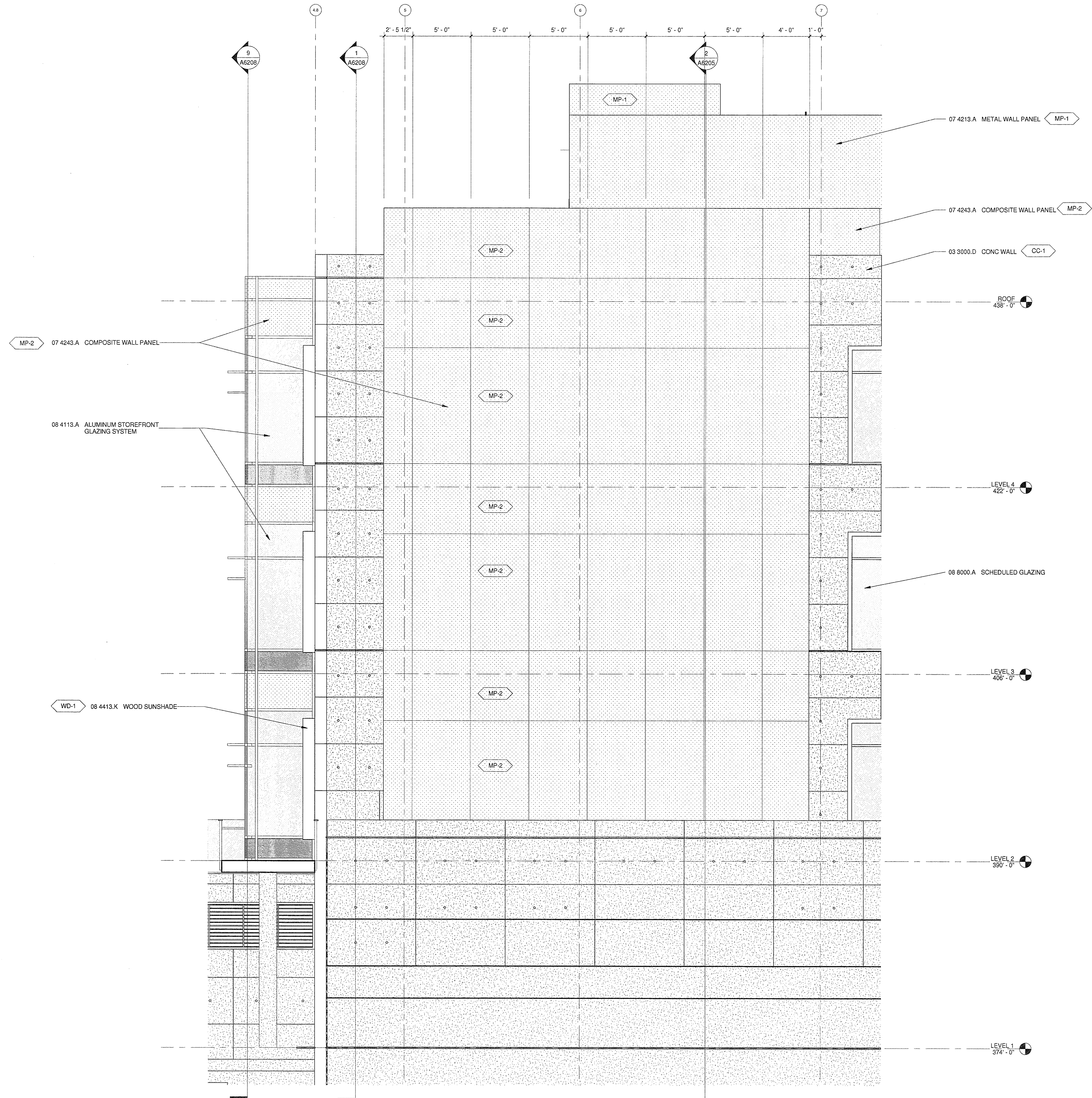
2 PARTIAL ELEV. - EAST CORNER A5102/A5203 1/4" = 1'-0"
