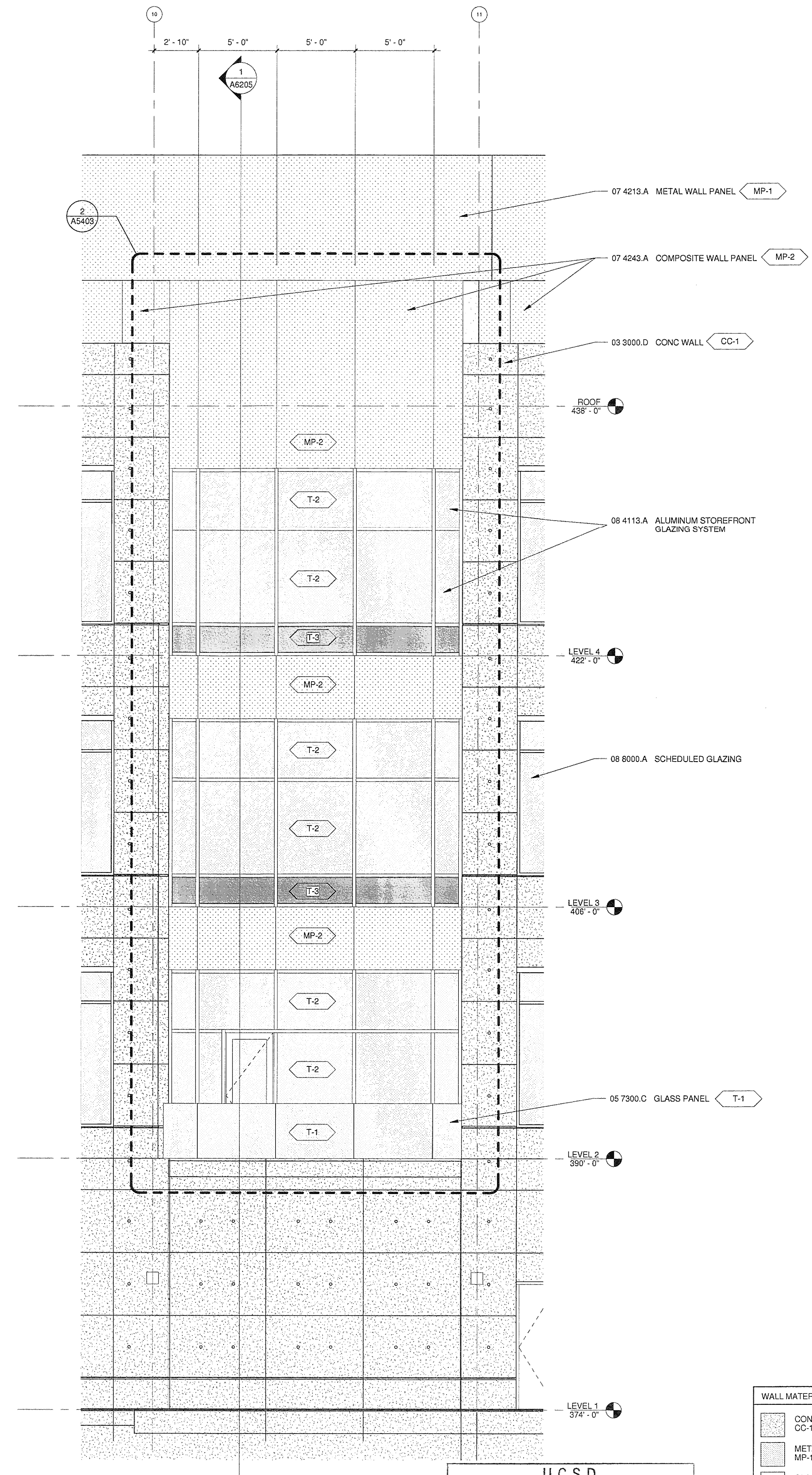
1 PARTIAL ELEV. - EAST BREAK A5102/A5203 1/4" = 1'-0"
