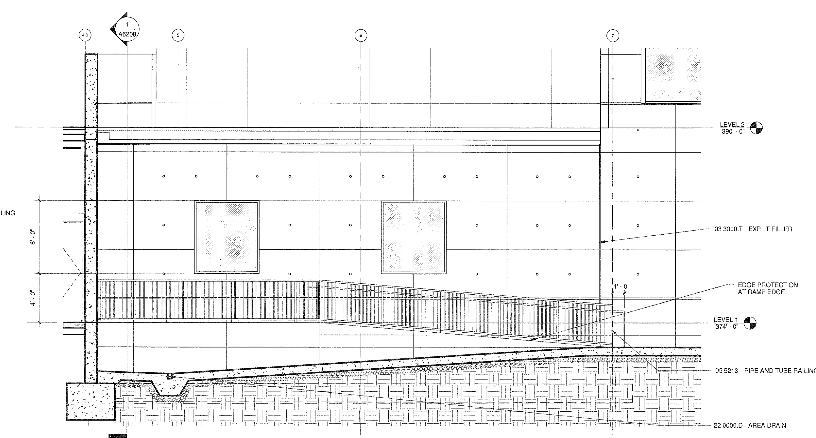
1 RAMP ELEVATION A2110/A5208 1/4" = 1'-0"
