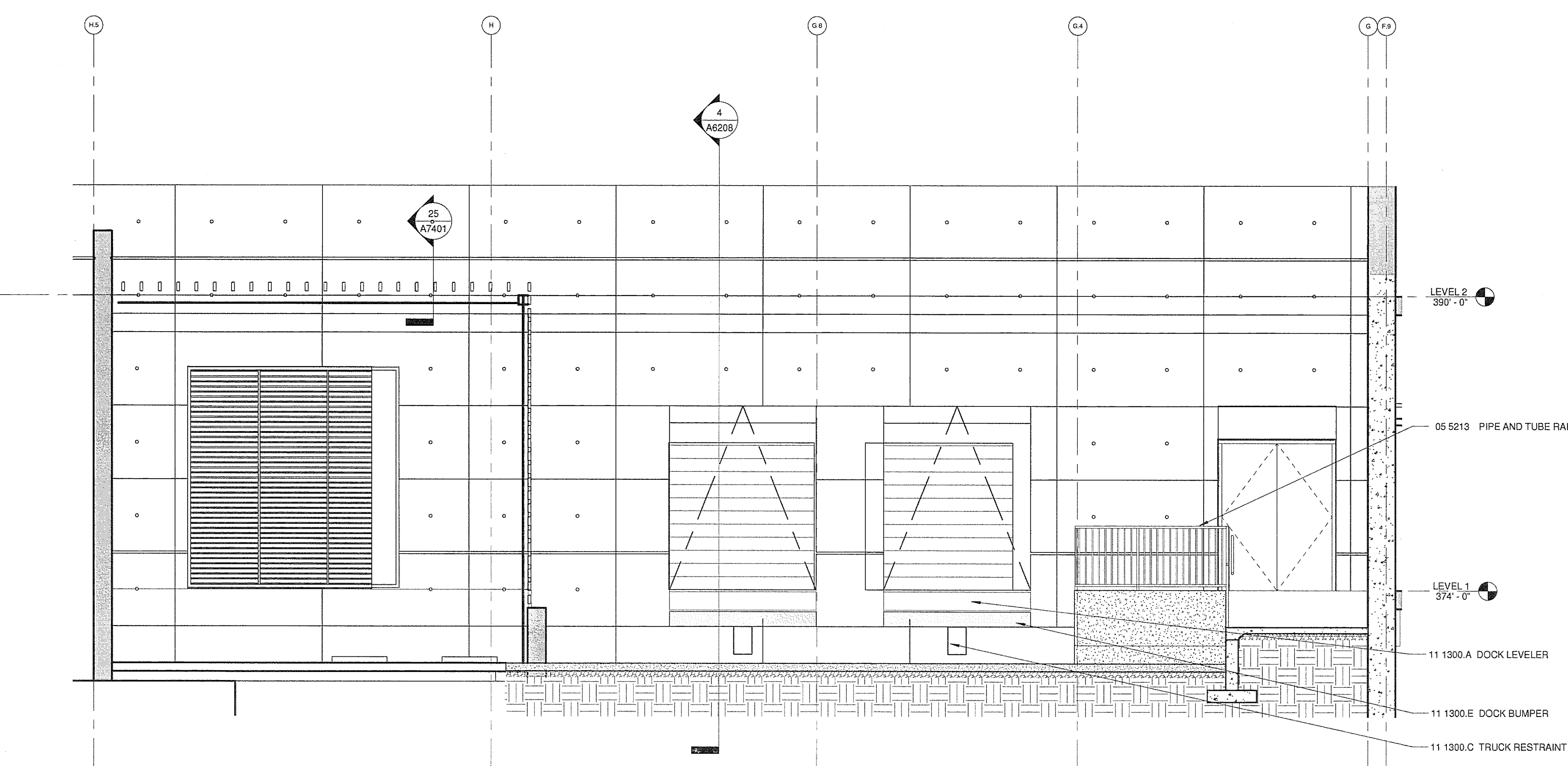
7 RAMP SECTION/ ELEVATION A2110/A5208 1/4" = 1'-0"
