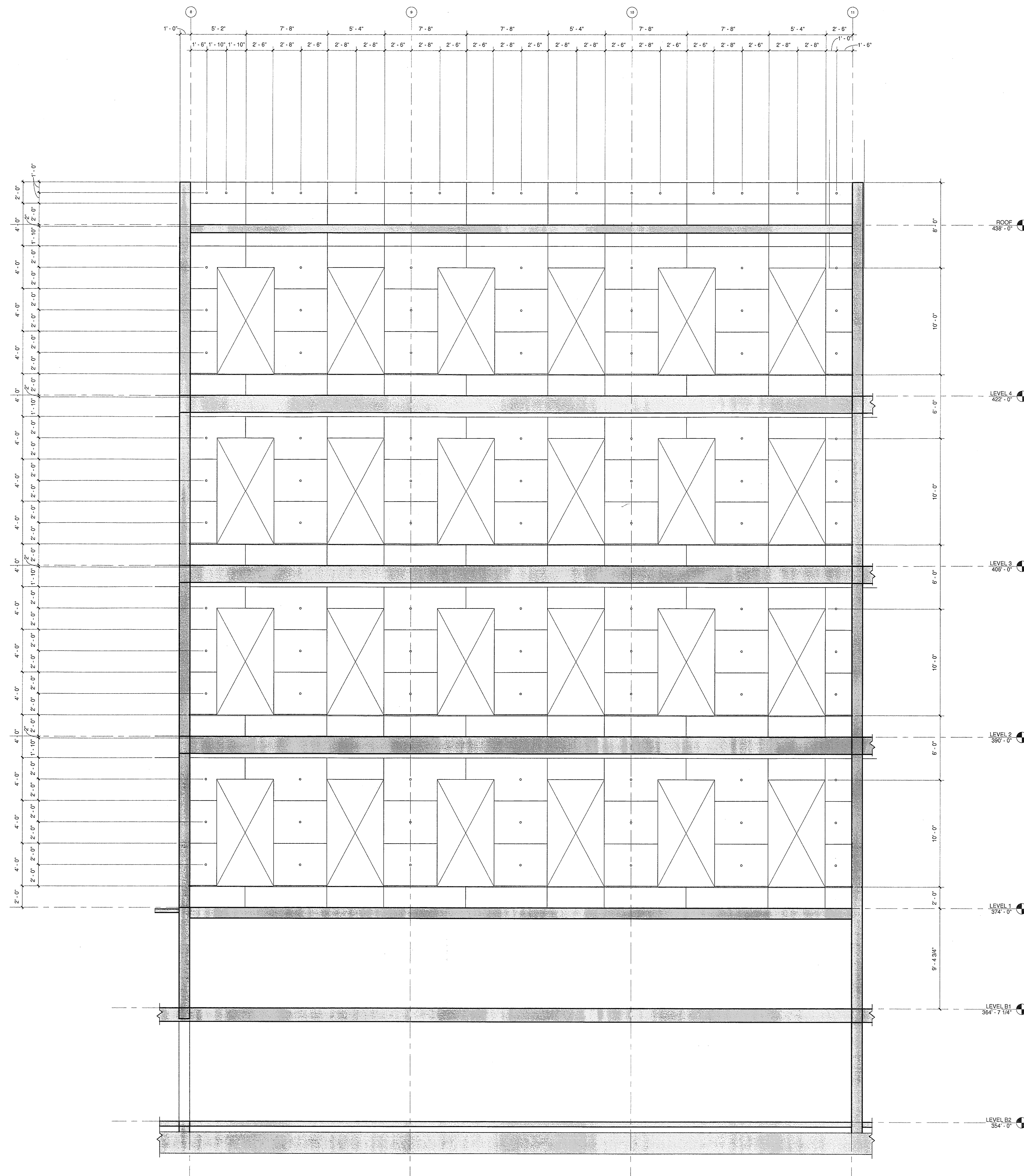
2 INTERIOR CONC. WALL ELEV.
