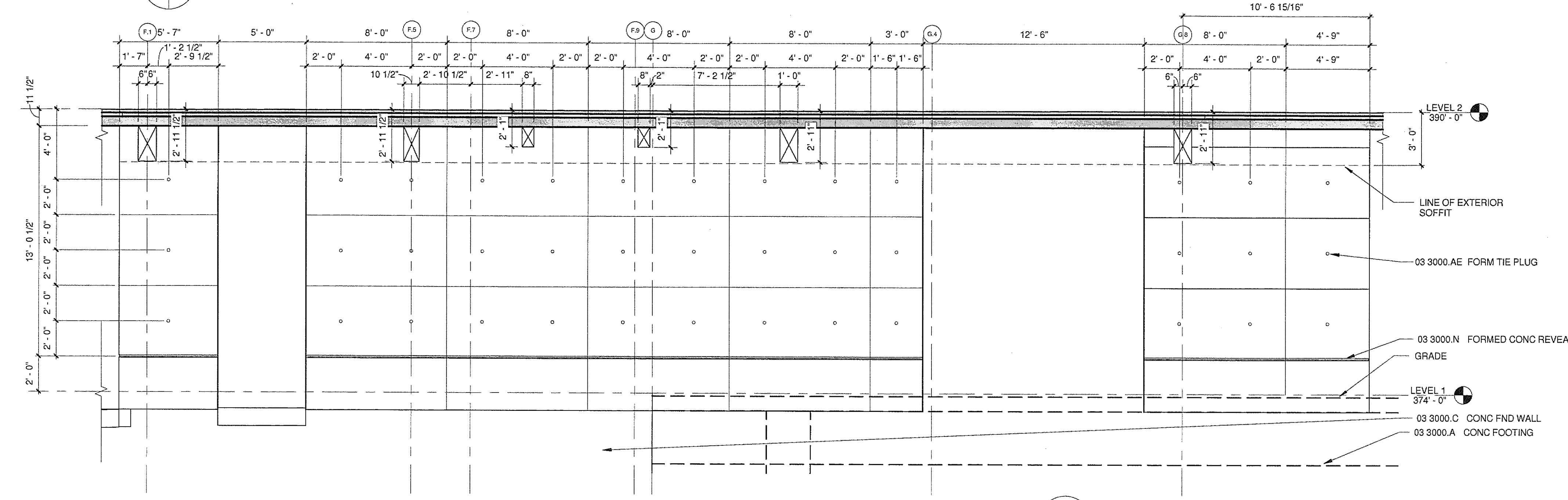
6 EXTERIOR CONC. WALL ELEV.
