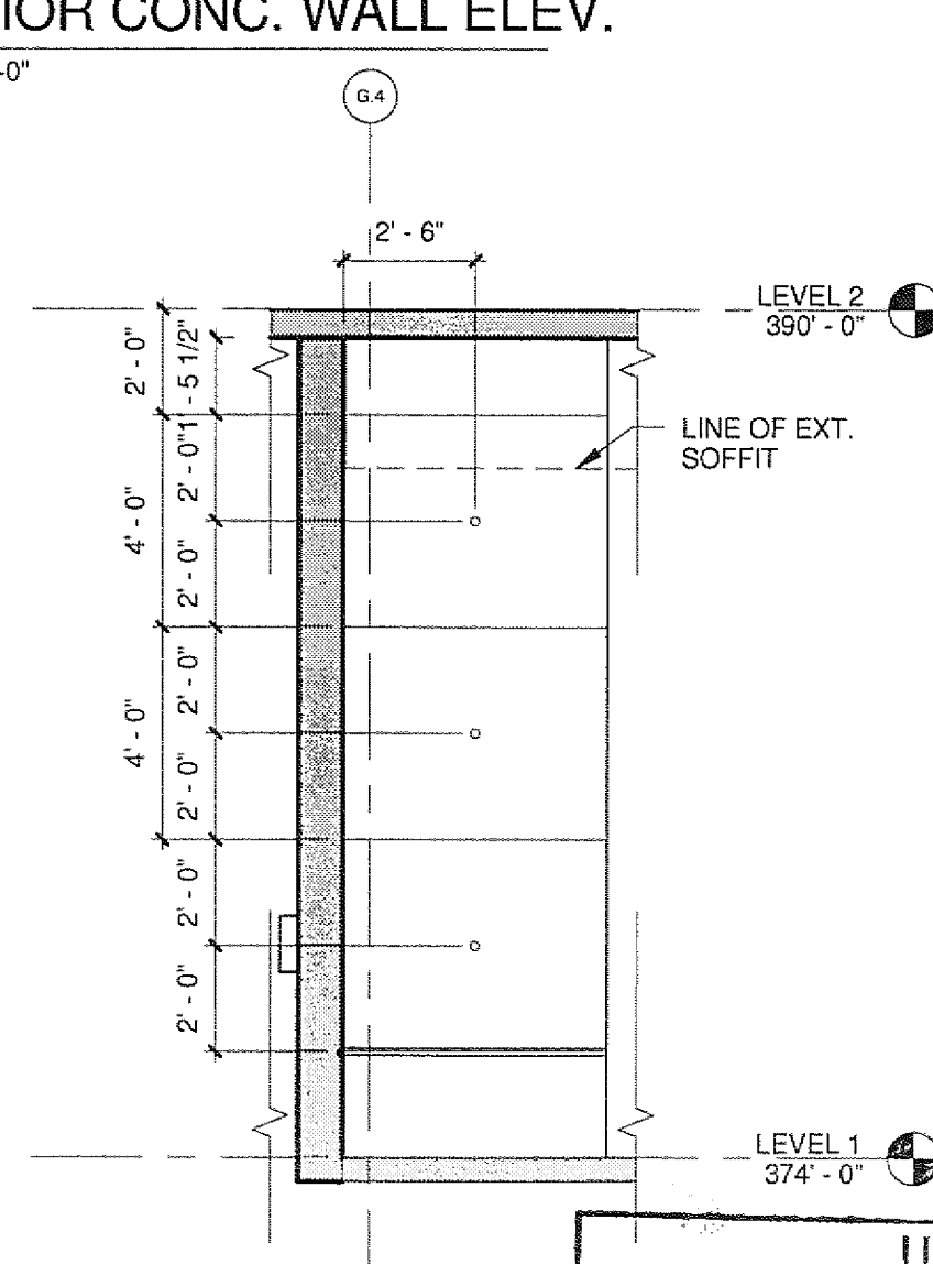
5 EXTERIOR CONC. WALL ELEV
