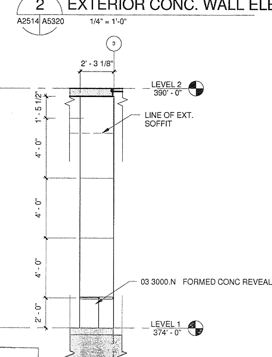
EXTERIOR CONC. WALL ELEV
