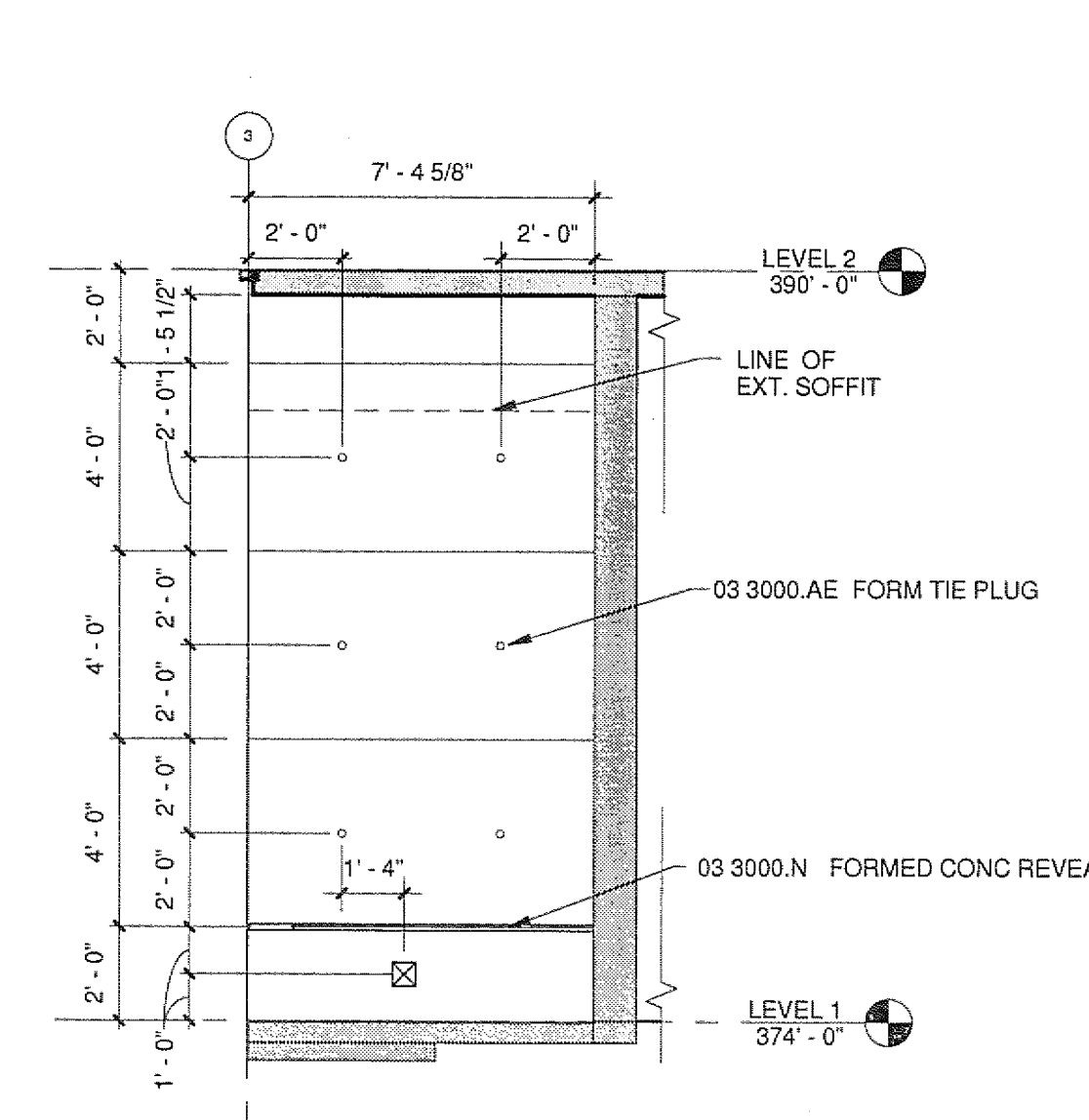
9 EXTERIOR CONC. WALL ELEV. A2514/A5320 1/4" = 1'-0"
