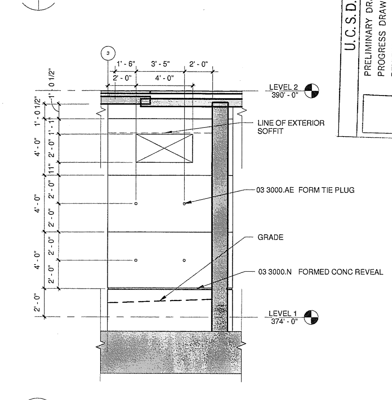
2 EXTERIOR CONC. WALL ELEV
