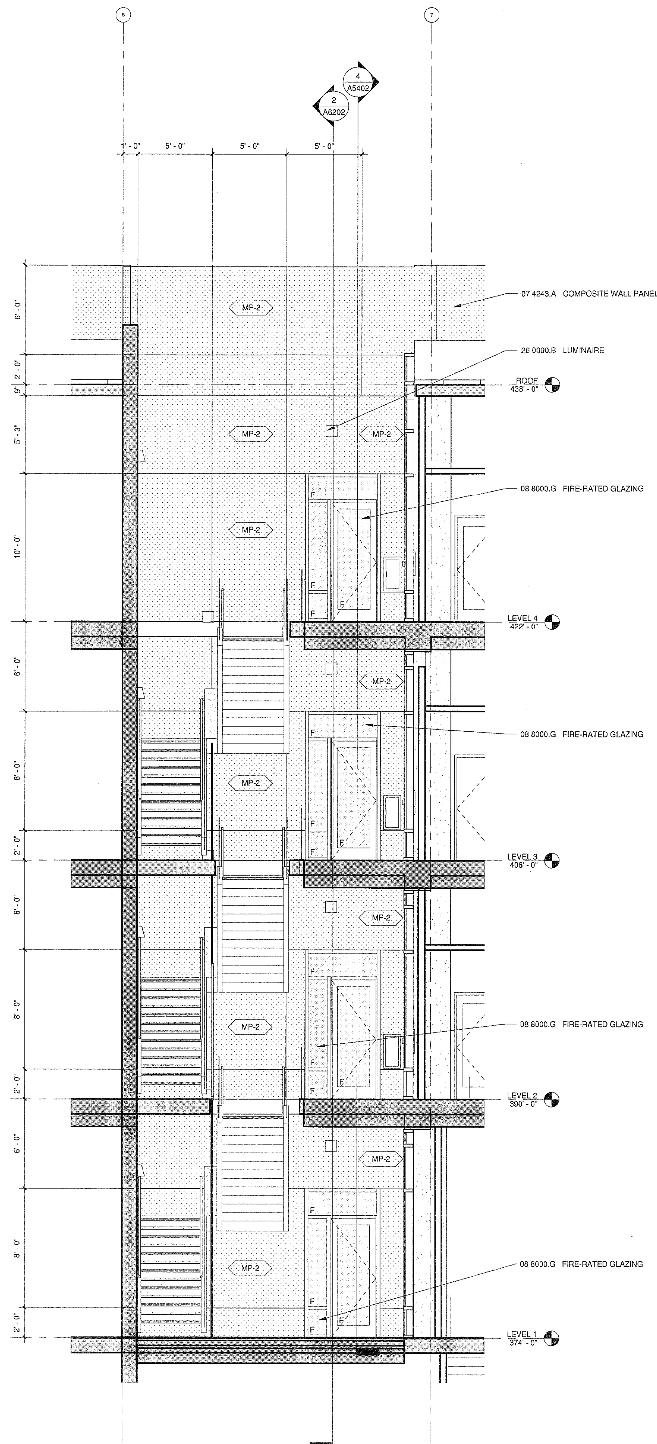
3 SECT. ELEV. @ STAIR#4 A5202 AS403 1/4" = 1'-0"
