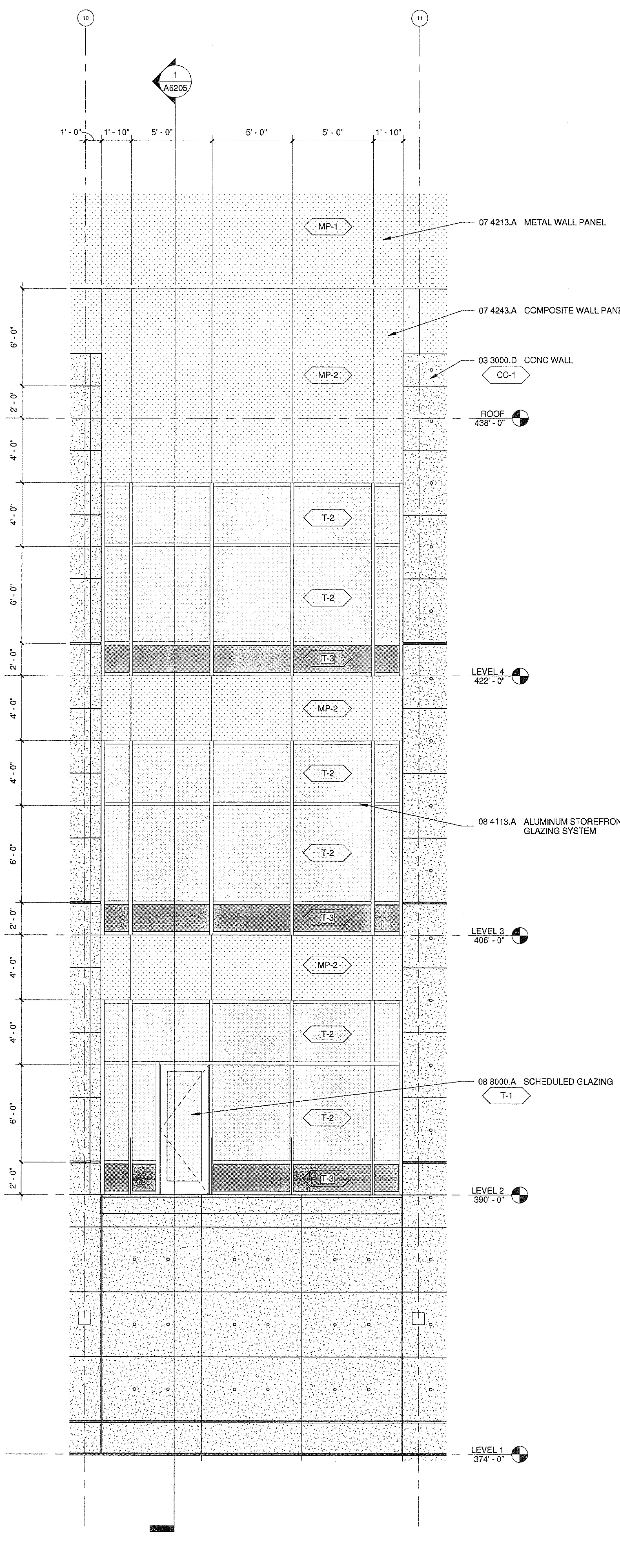
2 CW EAST ELEV BREA A5202 AS403 1/4" = 1'-0"
