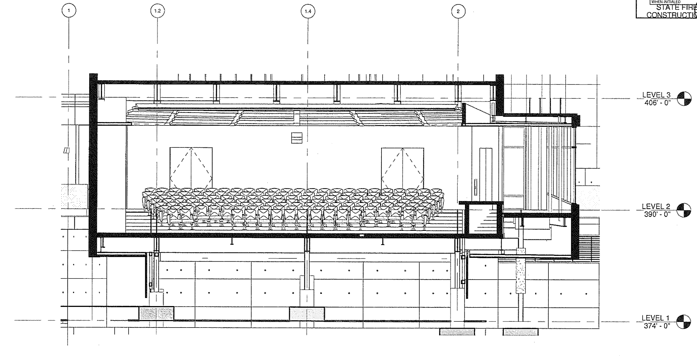
3 BUILDING SECTION A2110/A6102 1/8" = 1'-0"
