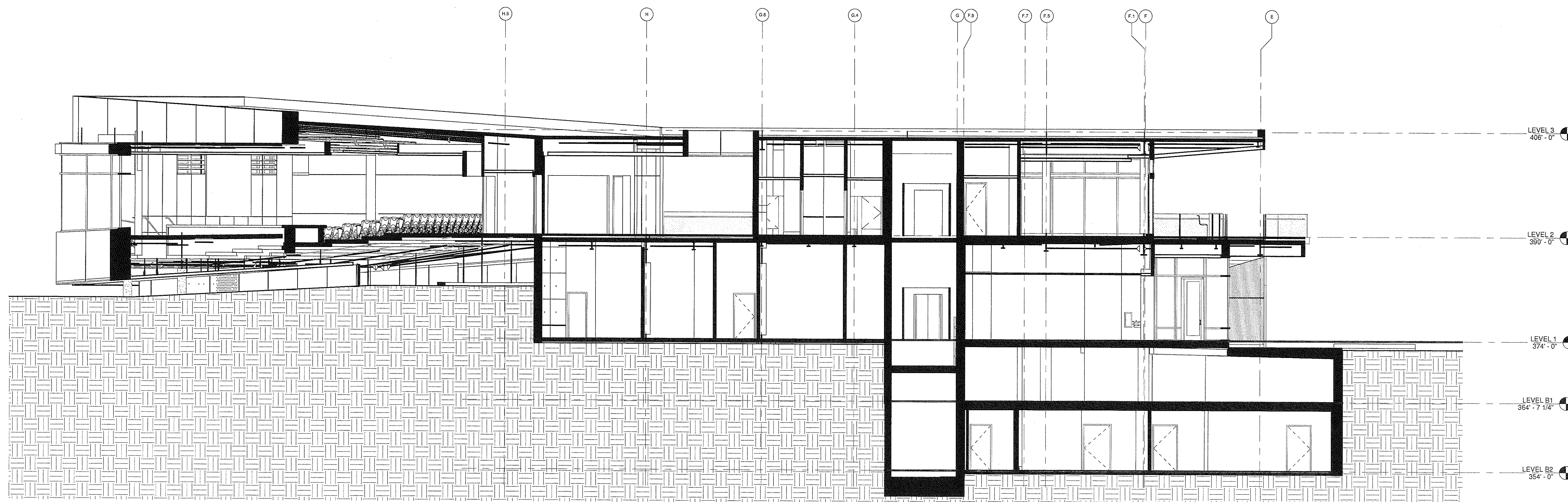
1 BUILDING SECTION A2110/A6102 1/8" = 1'-0"
