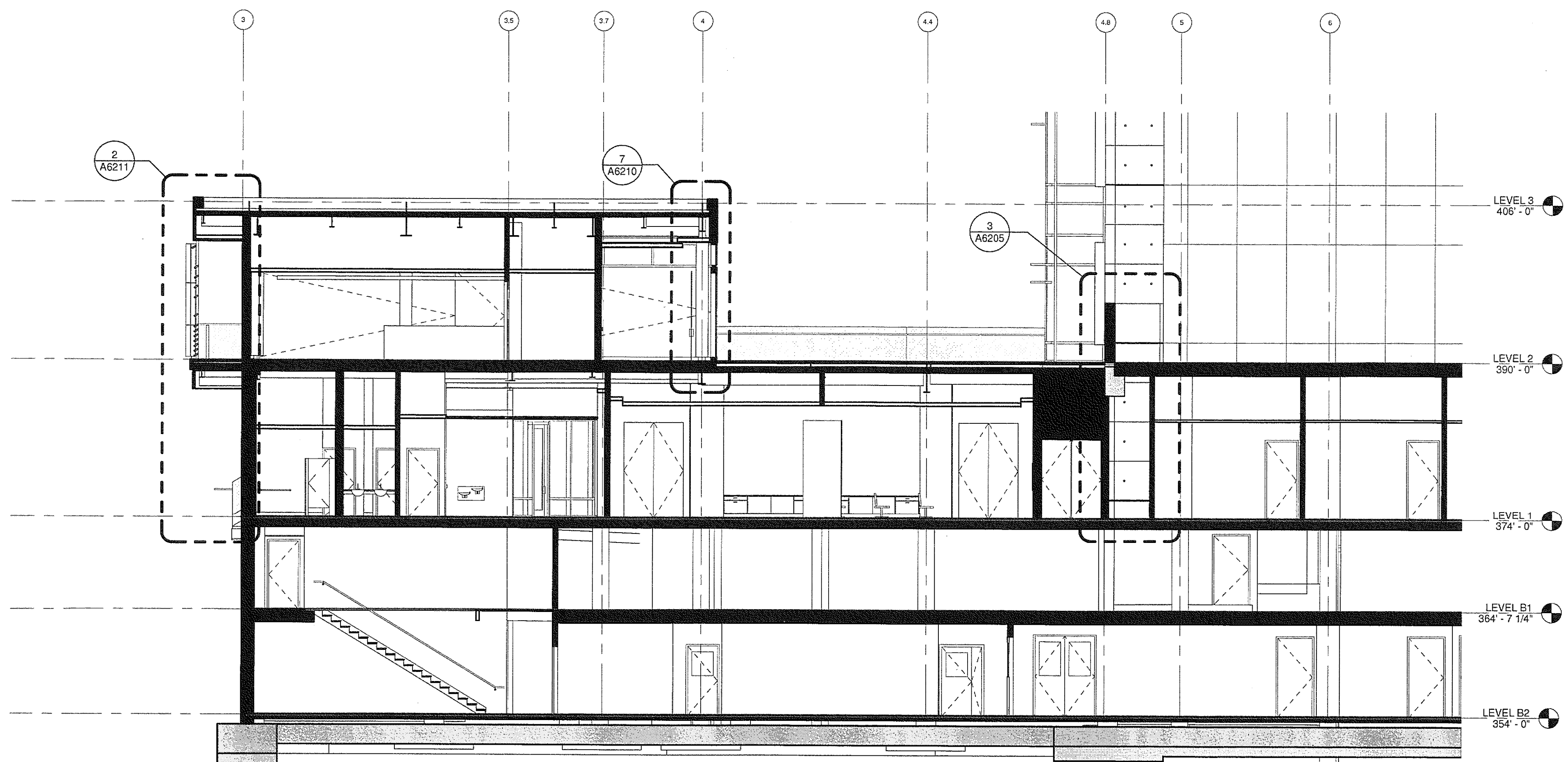
2 BUILDING SECTION A2120/A6102 1/8" = 1'-0"
