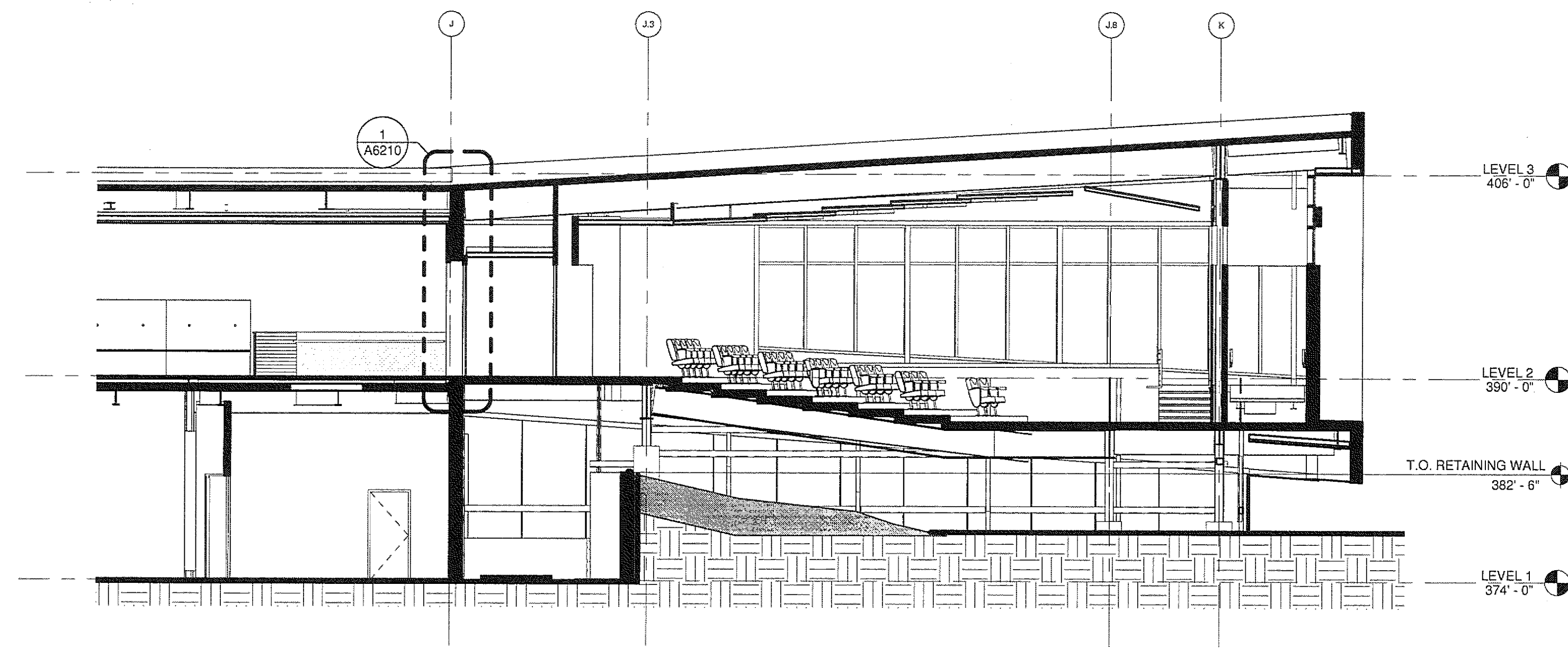
6 BUILDING SECTION A2110/A6102 1/8" = 1'-0"
