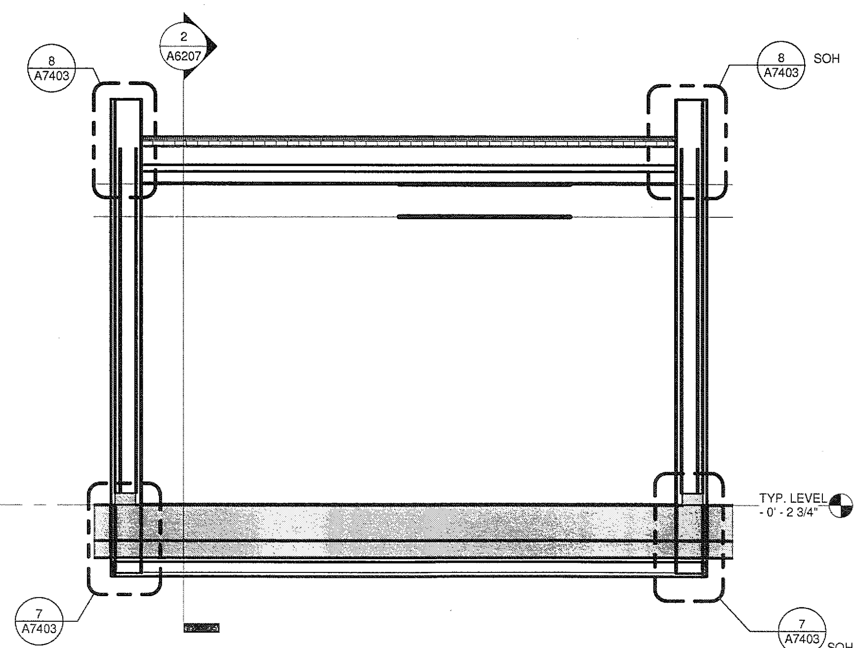
10 JUNIOR POD SECTION A2601 A6207 3/8" = 1'-0"
