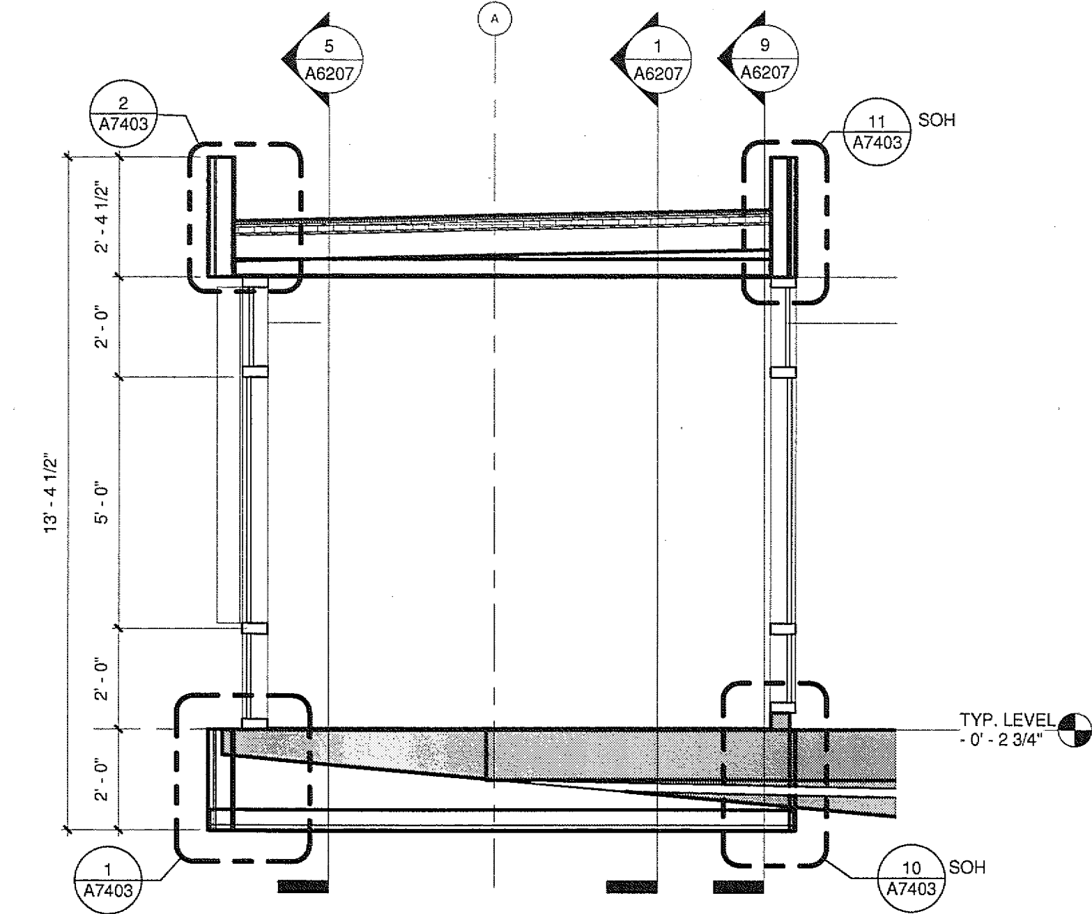
2 TYPICAL POD SECTION A2601 A6207 3/8" = 1'-0"
