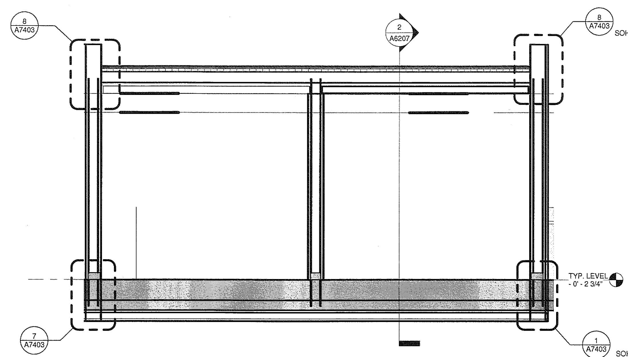
10 JUNIOR POD SECTION A2601 A6207 3/8" = 1'-0"
