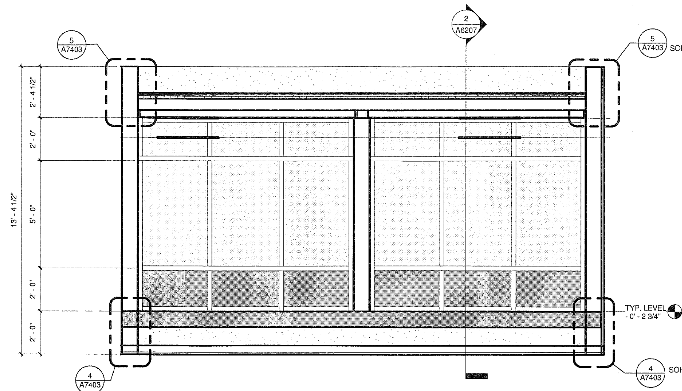
6 JUNIOR POD SECTION A2601 A6207 3/8" = 1'-0"
