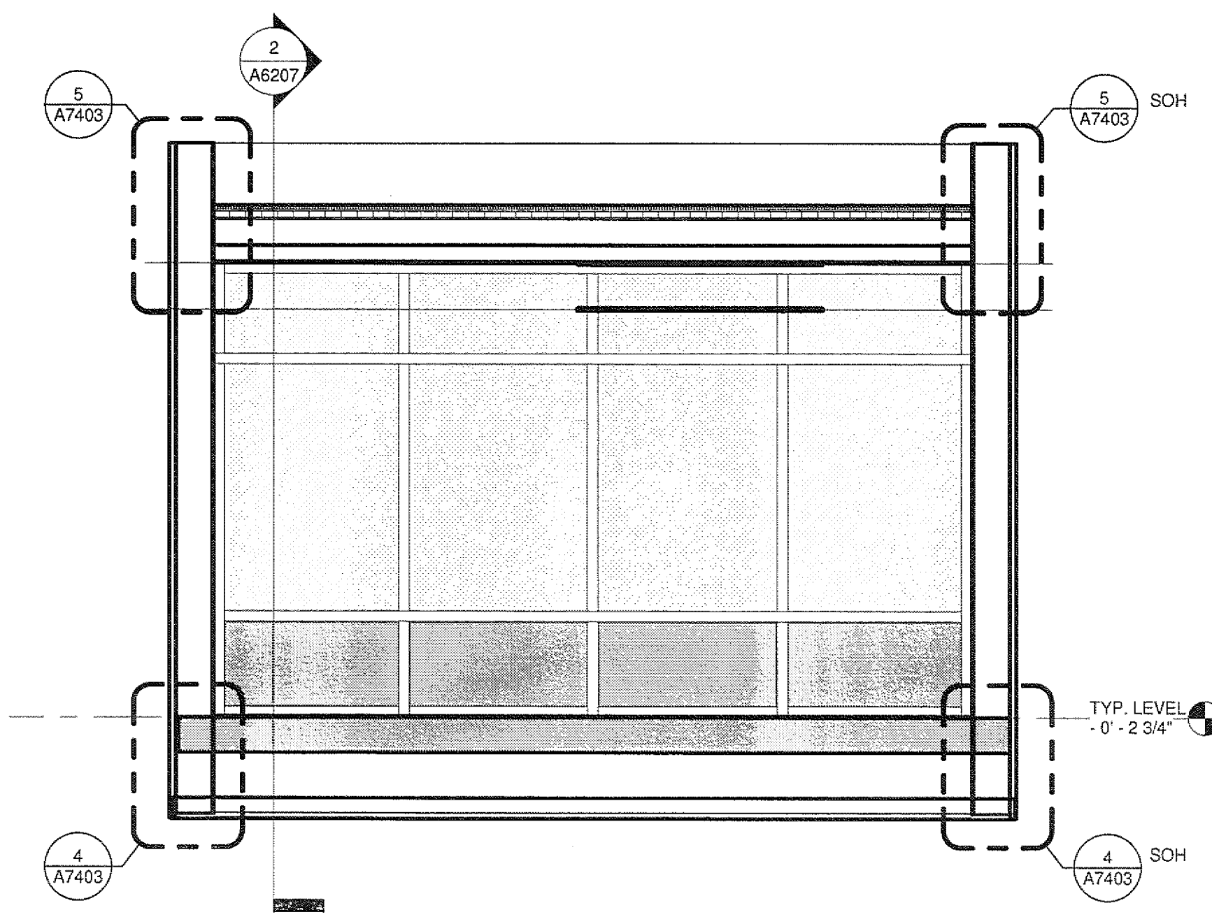
6 JUNIOR POD SECTION A2601 A6207 3/8" = 1'-0"
