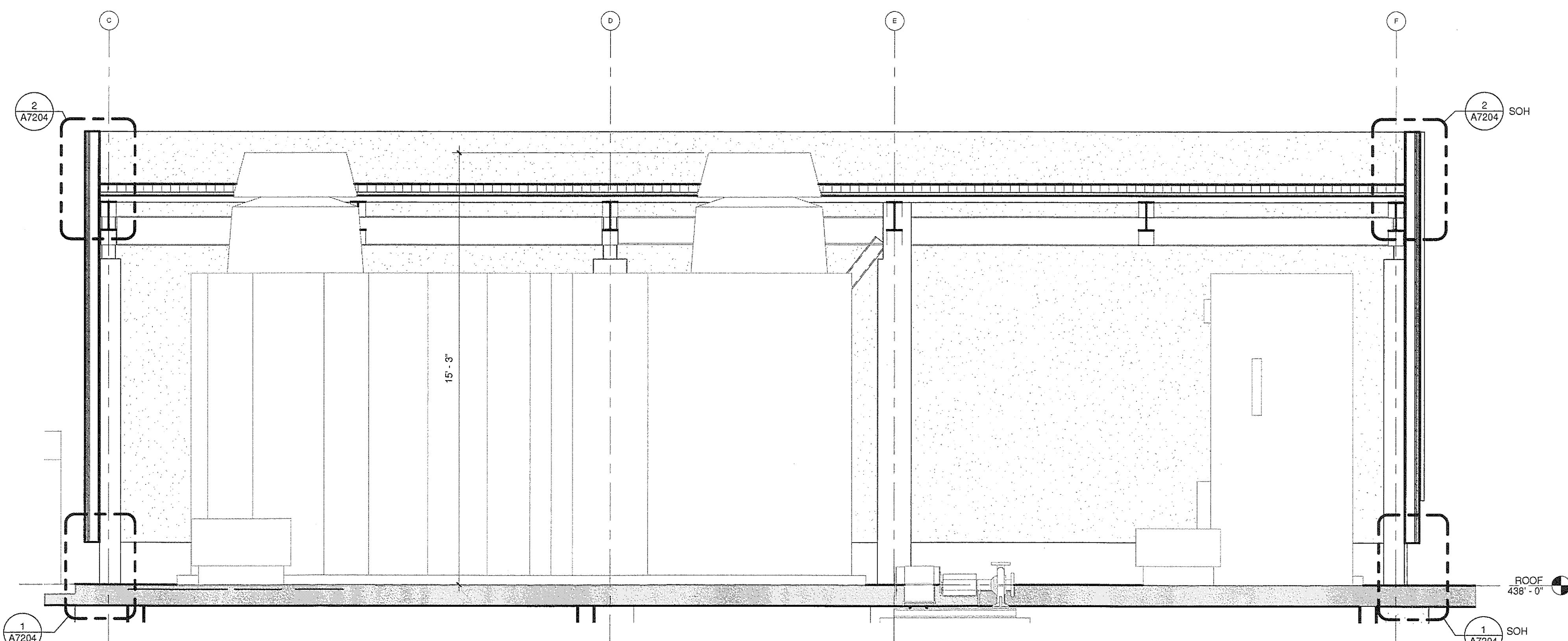
11 MECH PENTHOUSE SECTION A2251 A6207 3/8" = 1'-0"
