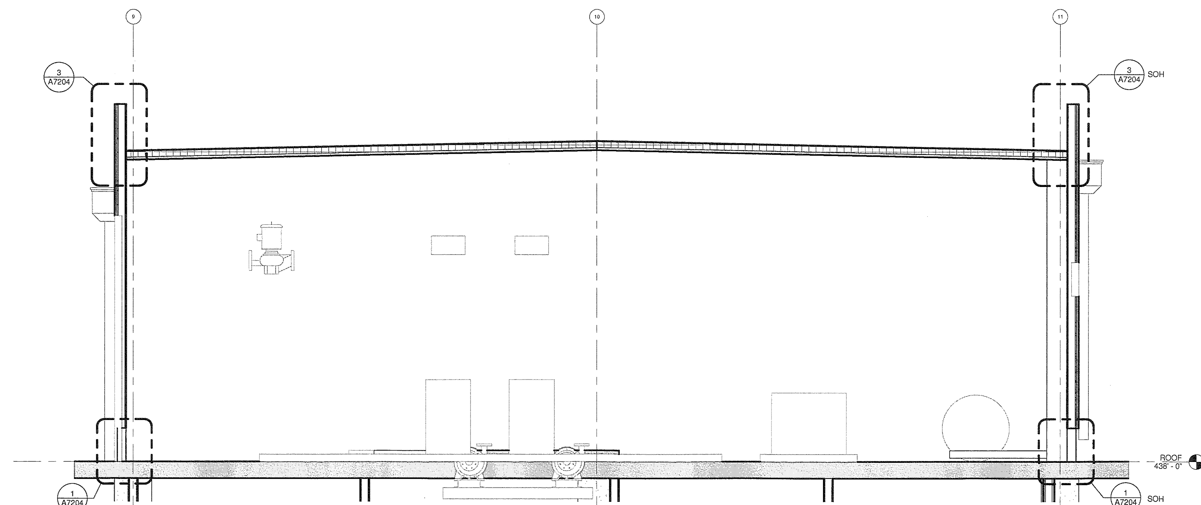
3 MECH PENTHOUSE SECTION A2251 A6207 3/8" = 1'-0"
