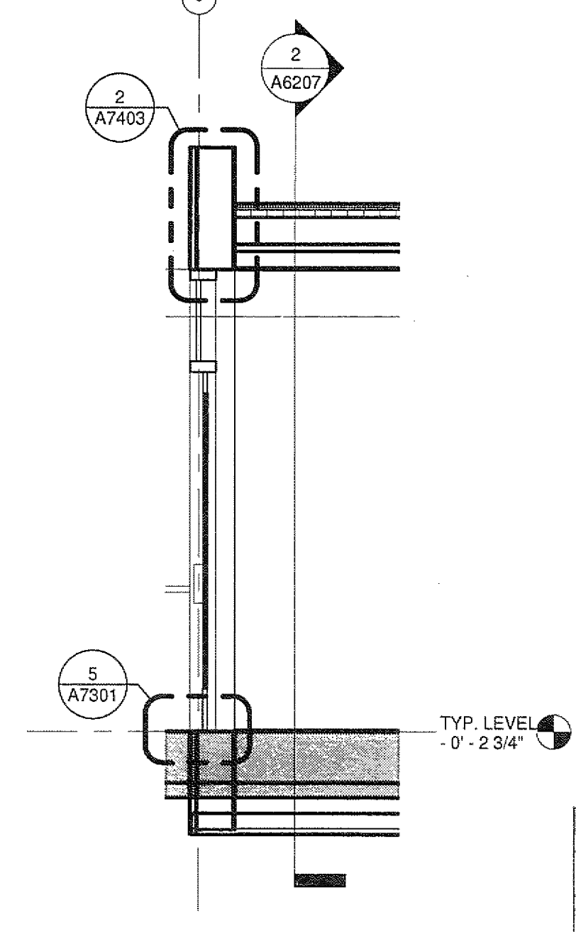
2 TYPICAL POD SECTION A2601 A6207 3/8" = 1'-0"
