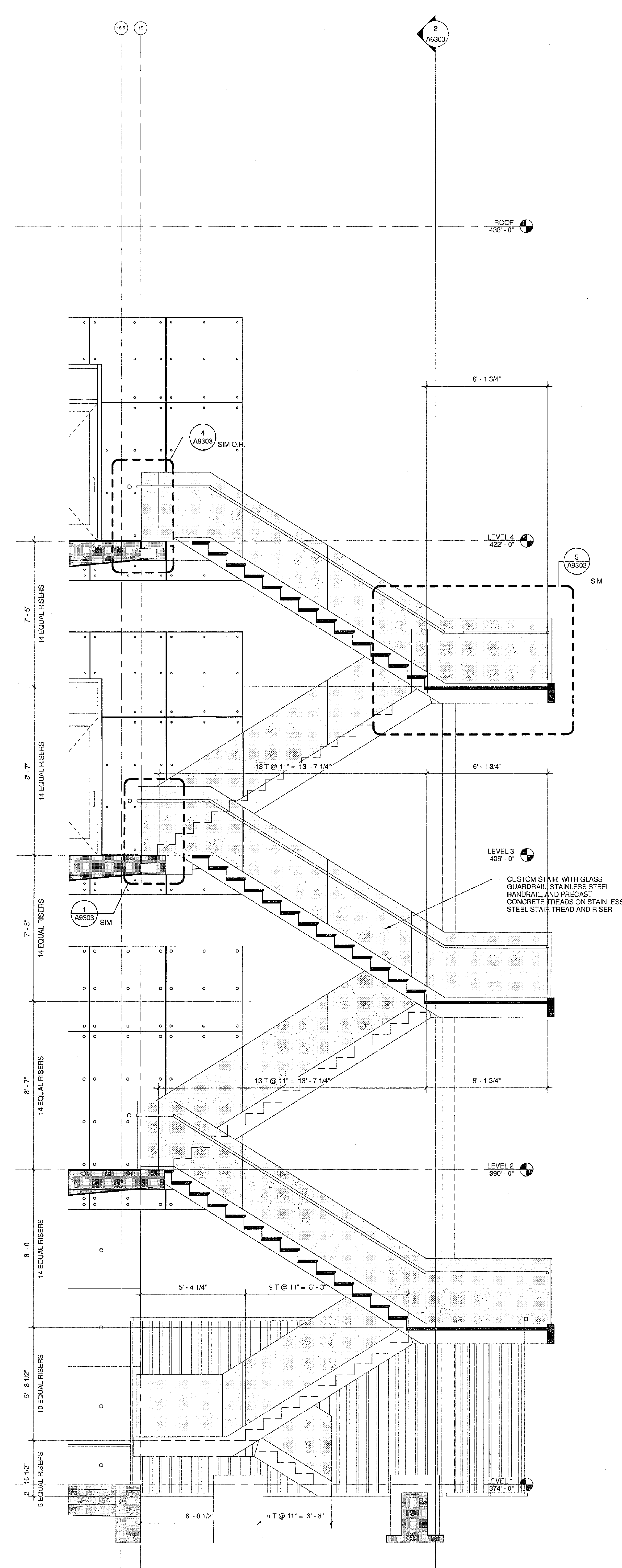
1 STAIR 1 WEST SECTION A212 | A6303 3/8" = 1'-0"
