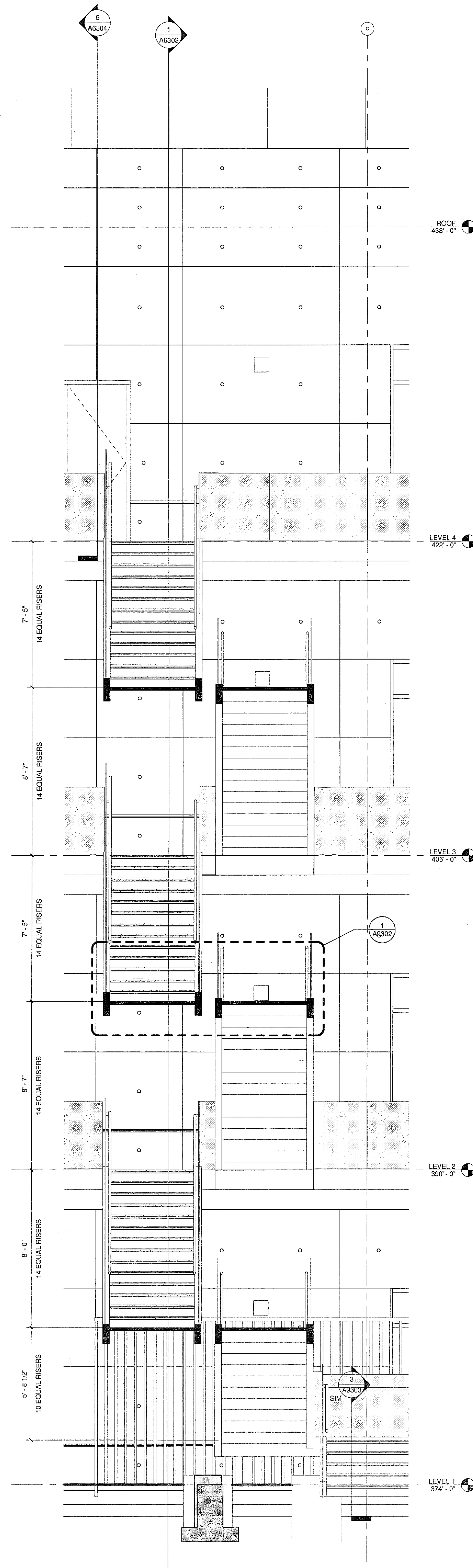
2 STAIR 1 SOUTH SECTION A212 | A6303 3/8" = 1'-0"
