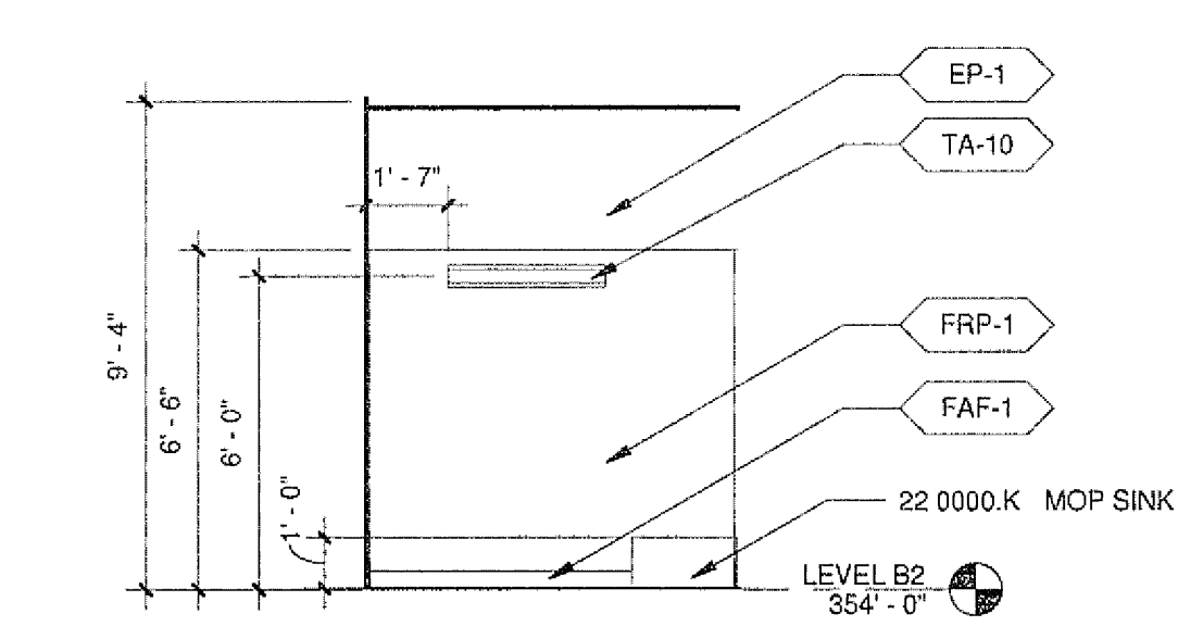
6 JANITOR CLOSET B301 - NORTH A22821 A8213 1/4" = 1'-0"
