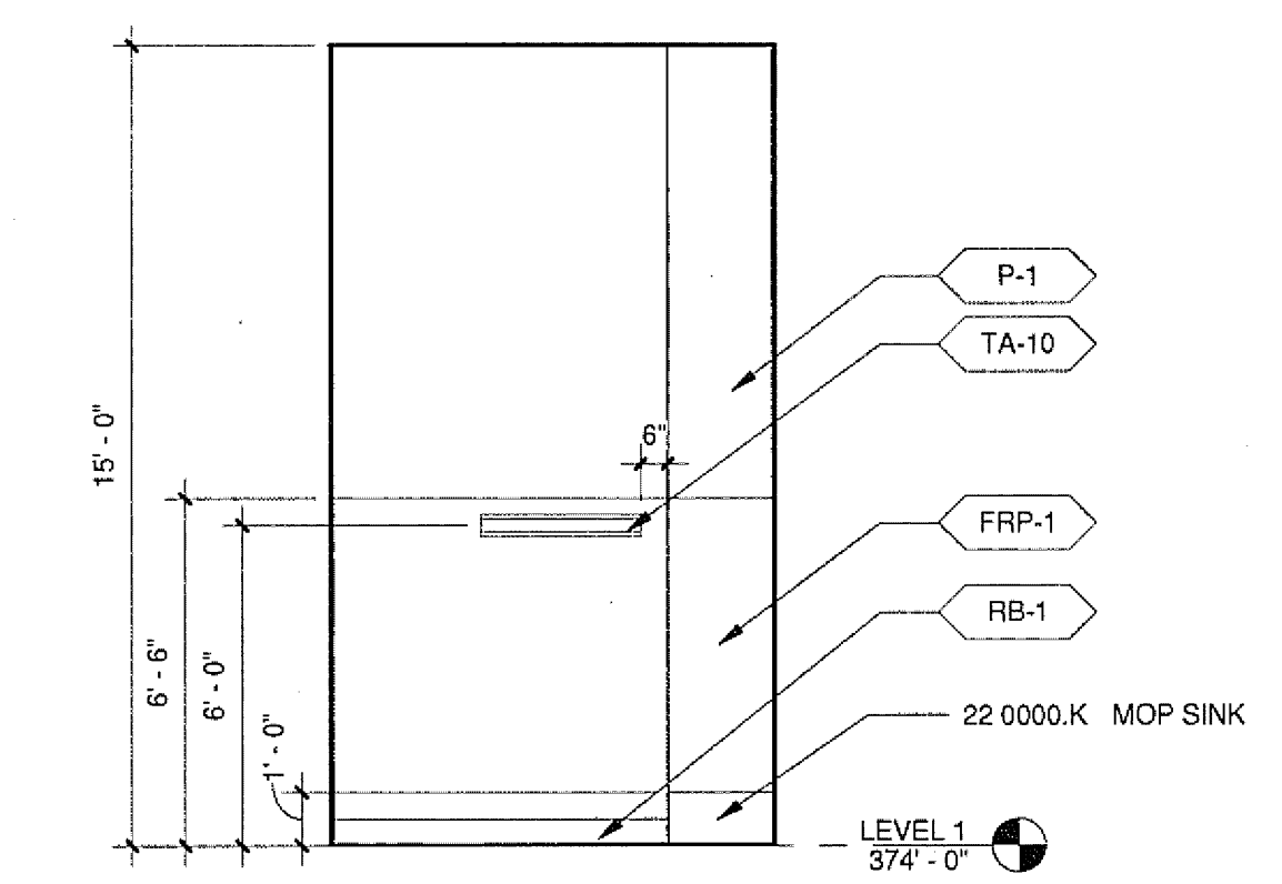
15 JANITOR CLOSET 1822 TYP. - SOUTH A2212 A8213 1/4" = 1'-0"
