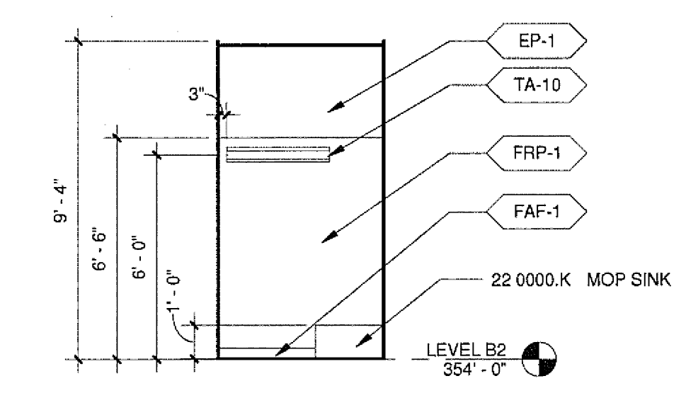
7 JANITOR CLOSET B510 - EAST A22821 A8213 1/4" = 1'-0"
