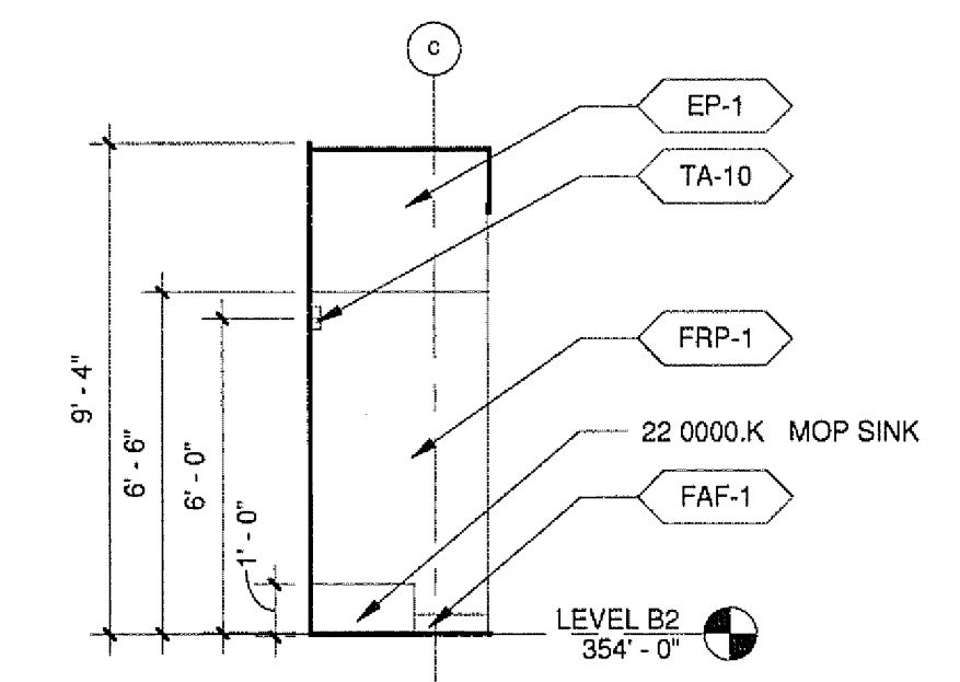
9 JANITOR CLOSET B510 - SOUTH A22821 A8213 1/4" = 1'-0"
