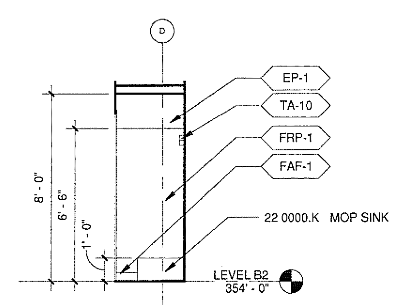
3 JANITOR CLOSET B004 - SOUTH A22821 A8213 1/4" = 1'-0"
