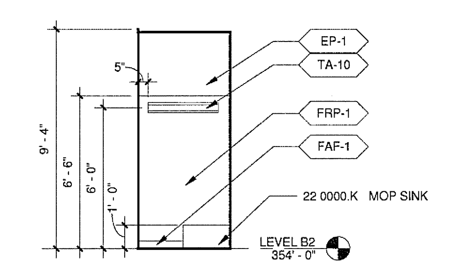
12 JANITOR CLOSET B710 - WEST A22821 A8213 1/4" = 1'-0"
