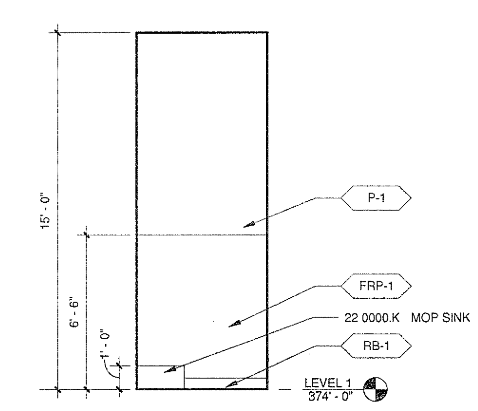
16 JANITOR CLOSET 1822 TYP. - WEST A2212 A8213 1/4" = 1'-0"
