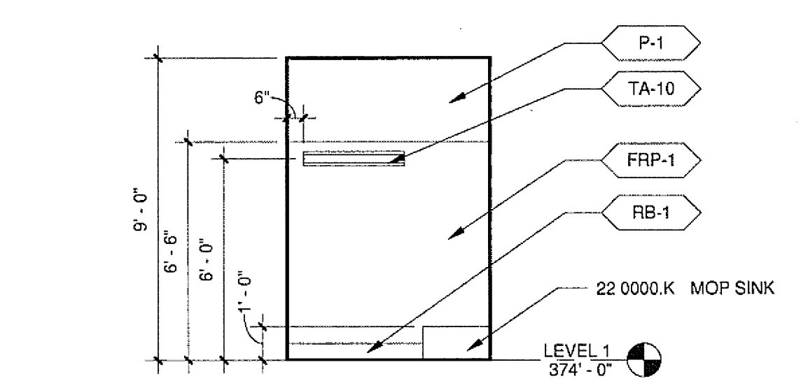
14 JANITOR CLOSET 1021 - WEST A2212 A8213 1/4" = 1'-0"
