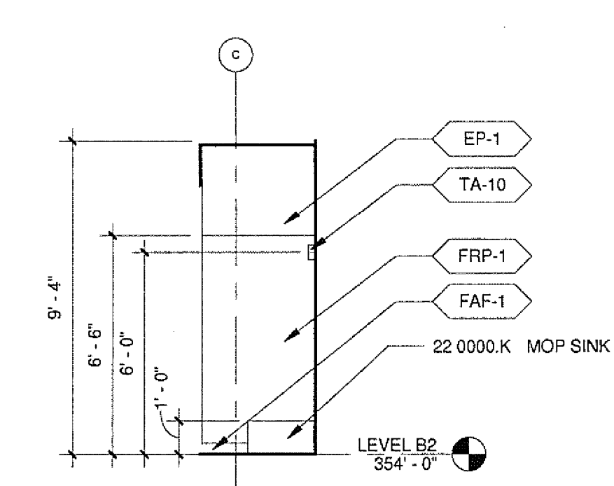
8 JANITOR CLOSET B510 - NORTH A22821 A8213 1/4" = 1'-0"
