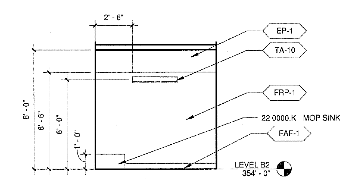
4 JANITOR CLOSET B004 - WEST A22821 A8213 1/4" = 1'-0"
