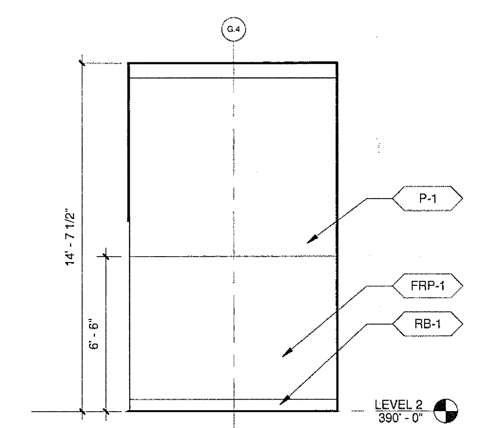
20 JANITOR CLOSET 2017 - NORTH A2702 A8213 1/4" = 1'-0"
