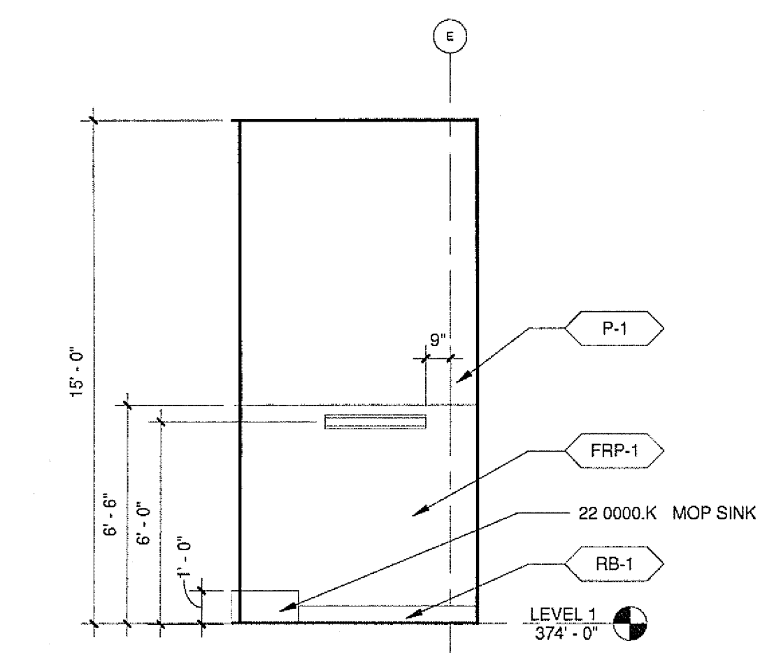
18 JANITOR CLOSET 1823 TYP. - SOUTH A2212 A8213 1/4" = 1'-0"
