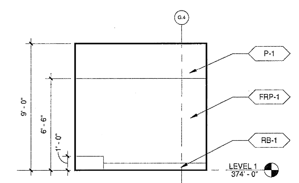
13 JANITOR CLOSET 1021 - NORTH A2212 A8213 1/4" = 1'-0"
