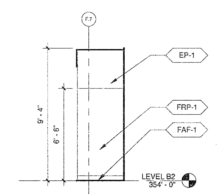
11 JANITOR CLOSET B710 - SOUTH A22821 A8213 1/4" = 1'-0"
