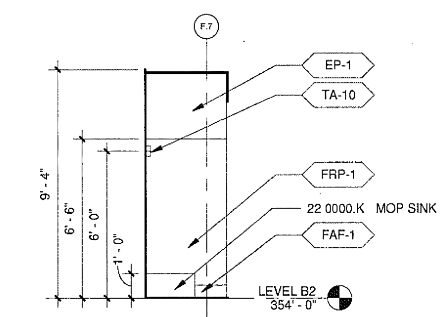
10 JANITOR CLOSET B710 - NORTH A22821 A8213 1/4" = 1'-0"
