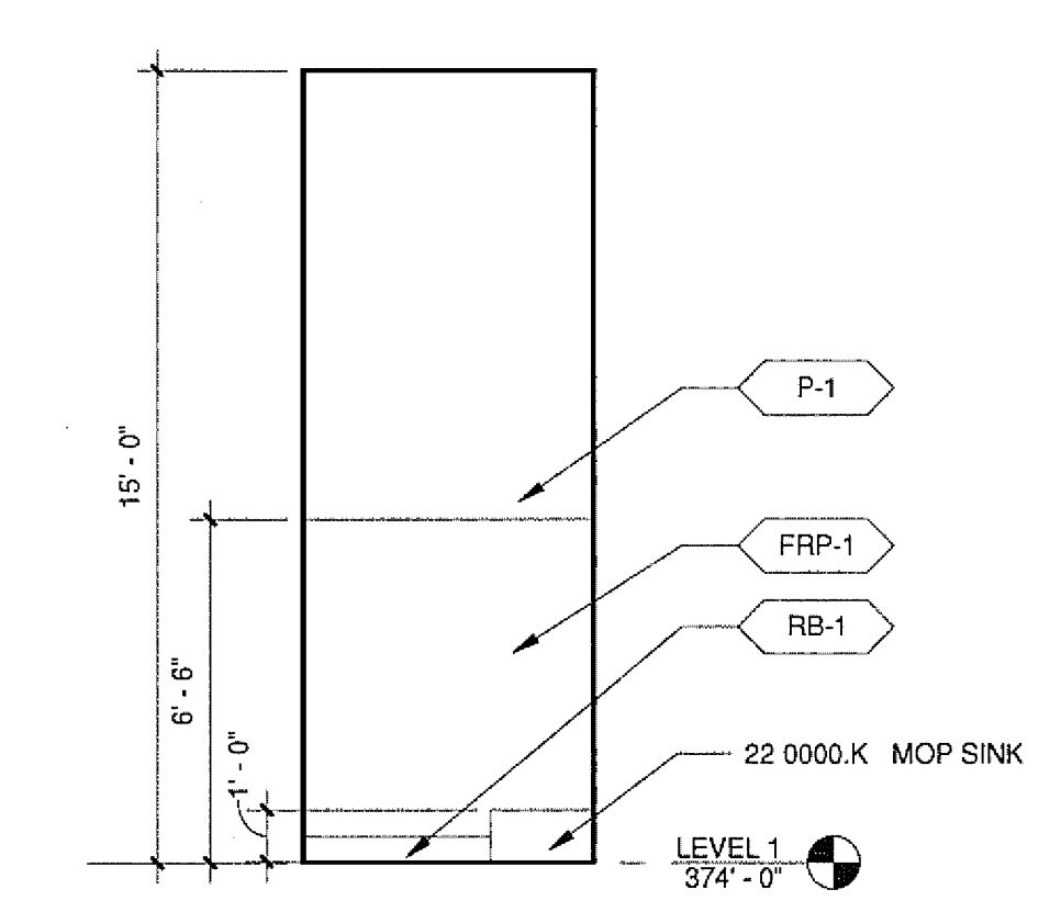
17 JANITOR CLOSET 1823 TYP. - EAST A2212 A8213 1/4" = 1'-0"
