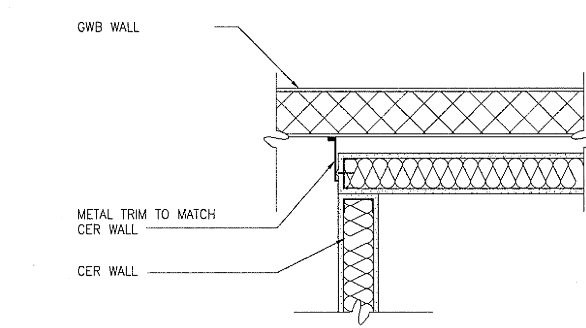
3 METAL TRIM AT CER TO GWB WALL
