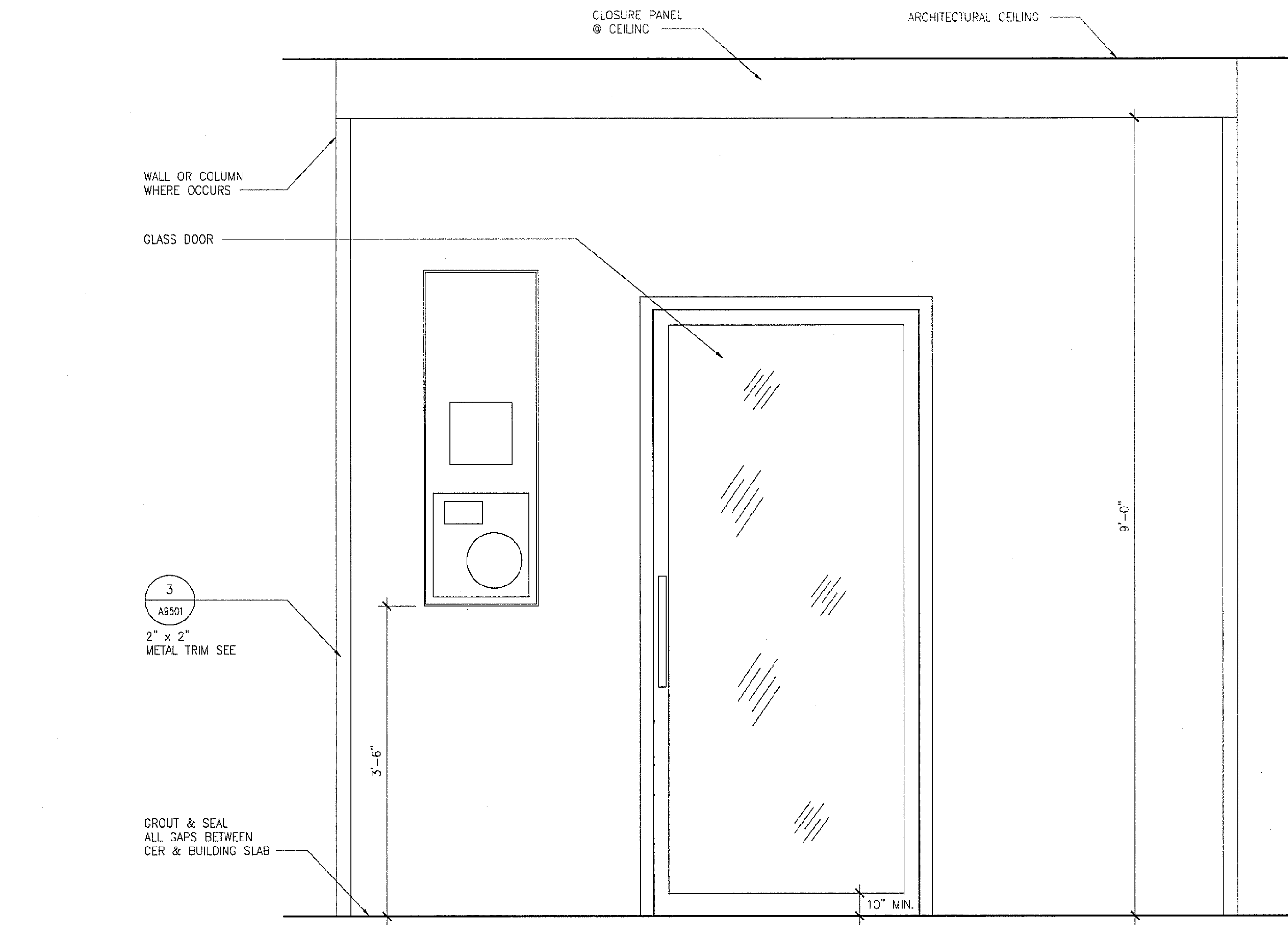
1 CONTROLLED ENVIRONMENTAL ROOM ELEVATION
