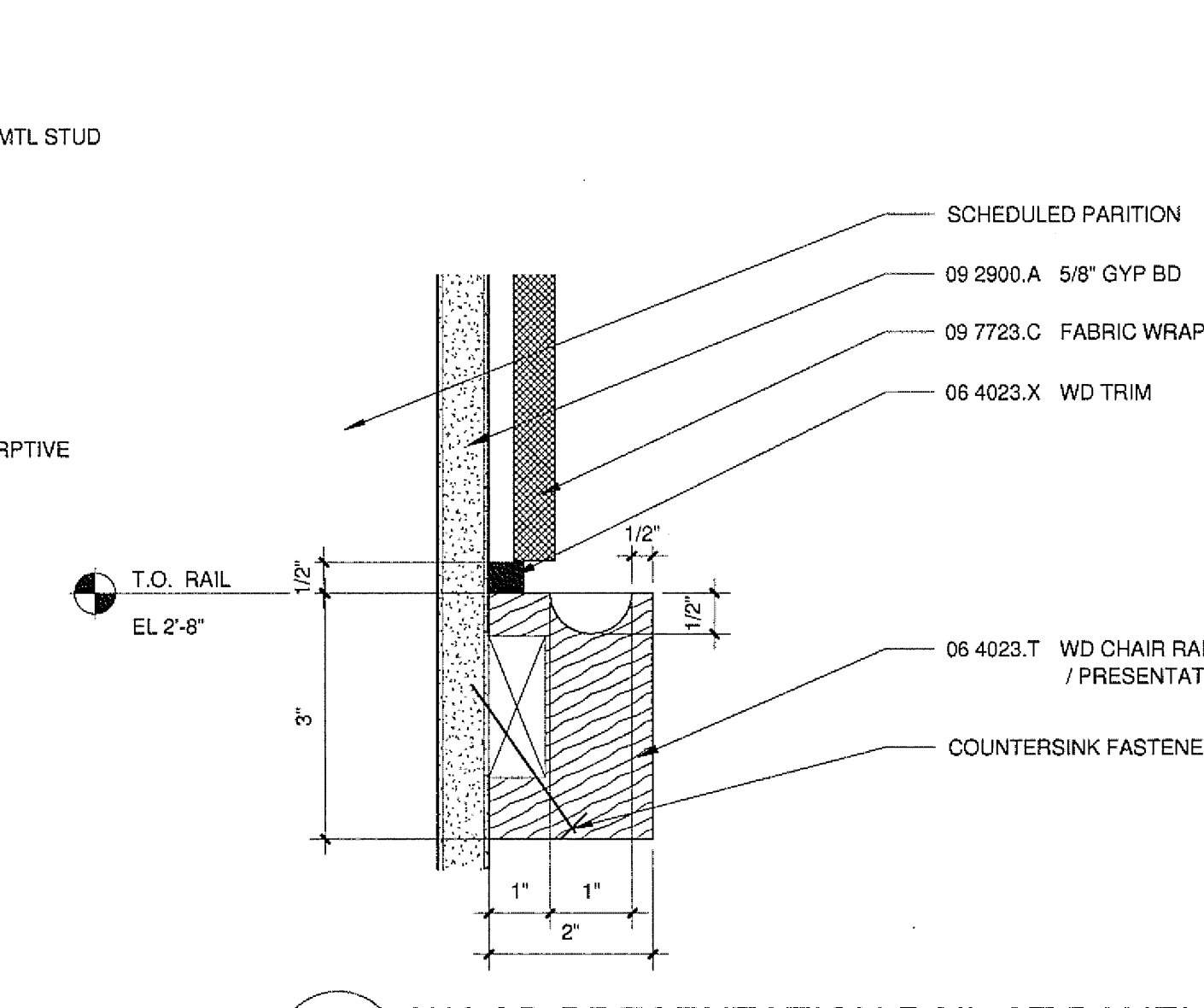
9 WOOD PRESENTATION RAIL AT PANEL A9601/A9704 6\"/>
