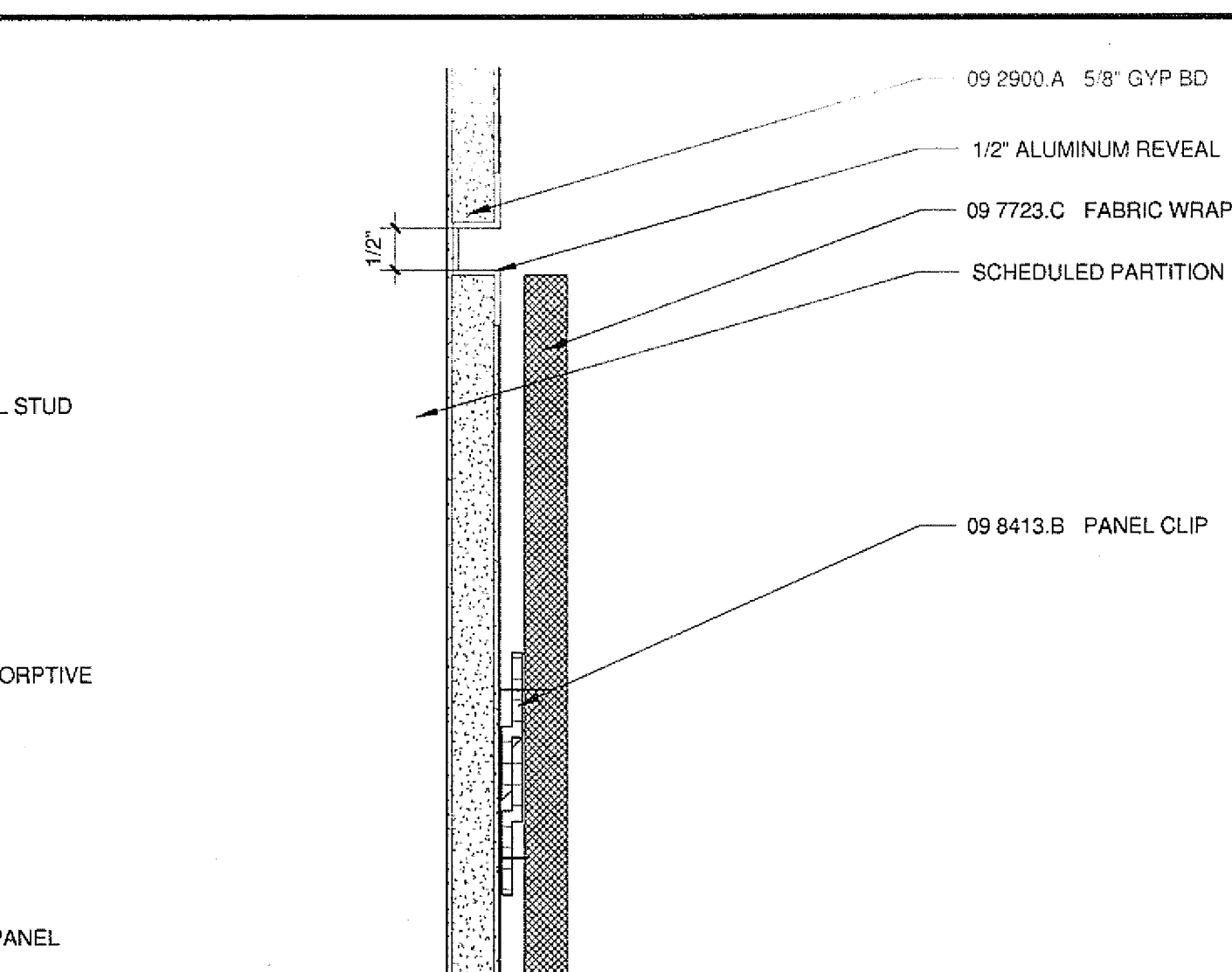
10 TACKABLE PANEL REVEAL DETAIL A9601/A9704 6\"/>
