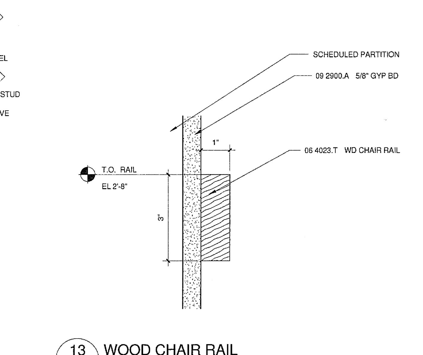
13 WOOD CHAIR RAIL A9601/A9704 6\"/>
