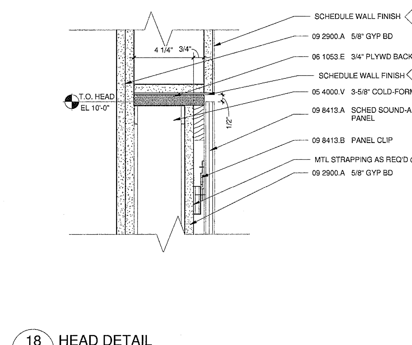
18 HEAD DETAIL A9601/A9704 3\"/>
