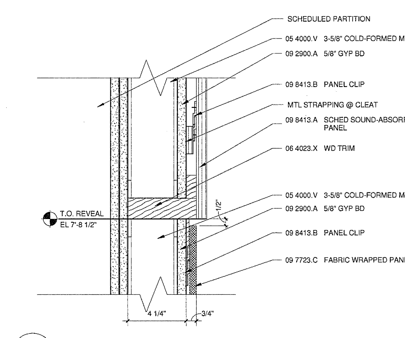
19 TACKABLE PANEL HEAD DETAIL A9601/A9704 3\"/>
