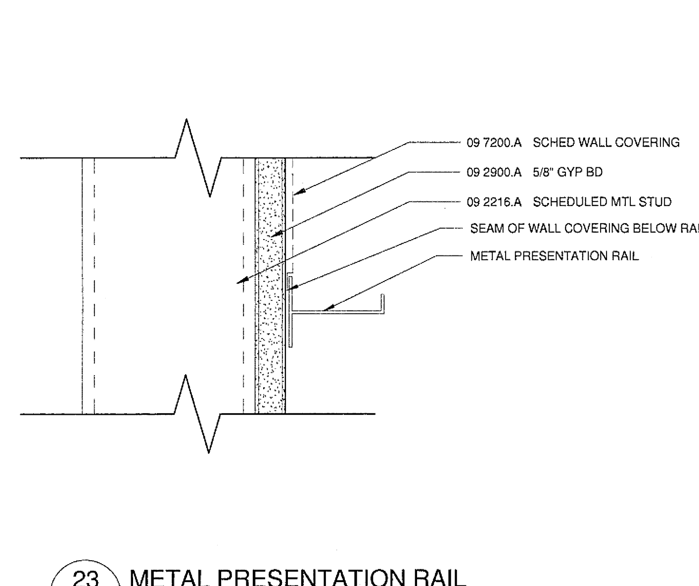
23 METAL PRESENTATION RAIL A9602/A9704 6\"/>
