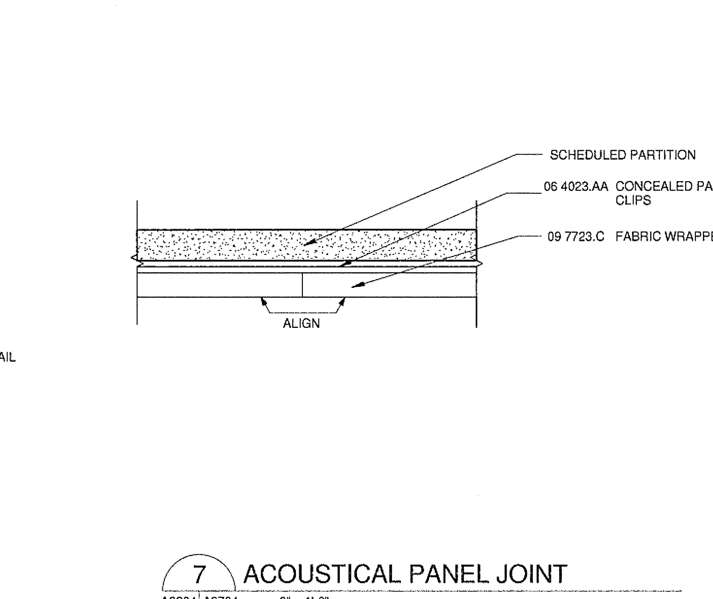
7 ACOUSTICAL PANEL JOINT A9204/A9704 6\"/>
