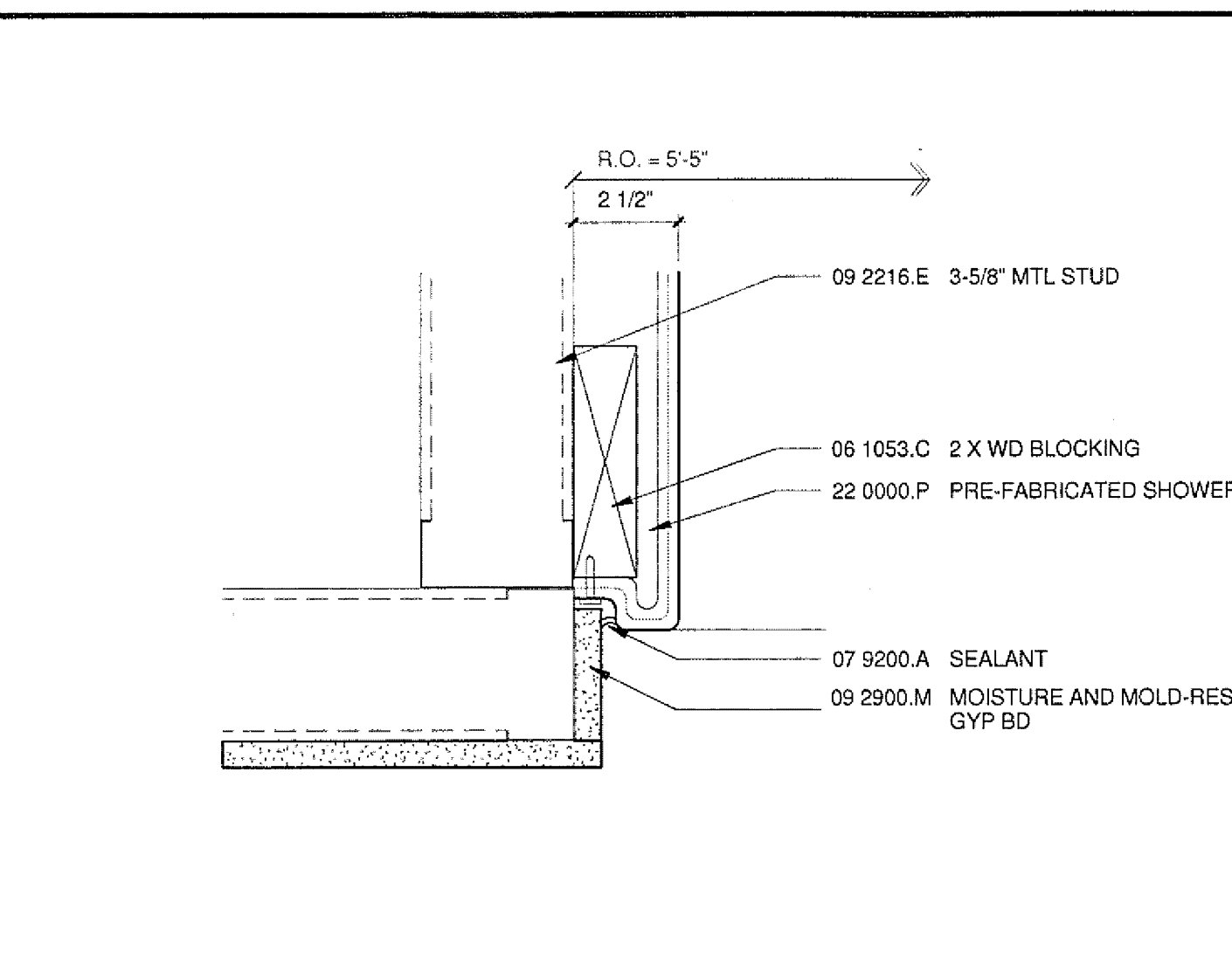
5 SHOWER CURB 1 A9701/A9704 3\"/>
