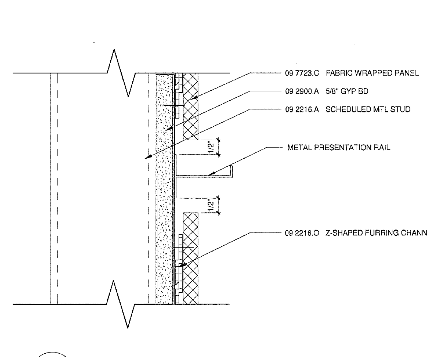
24 METAL PRESENTATION RAIL @ AWP A9602/A9704 6\"/>
