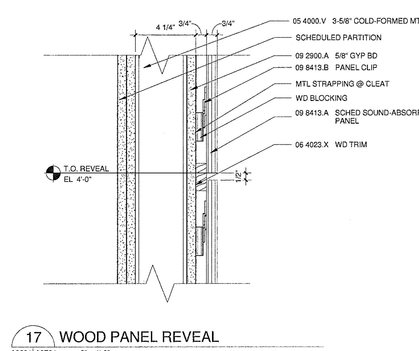
17 WOOD PANEL REVEAL A9601/A9704 3\"/>
