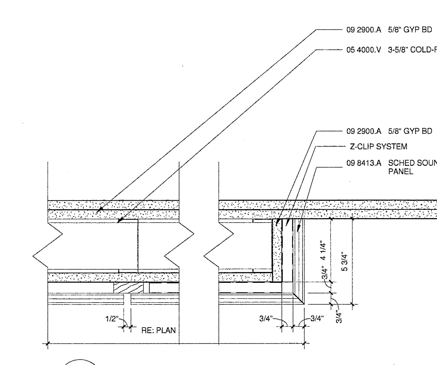
14 SIDE PLAN DETAIL A9704 3\"/>
