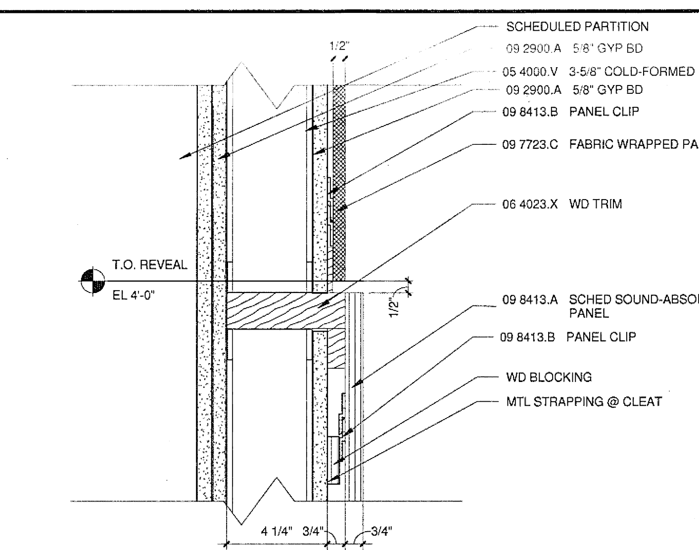
20 TACKABLE PANEL SILL DETAIL A9601/A9704 3\"/>
