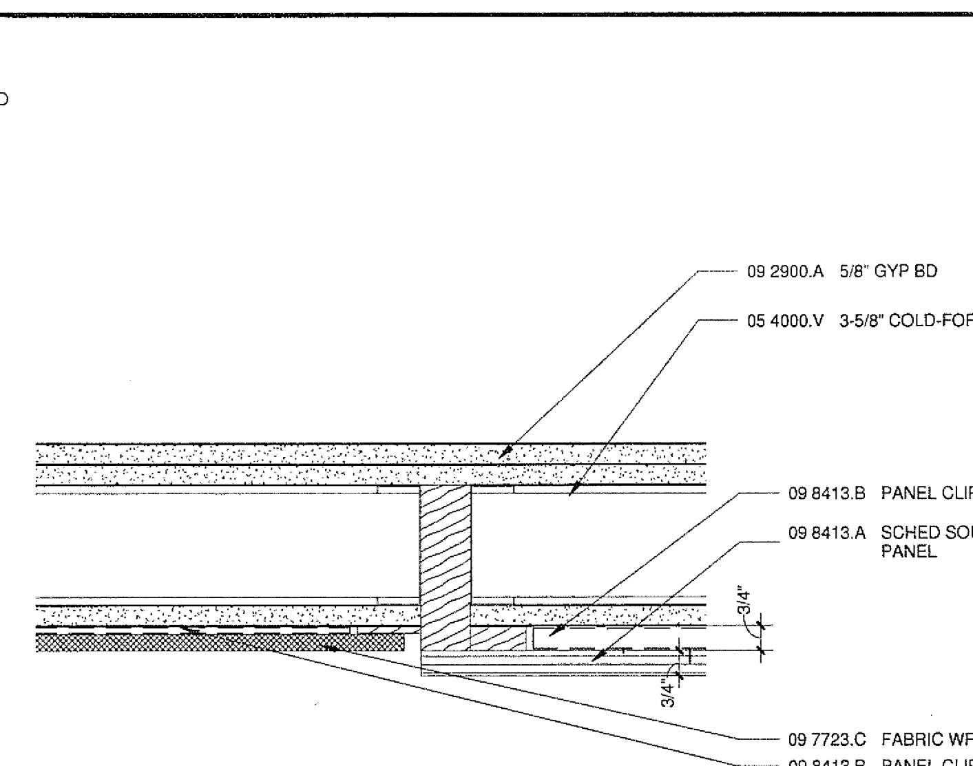
15 TACKABLE PANEL PLAN DETAIL A9204/A9704 3\"/>
