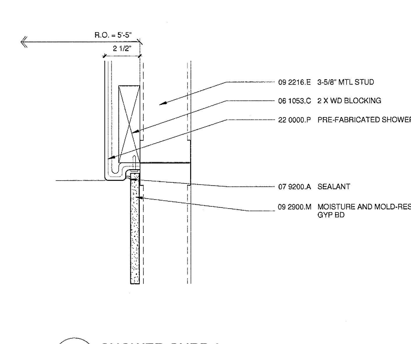
4 SHOWER CURB 2 A9701/A9704 3\"/>
