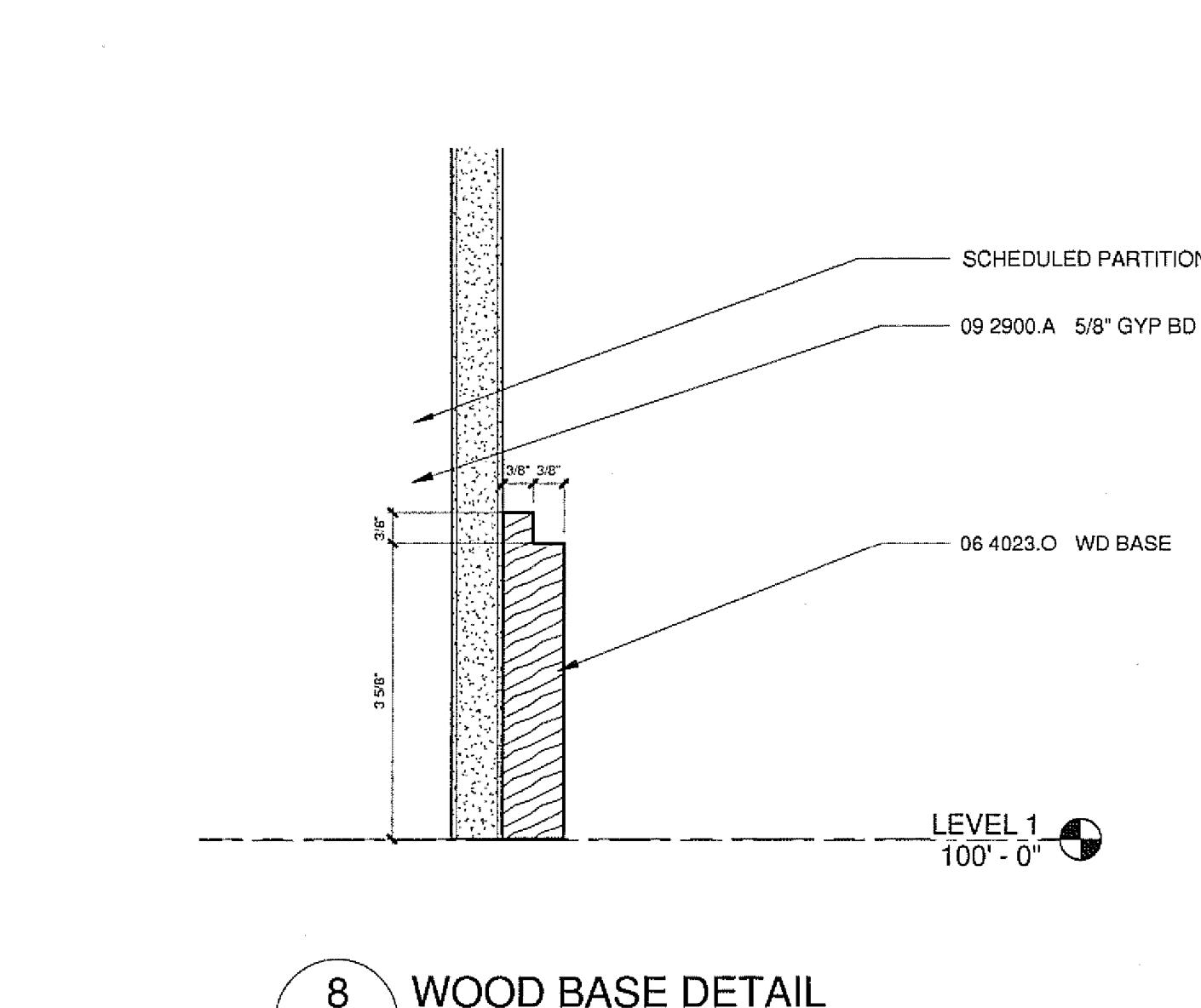
8 WOOD BASE DETAIL A9601/A9704 6\"/>
