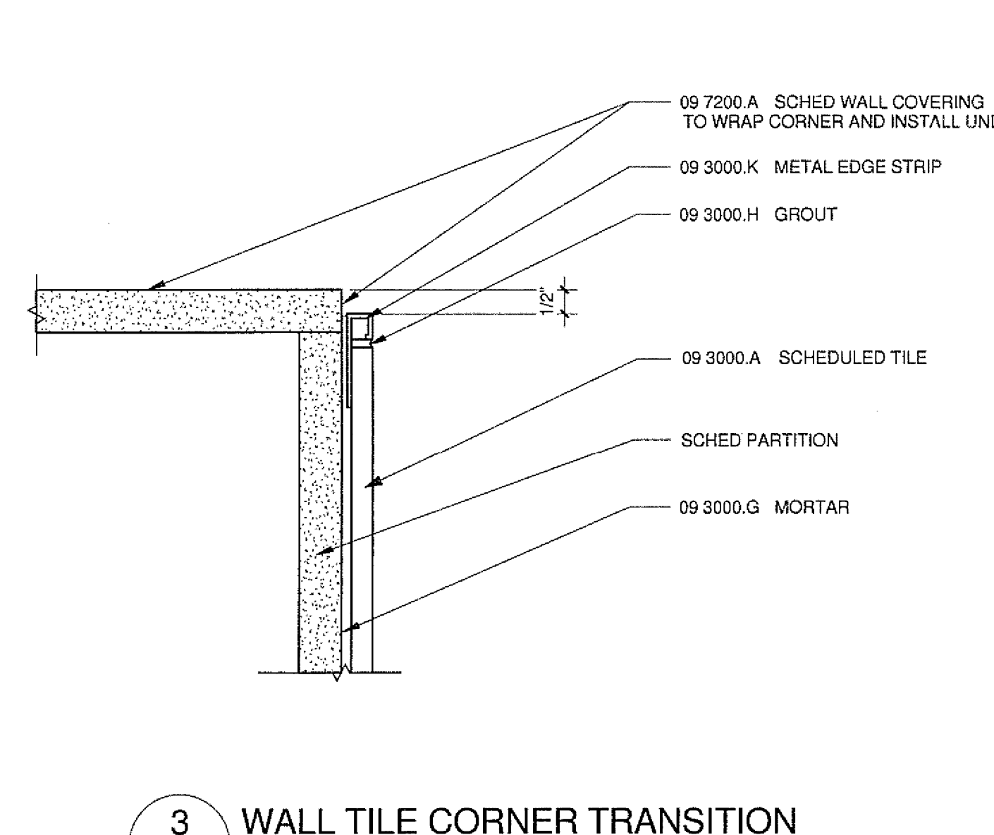
3 WALL TILE CORNER TRANSITION A9701/A9704 6\"/>
