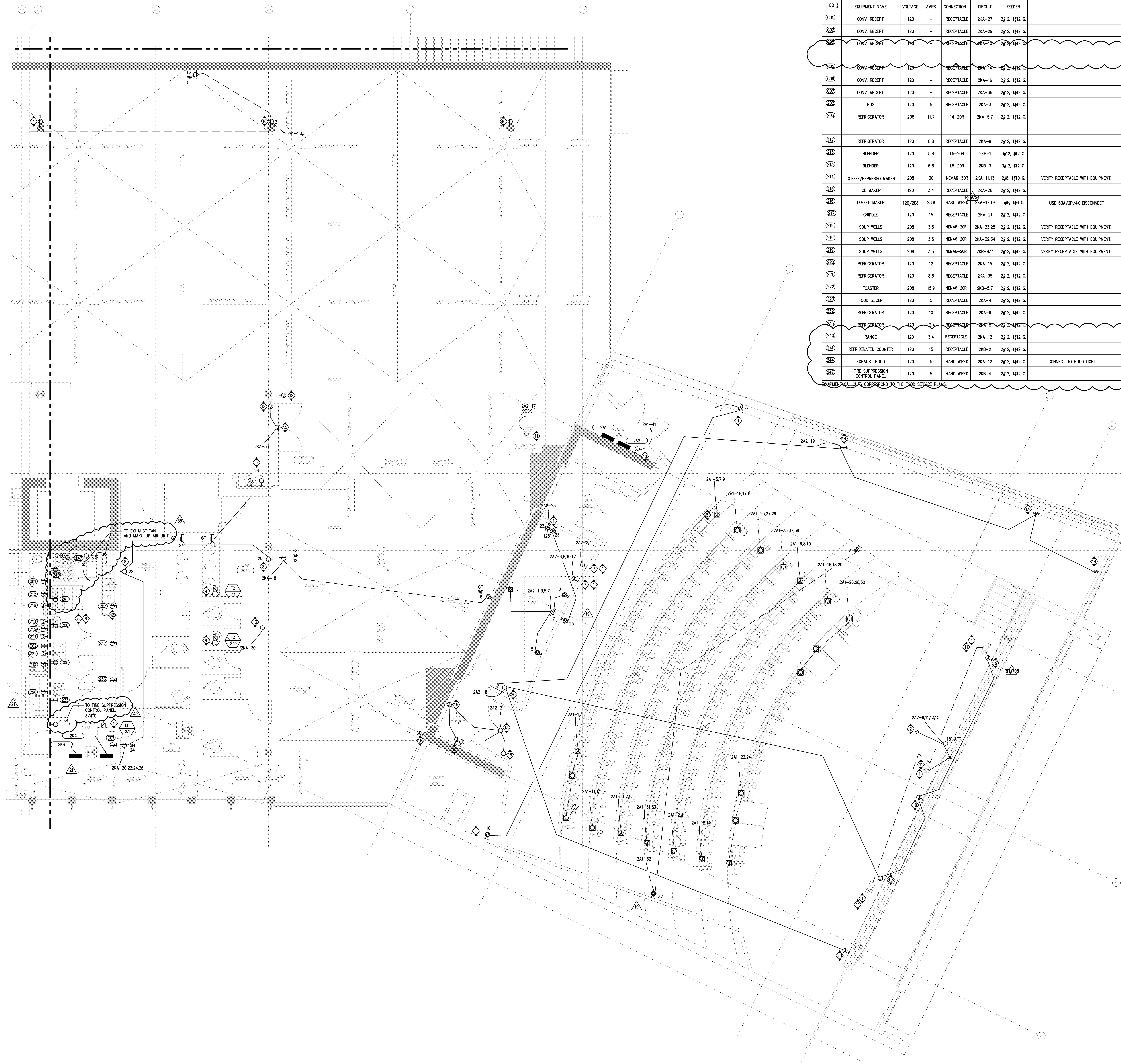
PARTIAL POWER SECOND FLOOR PLAN - ZONE 4
