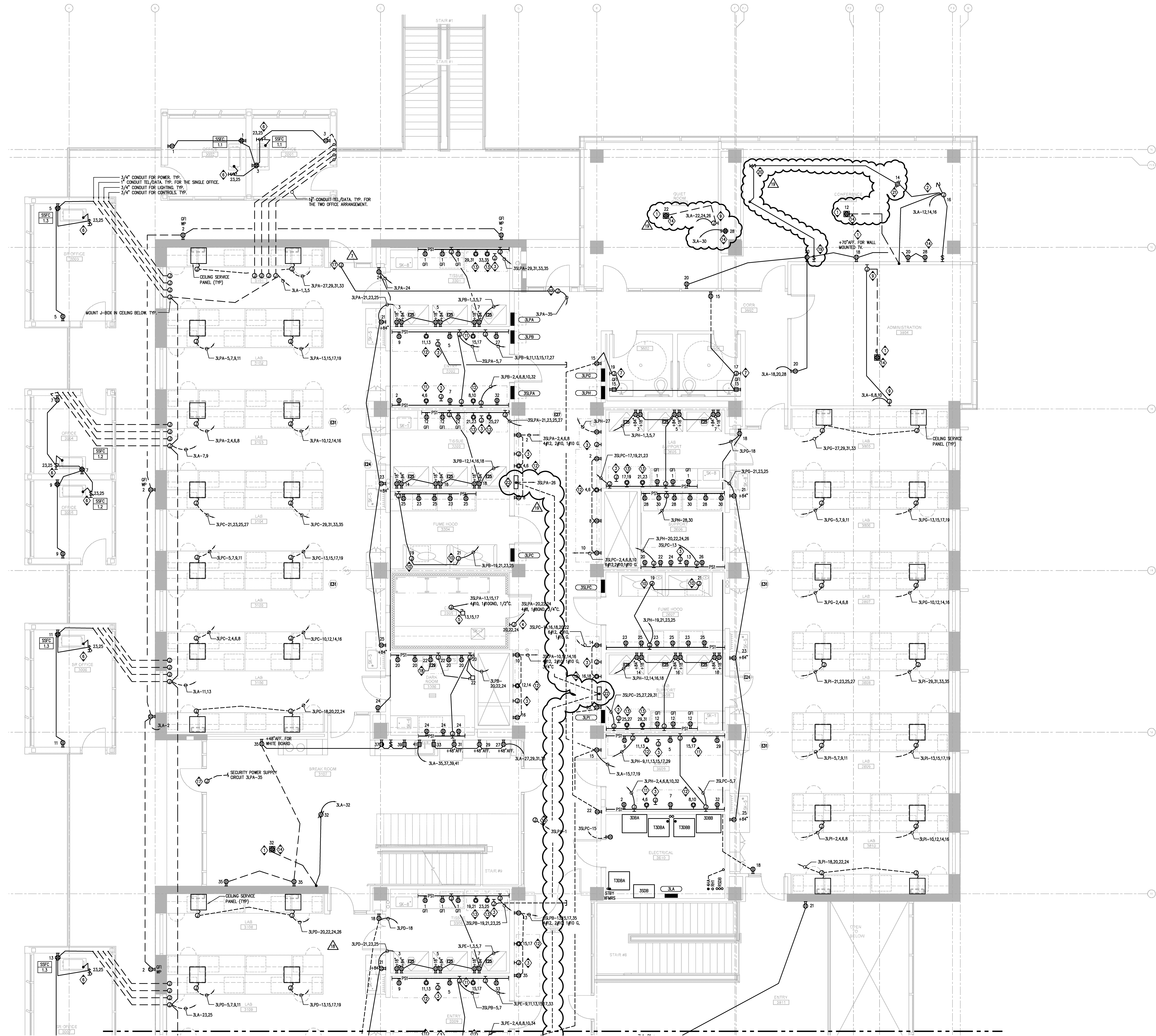
PARTIAL POWER THIRD FLOOR PLAN - ZONE 1
