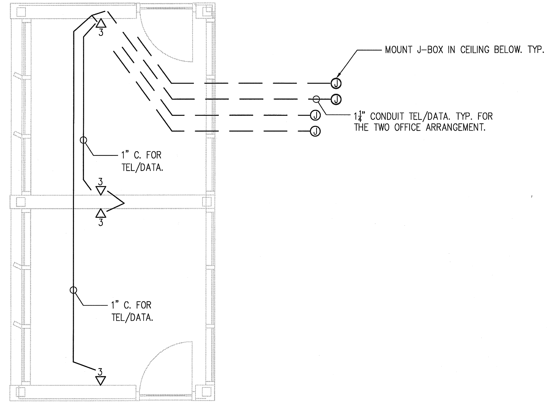
TEL/DATA TYPICAL FOR THE ONE OFFICE ARRANGEMENT
