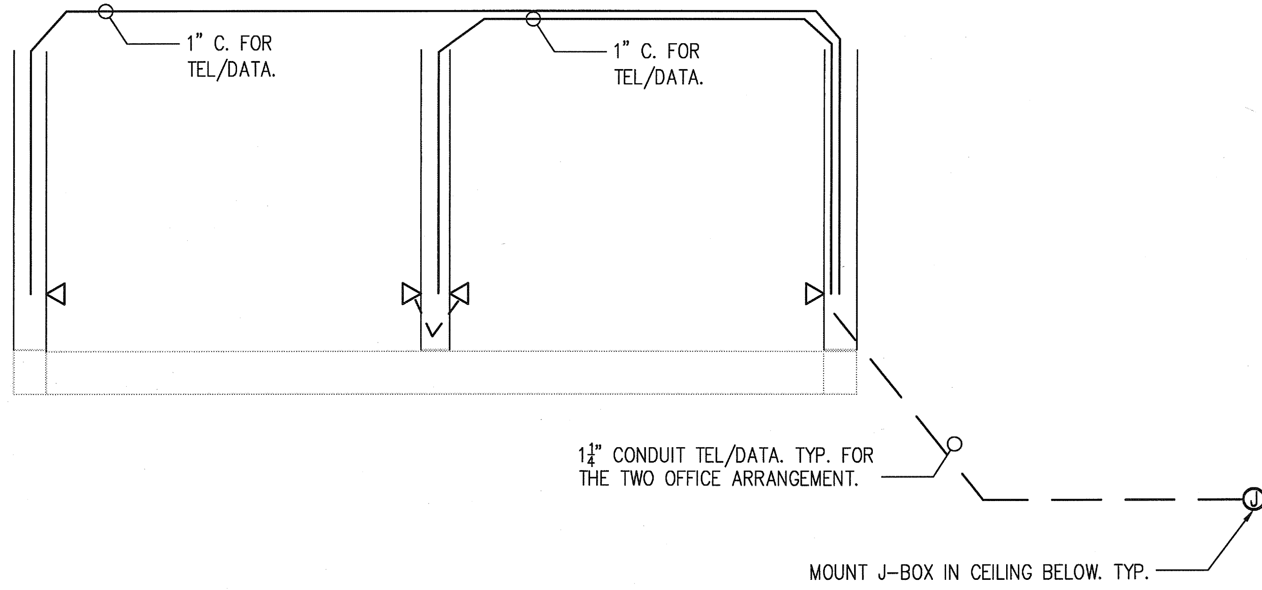
TEL/DATA TYPICAL FOR THE ONE OFFICE ARRANGEMENT
