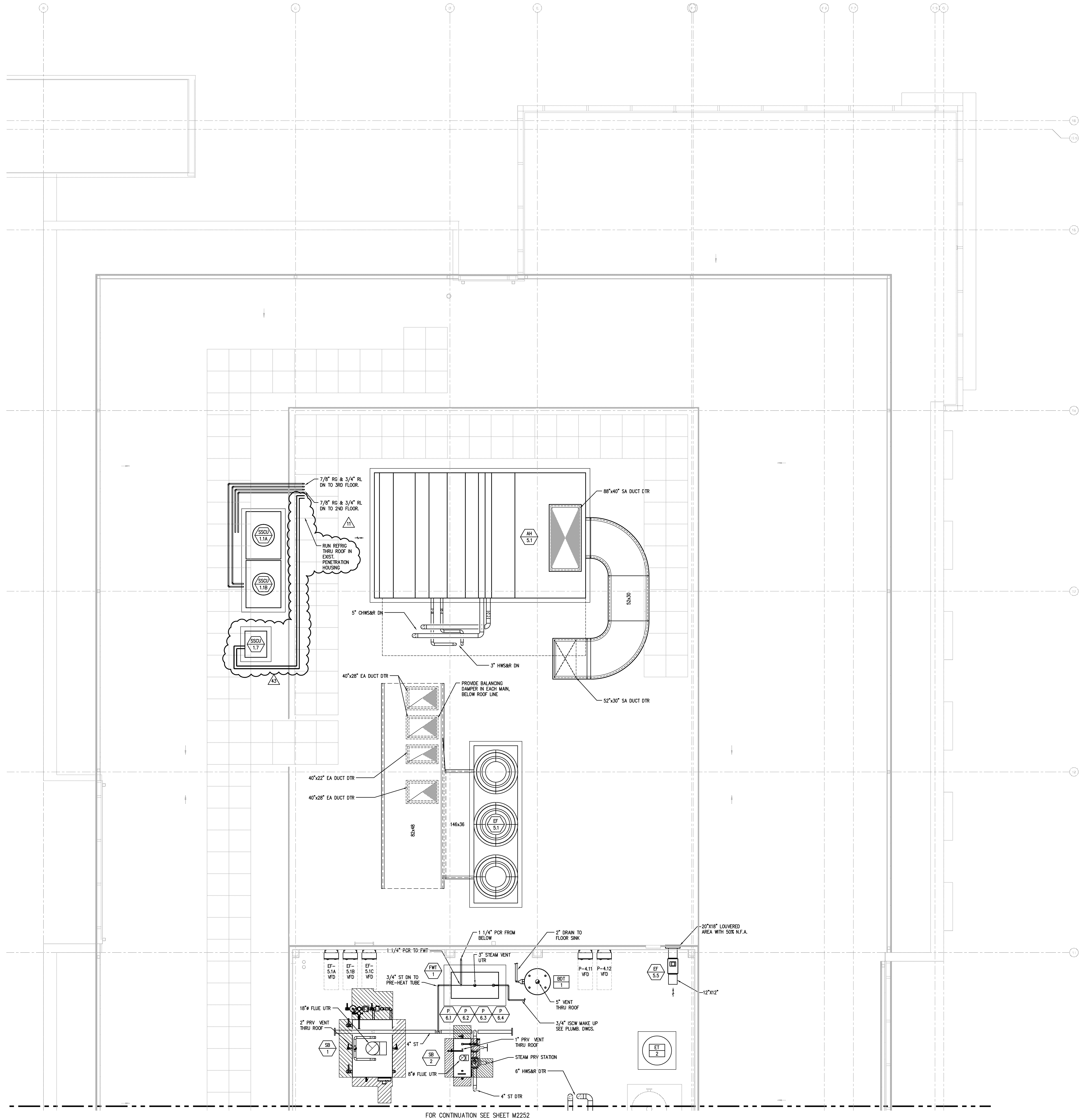
FOR CONTINUATION SEE SHEET M2252 PARTIAL MECHANICAL ROOF PLAN - ZONE 1
