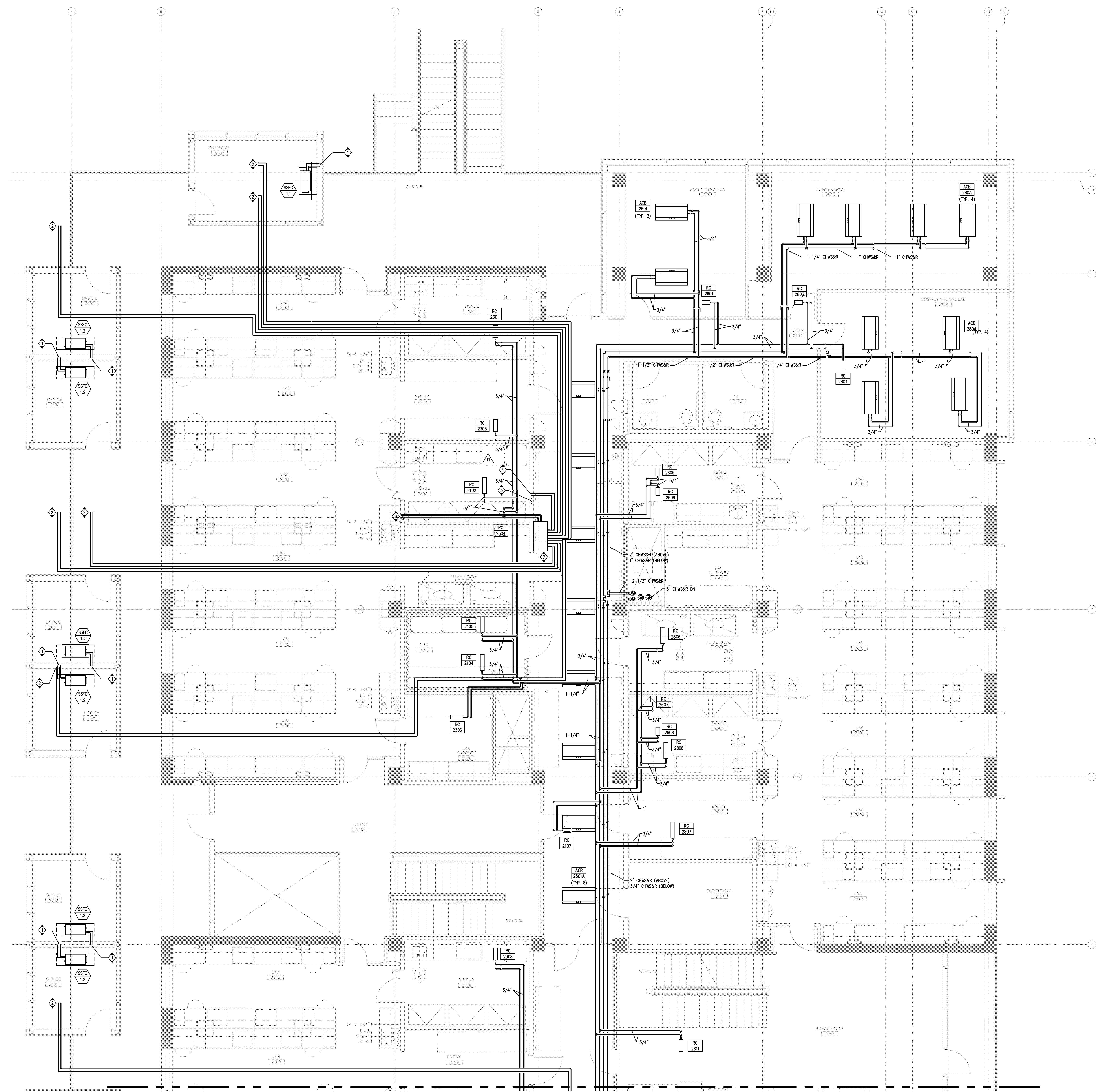
PARTIAL MECHANICAL PIPING SECOND FLOOR PLAN - ZONE 1
