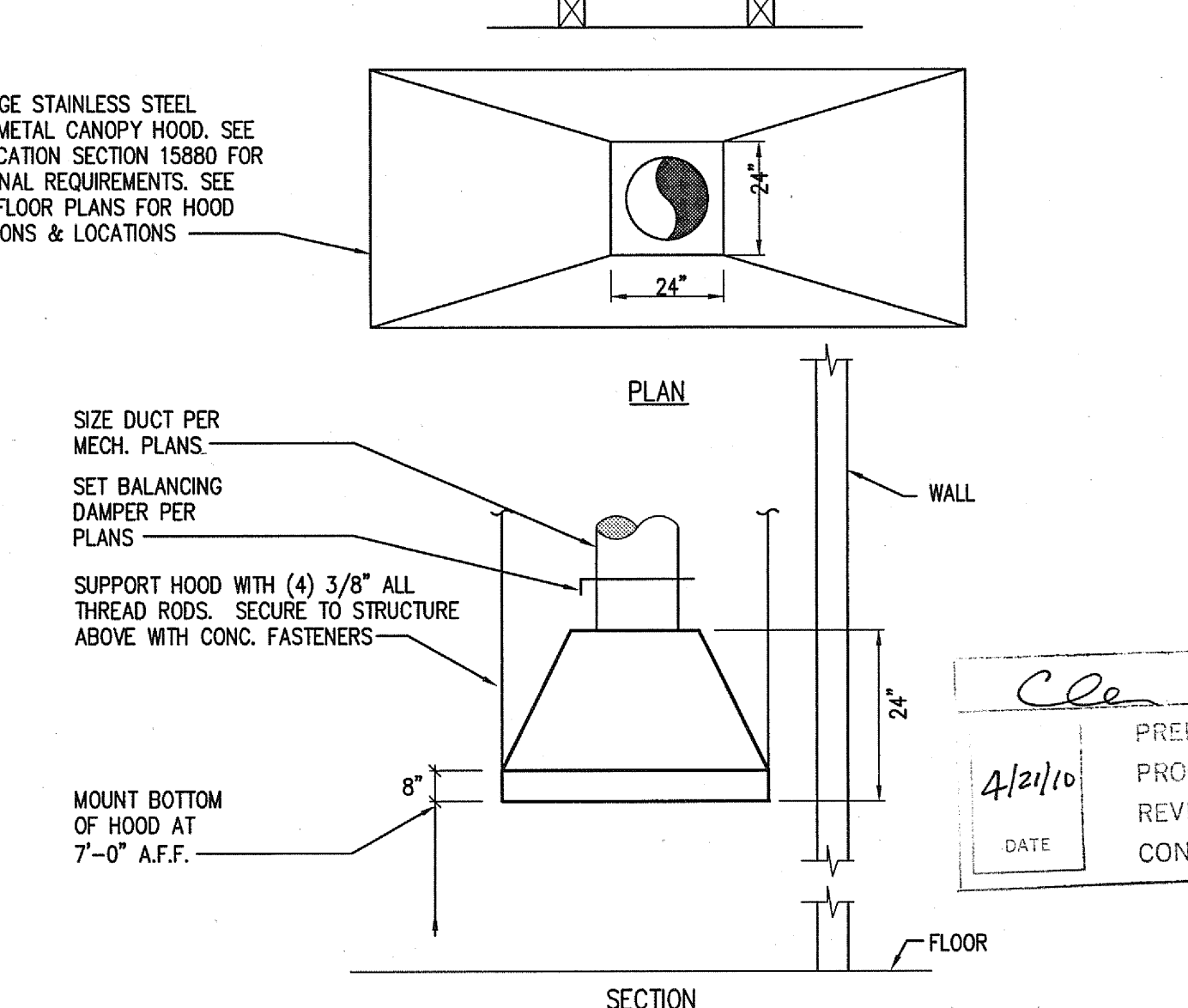
CANOPY HOOD
