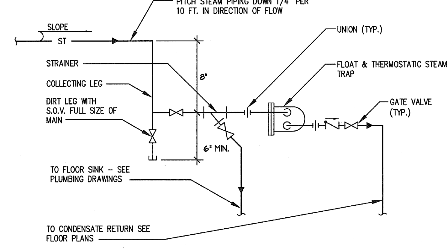
STEAM MAIN TRAP PIPING
