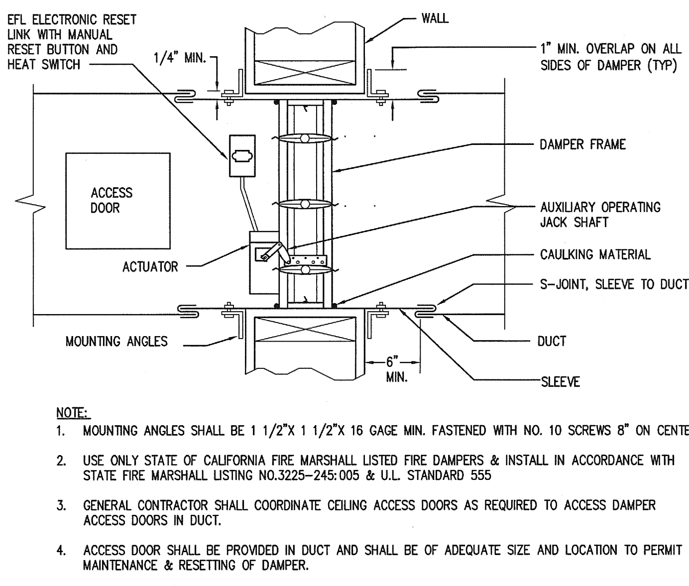
COMBINATION SMOKE / FIRE DAMPER
