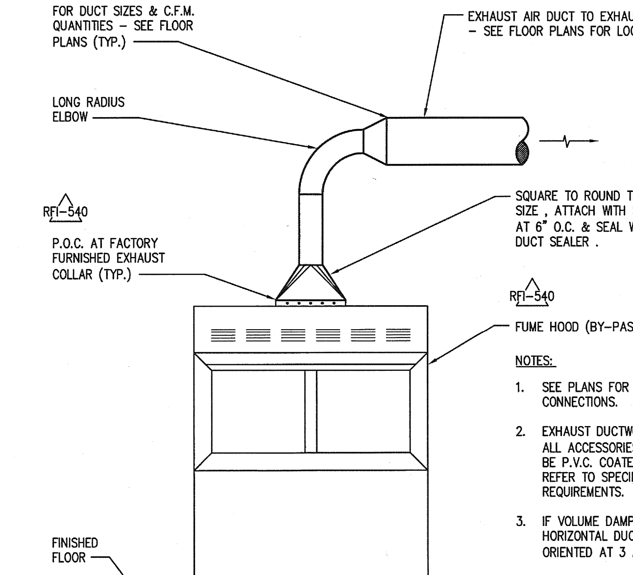
FUME HOOD CONNECTION (SINGLE)
