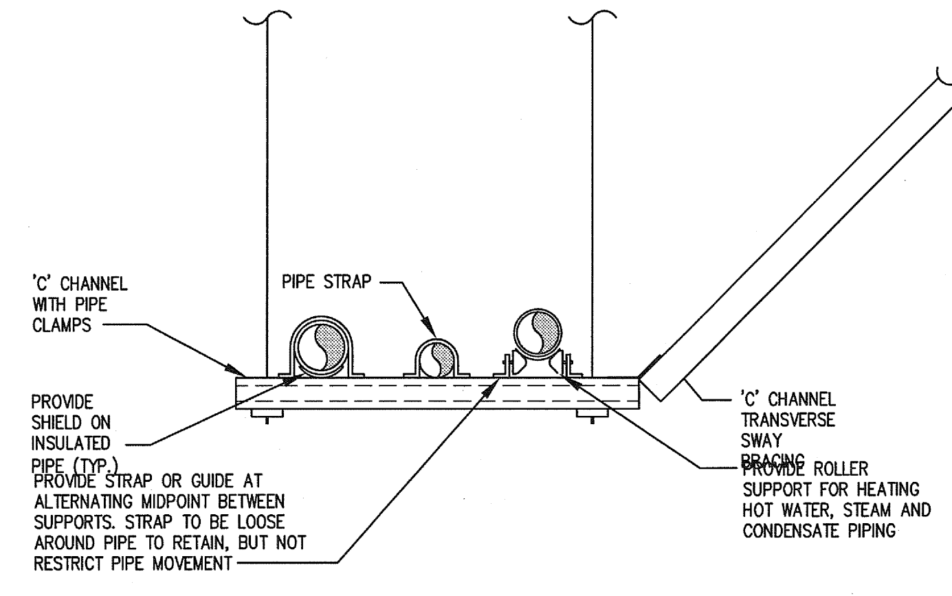
TRAPEZE PIPE SUPPORT
