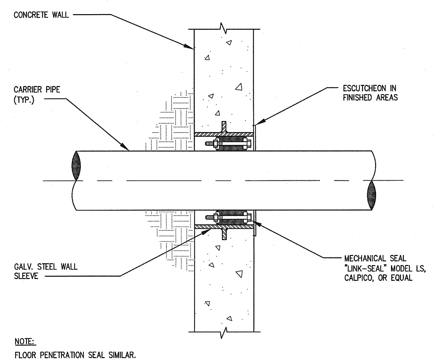
PIPE THRU CONCRETE EXTERIOR BELOW GRADE WALL
