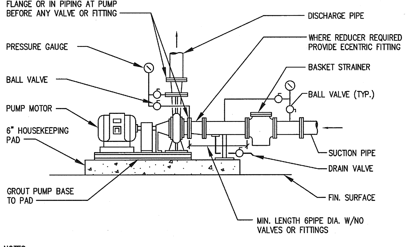
CONDENSER WATER PUMP DETAIL
