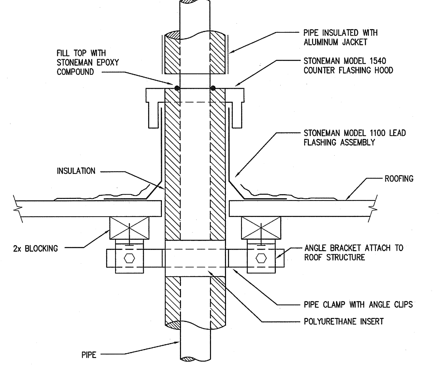
INSULATED PIPE THRU ROOF DETAIL
