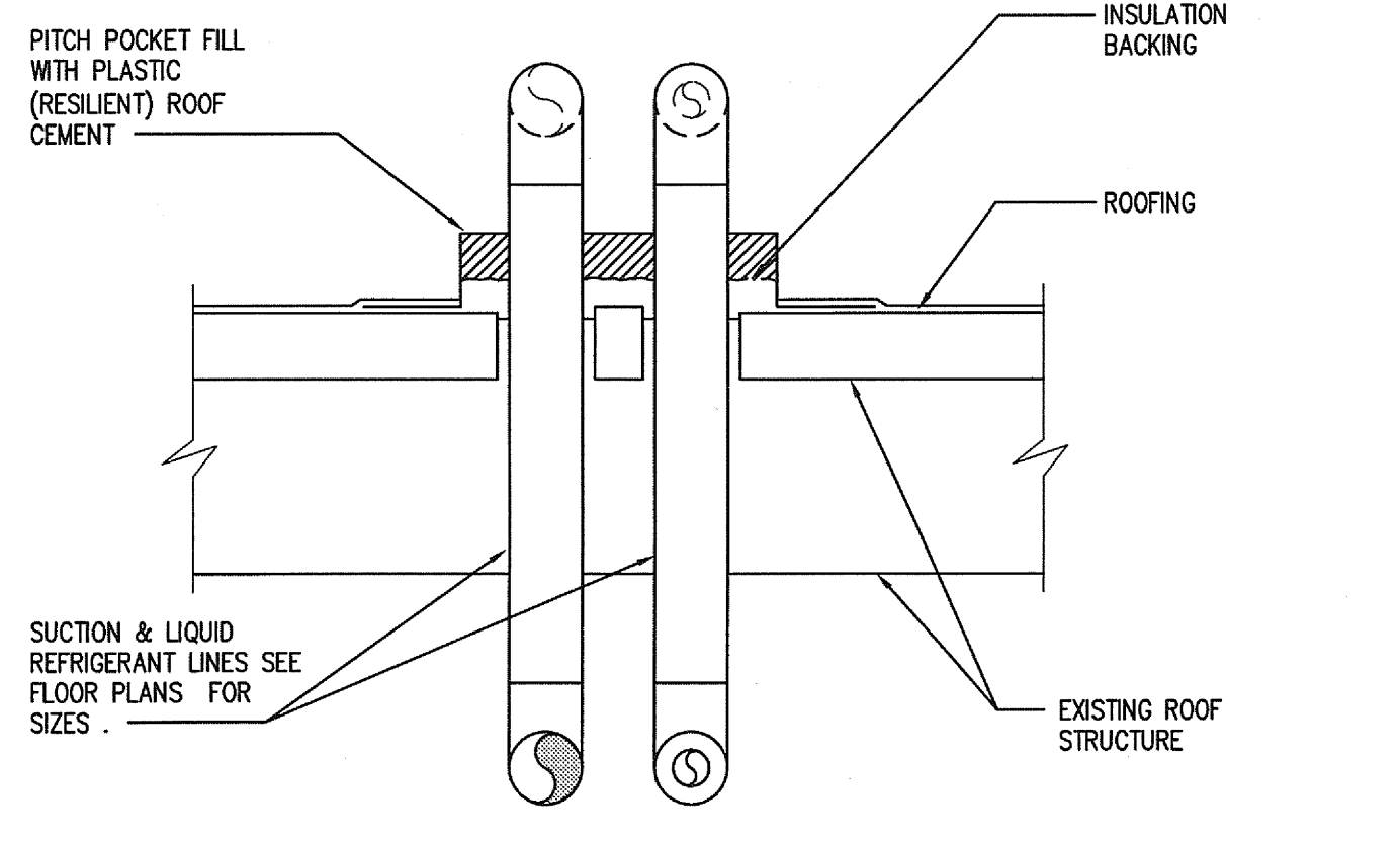
REFRIGERANT PIPING THRU ROOF
