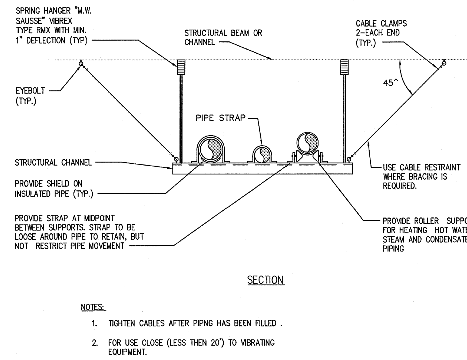
SUSPENDED PIPE SUPPORTS
