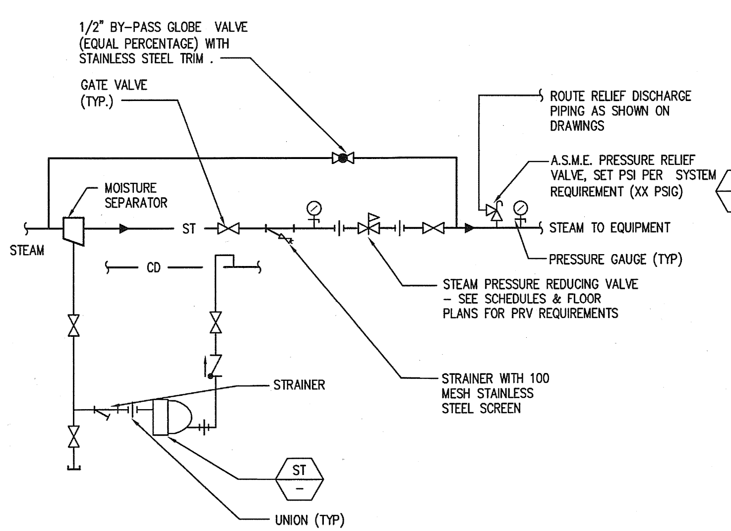
STEAM PRESSURE REDUCING STATION
