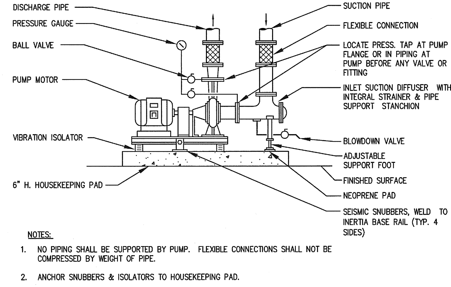
PUMP DETAIL
