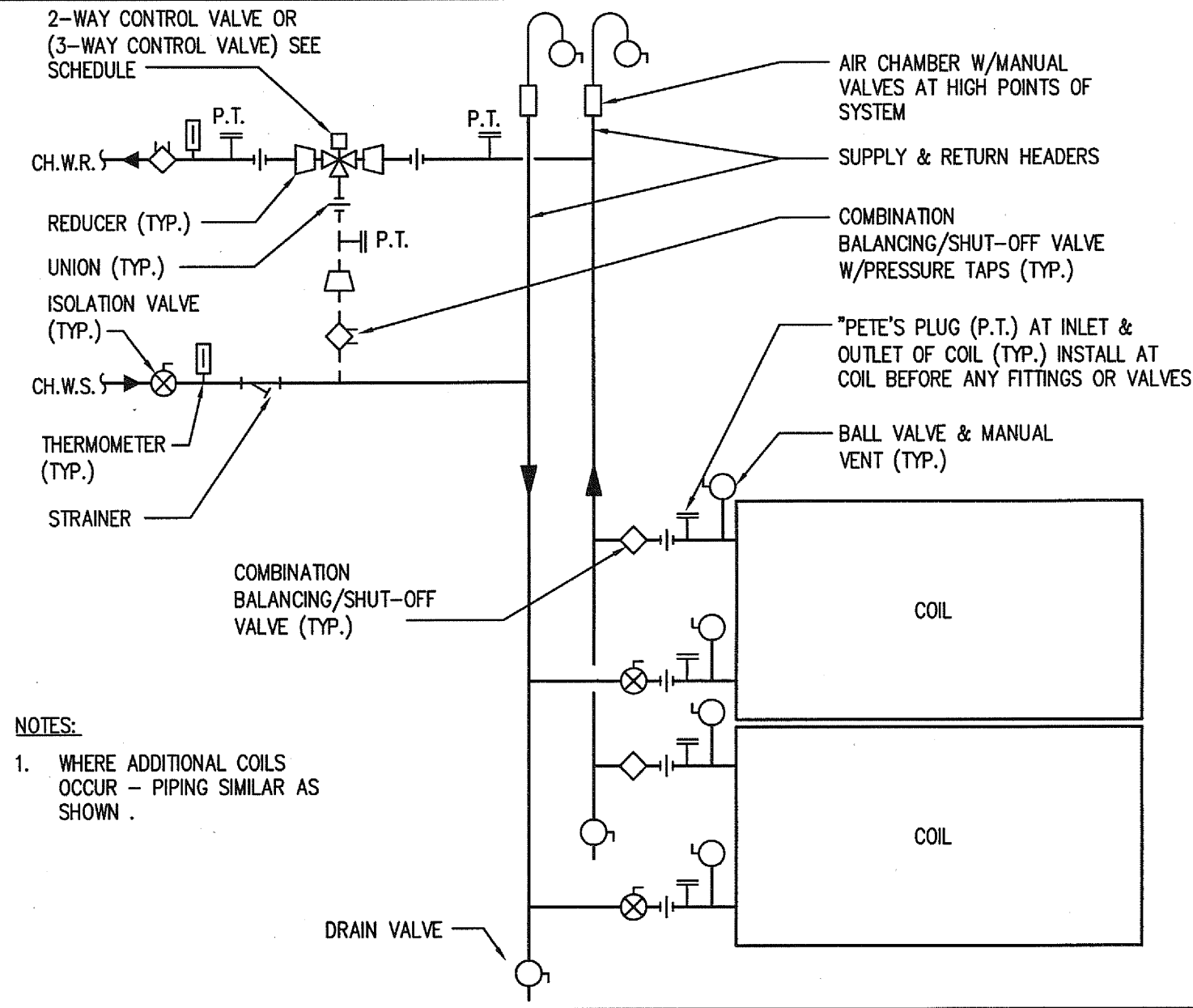
A.H. UNIT HEATING/COOLING COIL PIPING
