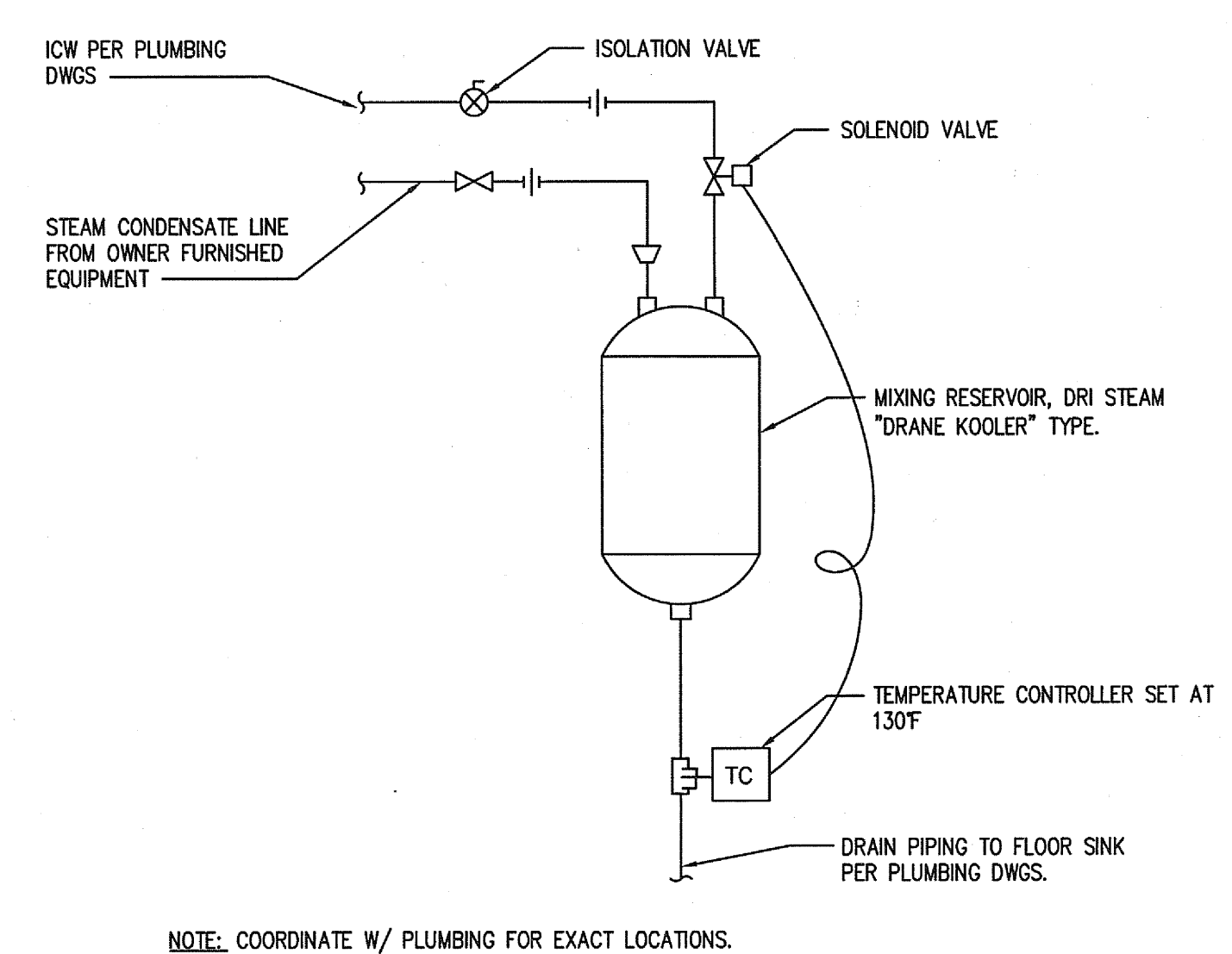
STEAM CONDENSATE COOLER DRAIN PIPING
