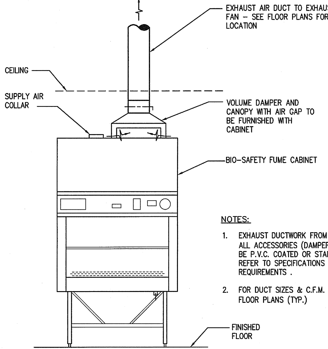
BIO-SAFETY FUME CABINET (WITH AIR GAP)
