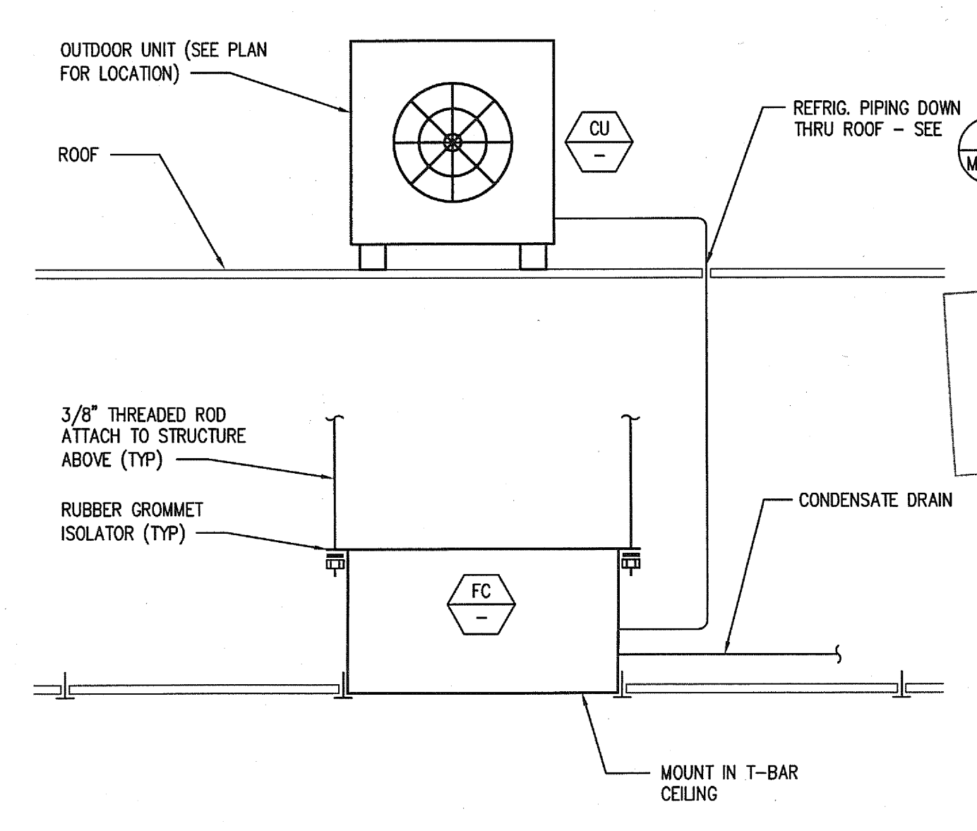
SPLIT SYSTEM A/C UNIT
