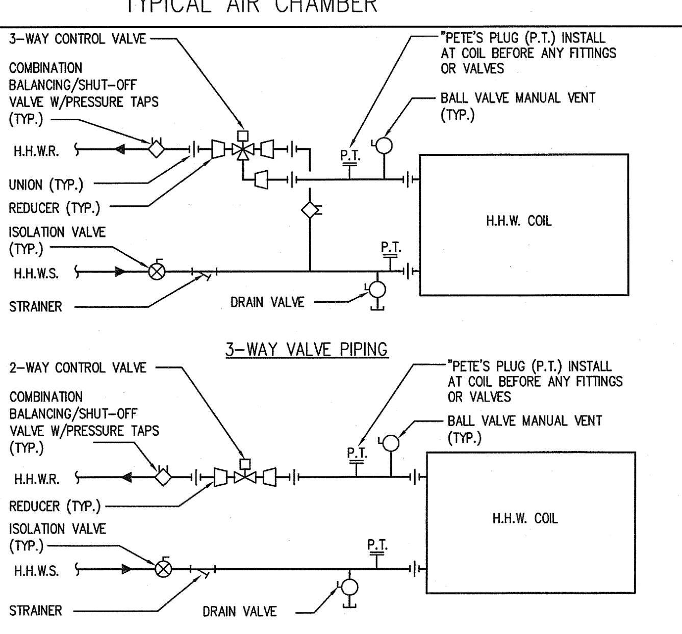
UNITARY HEATING/COOLING COIL PIPING
