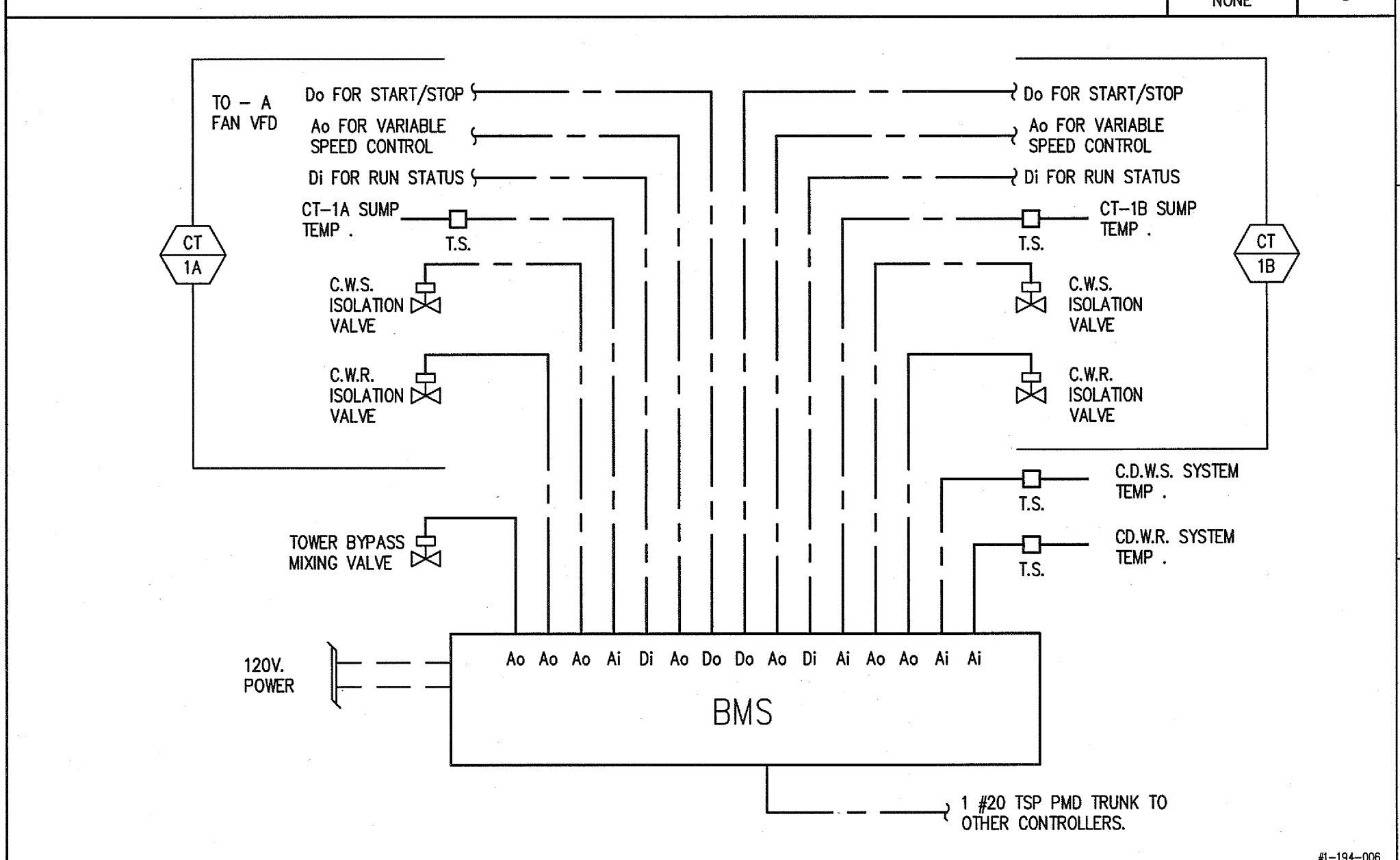
COOLING TOWER CONTROLS
