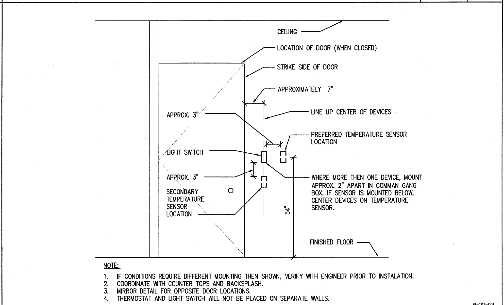
WALL DEVICE LOCATION
