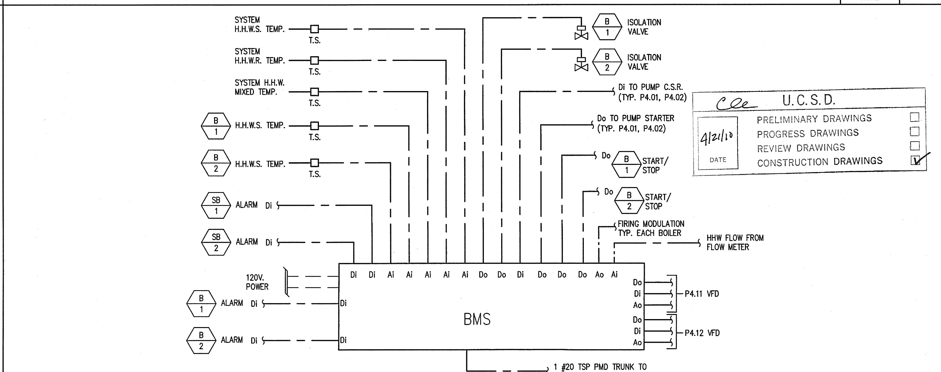
STEAM / HEATING HOT WATER CONTROLS
