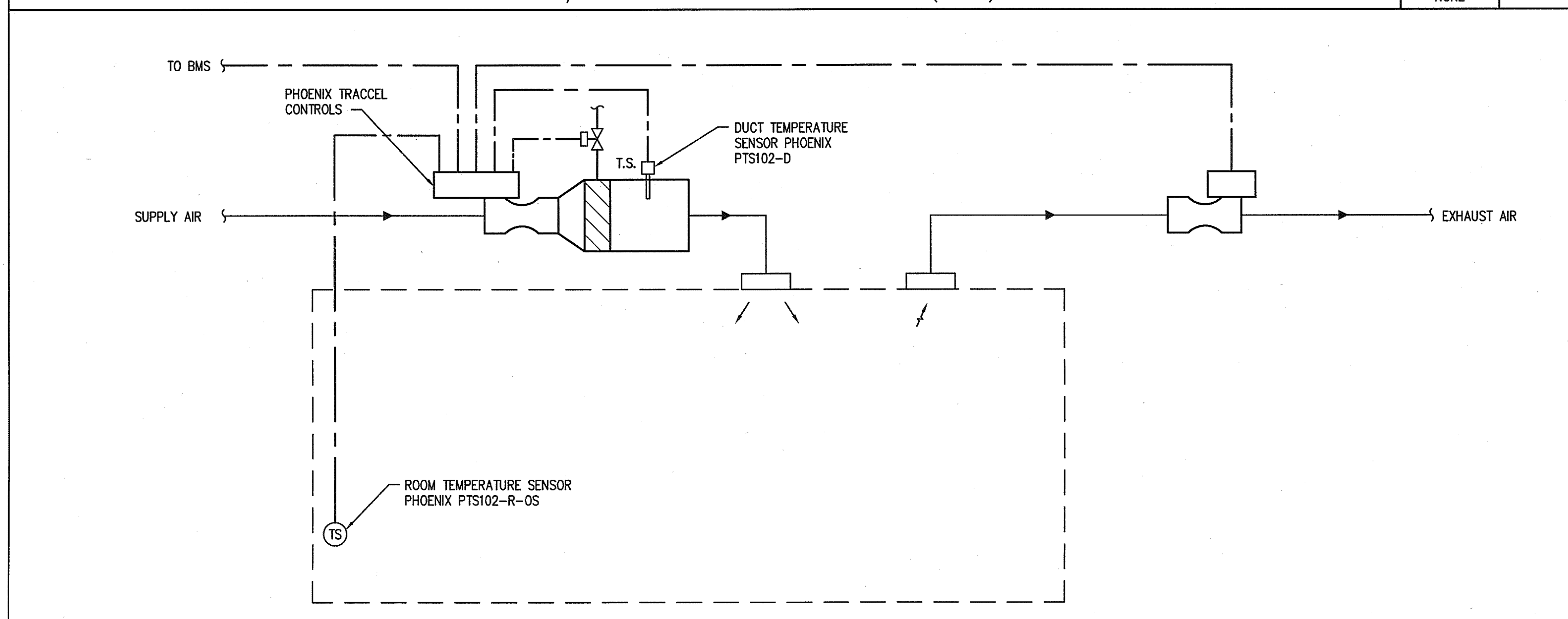
TYPICAL LAB SUPPORT ROOM CONTROL
