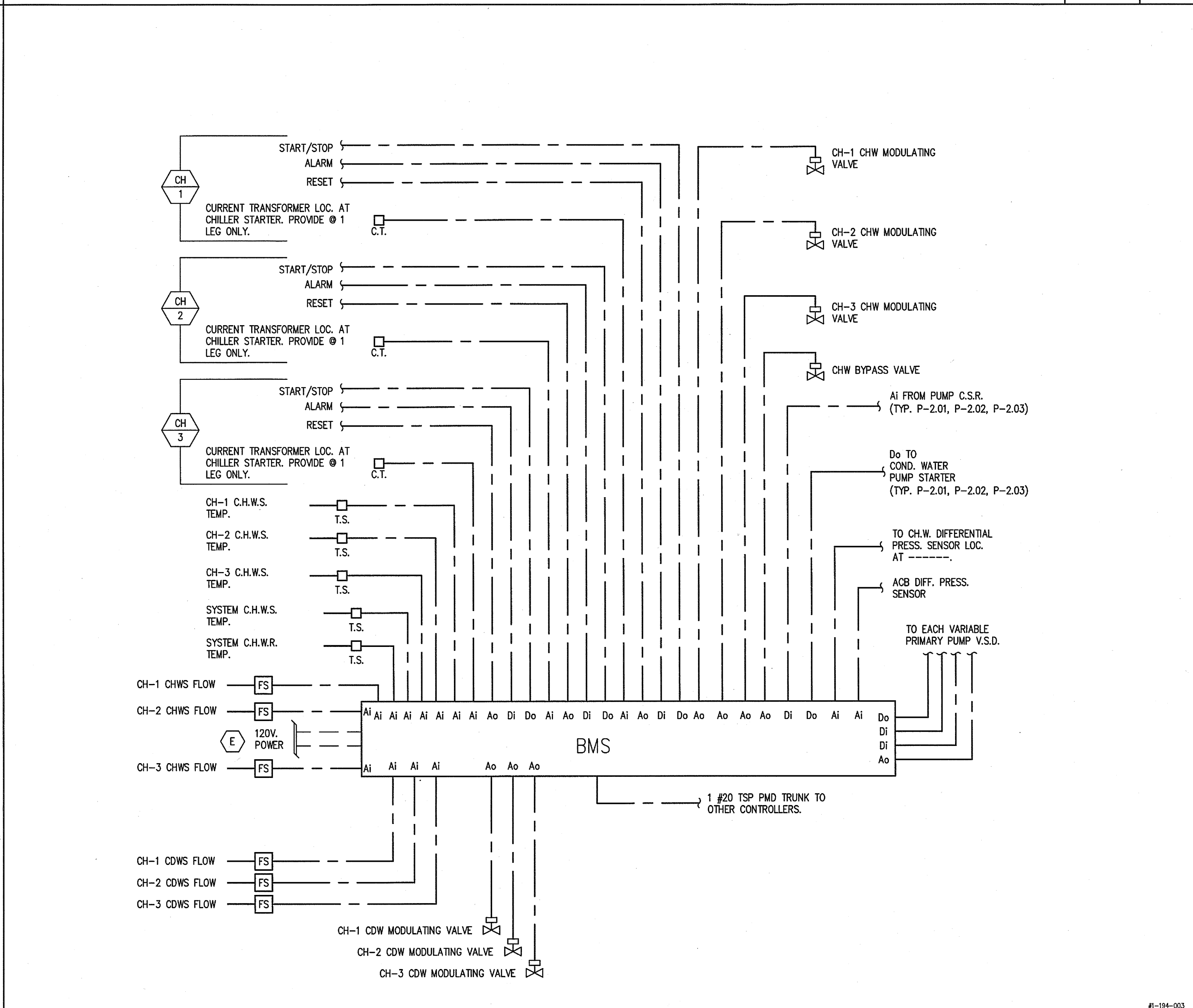
VARIABLE PRIMARY CHW SYSTEM CONTROL
