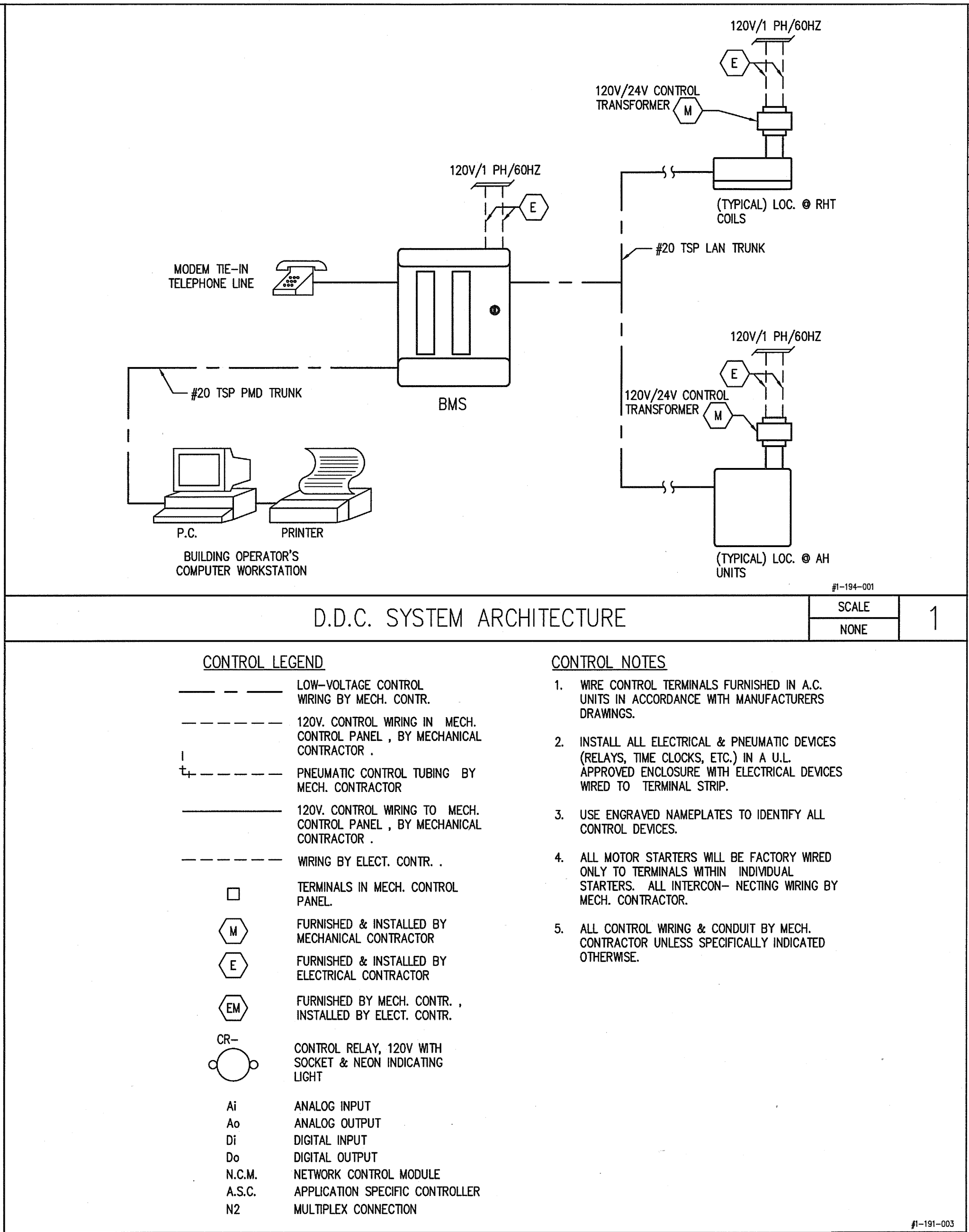
D.D.C. SYSTEM ARCHITECTURE
