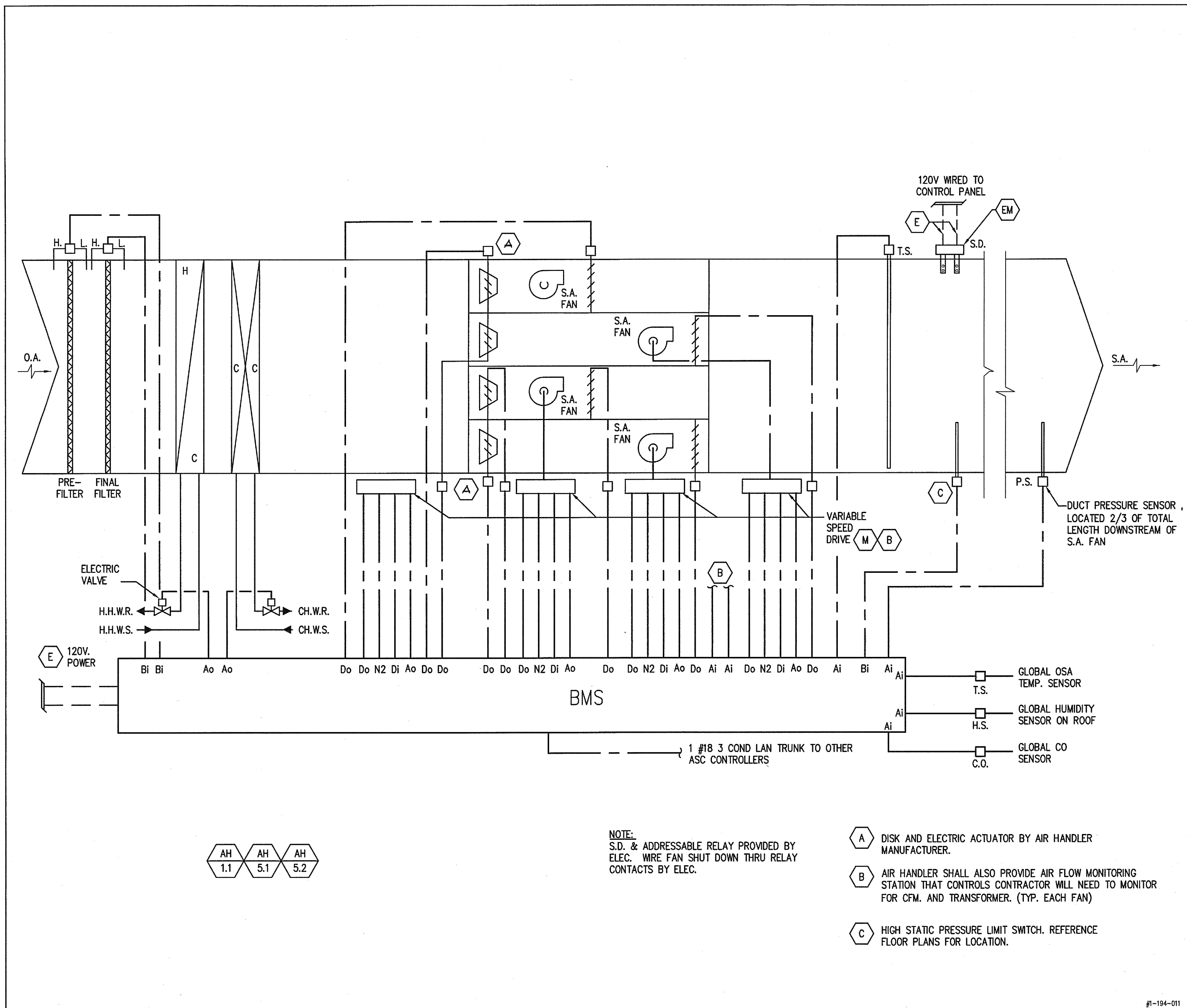
LABORATORY AND VIVARIUM AIR HANDLER CONTROL W/ V.F.D.
