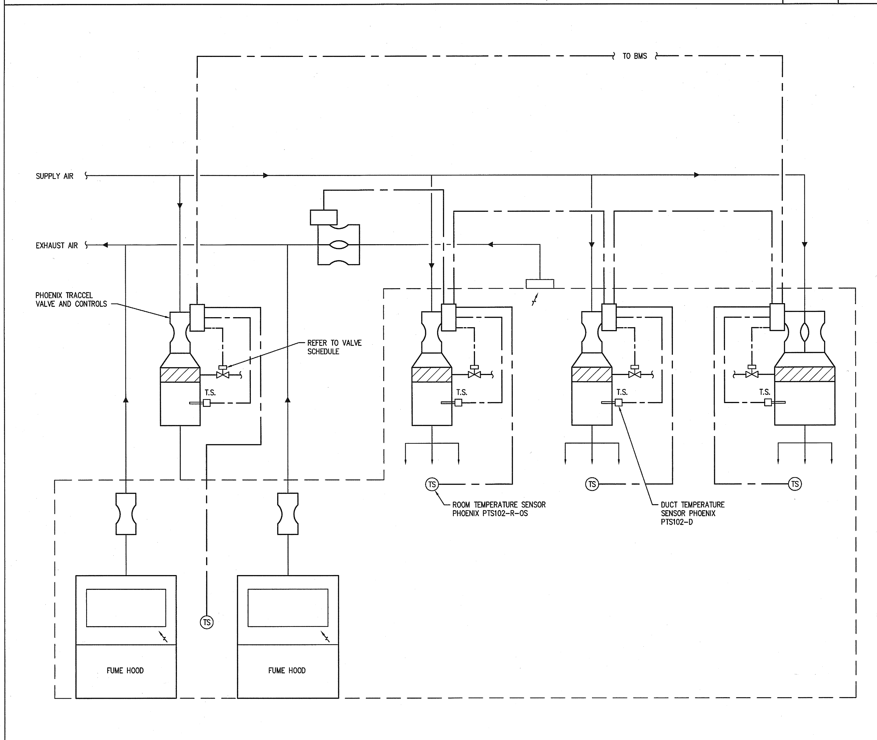
TYPICAL LAB/FUME HOOD ROOM CONTROLS (TYP.)
