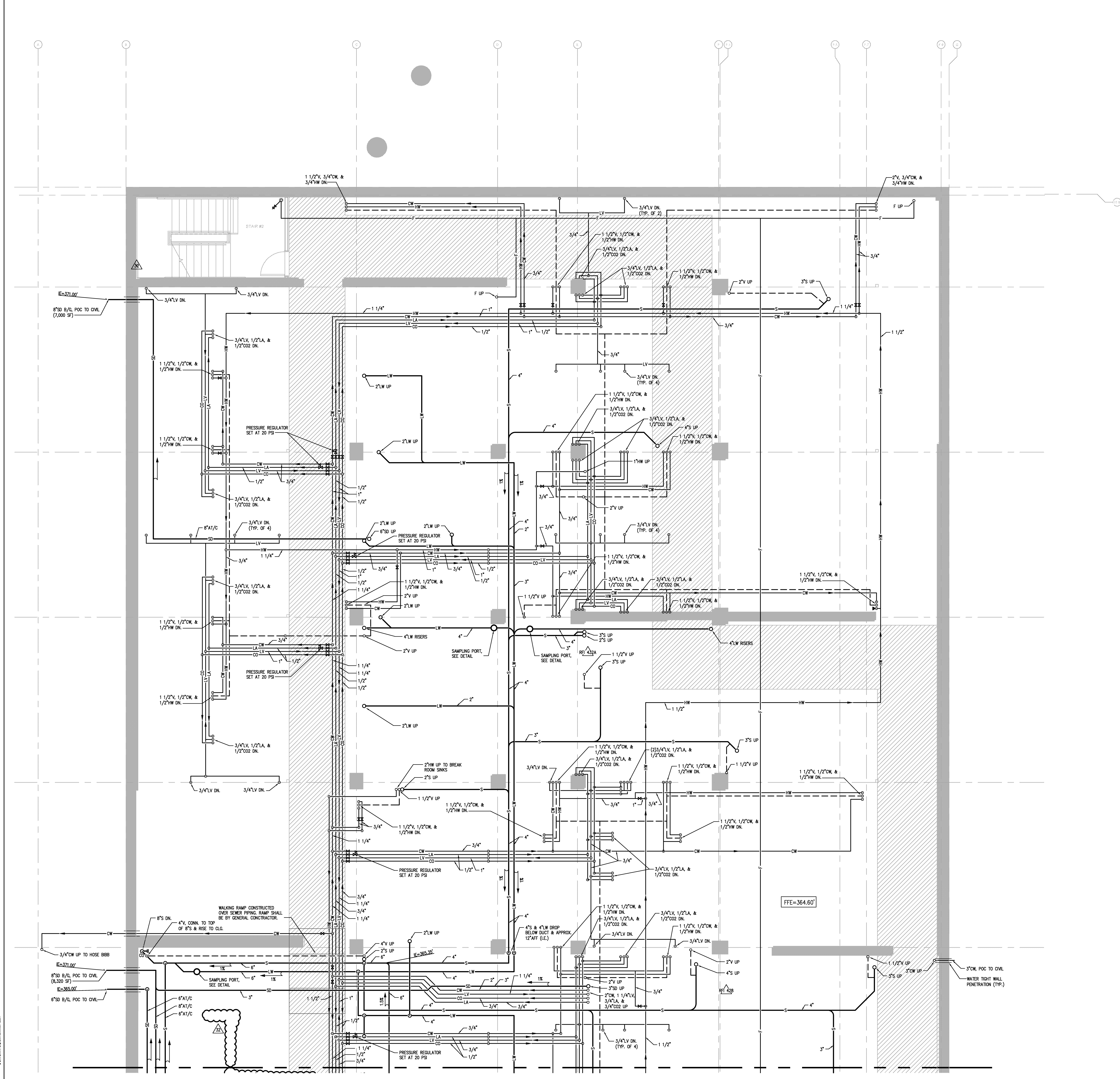
PARTIAL PLUMBING INTERSTITIAL PLAN - ZONE 1
