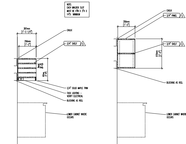
TYP UPPER SHELF, SMALL 3 1" = 1'-0"
