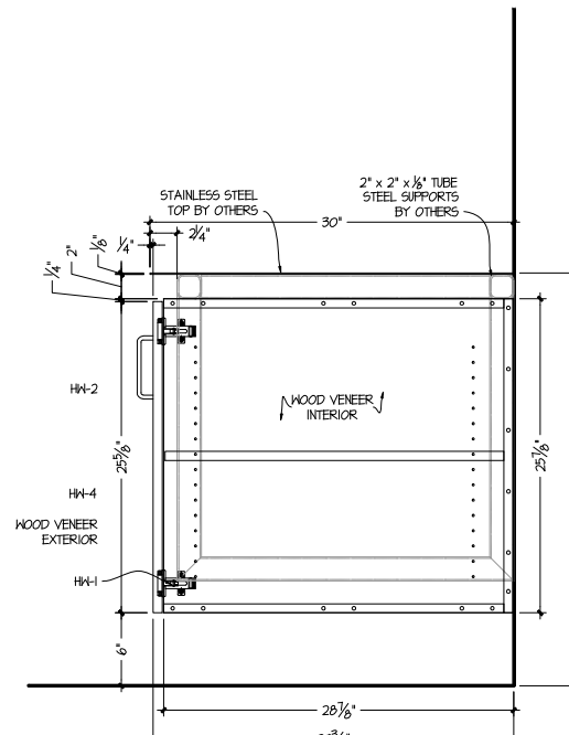
F MILLWORK SECTION SCALE: 1 1/2" = 12"
