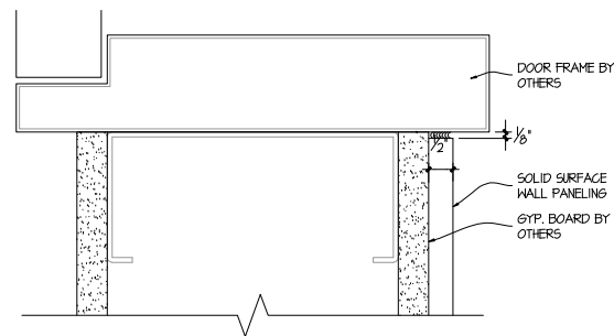
K WALL PANELING DETAIL SECTION 6" = 12"
