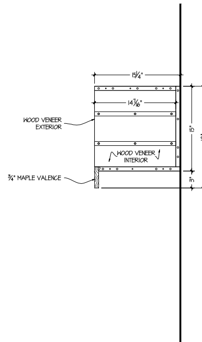
E MILLWORK SECTION SCALE: 1 1/2" = 12"
