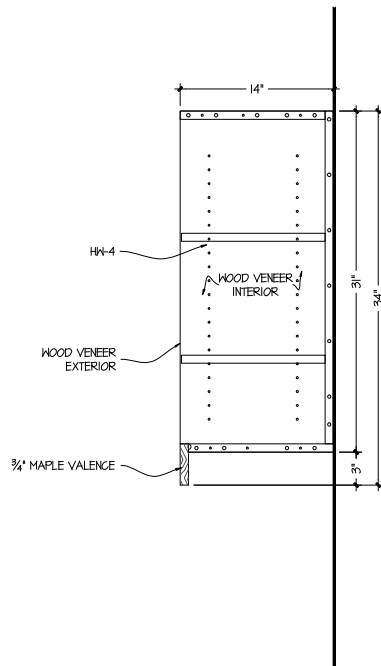
D MILLWORK SECTION SCALE: 1 1/2" = 12"
