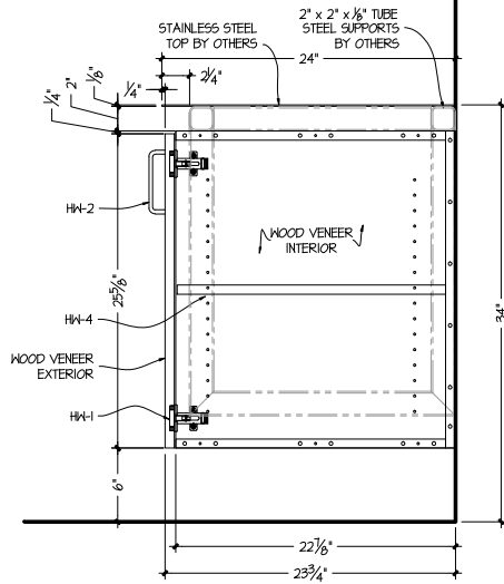
A MILLWORK SECTION SCALE: 1 1/2" = 12"
