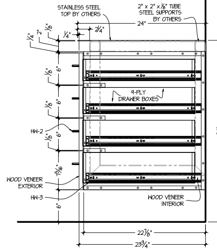
B MILLWORK SECTION SCALE: 1 1/2" = 12"
