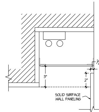
N WALL PNING LIGHT COVE DTL SECTION 3" = 12" ARCH. REF.: 12 / Z_A5550
