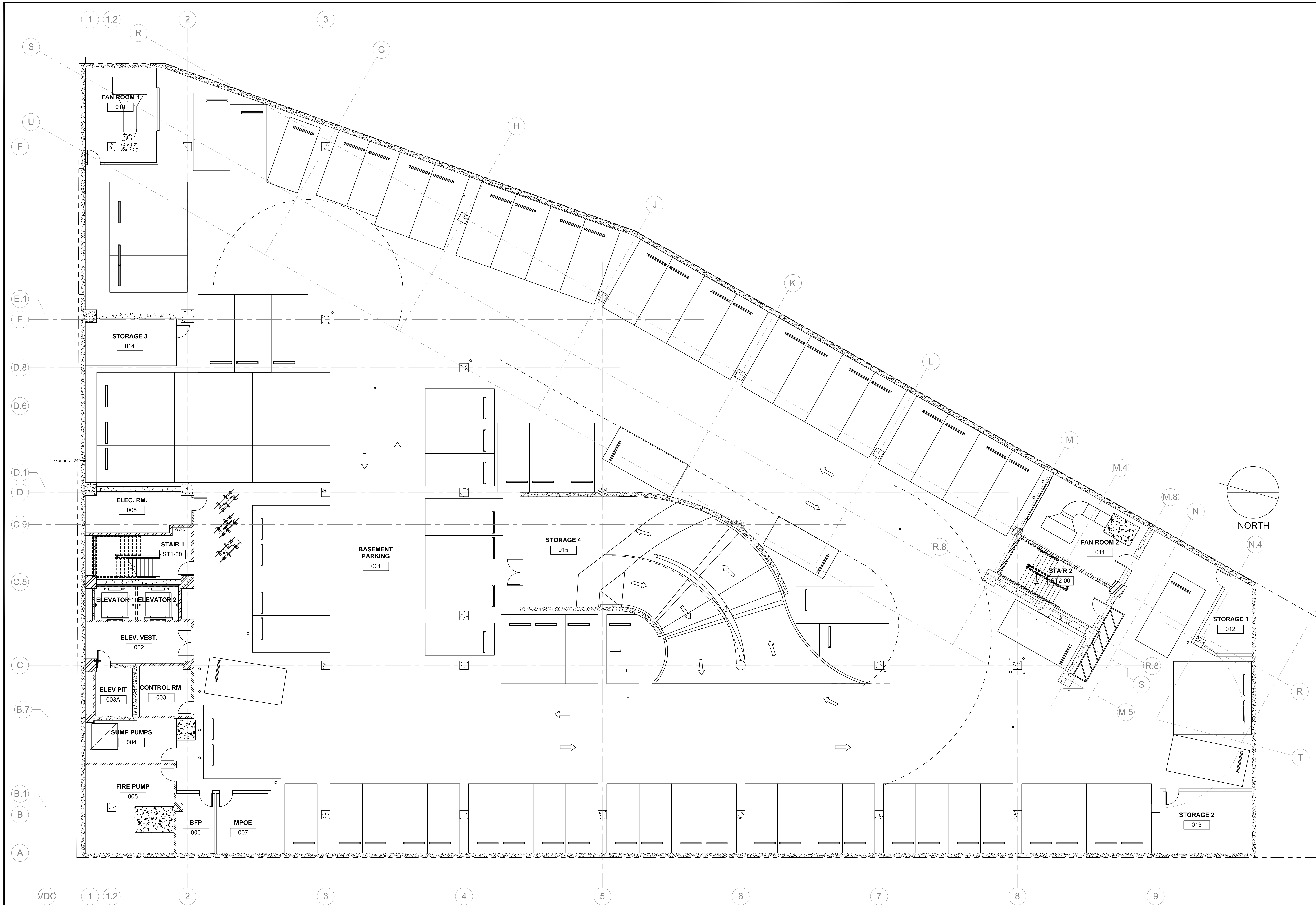
1 BASEMENT FLOOR PLAN SCALE 1/8" = 1'-0"
